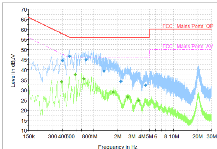
Fig. 96 AC Power line Conducted Emission (Idle, AE4, 120V)
