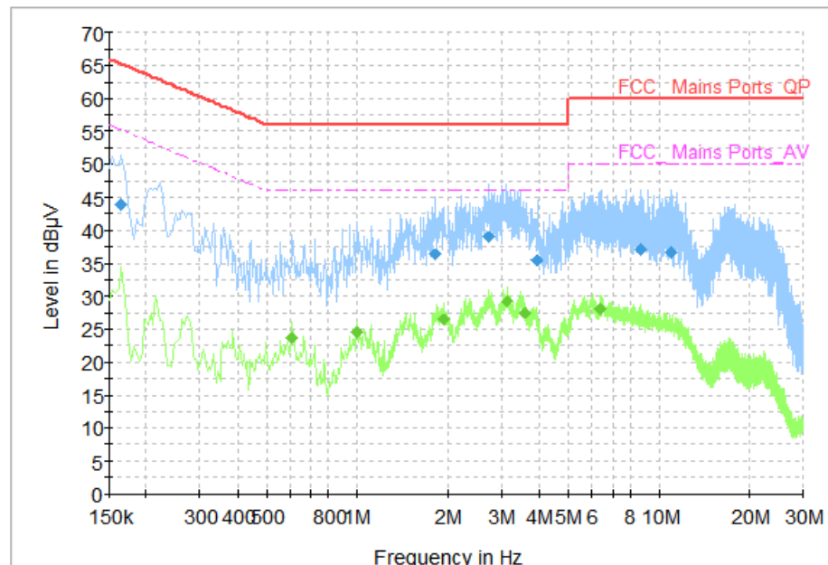
Fig. 97 AC Powerline Conducted Emission (Traffic, AE3, 240V)
