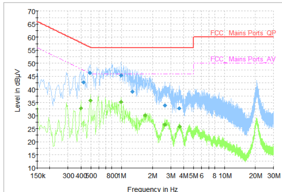
Fig. 95 AC Powerline Conducted Emission (Traffic, AE4, 120V)
