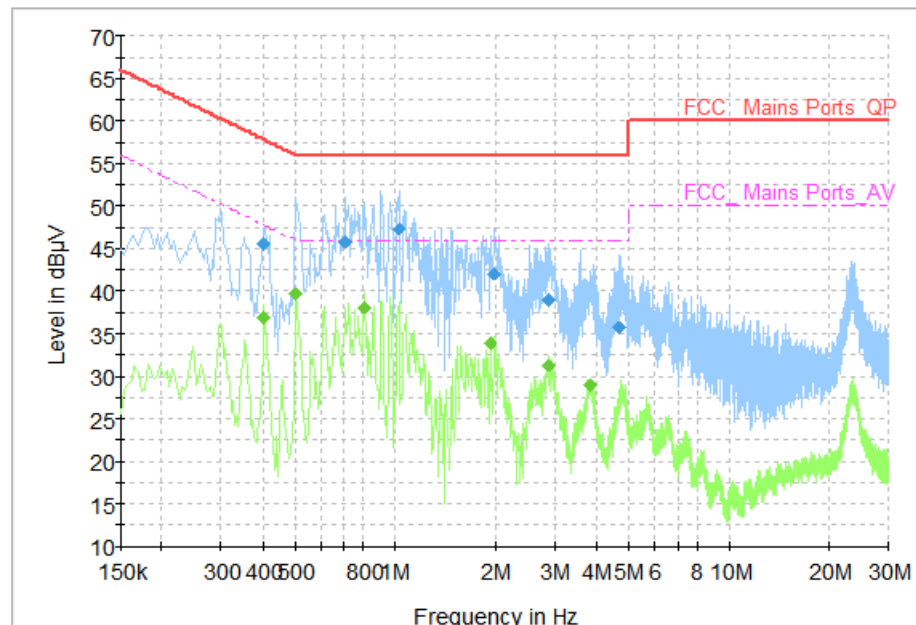
Fig. 99 AC Powerline Conducted Emission (Traffic, AE4, 240V)
