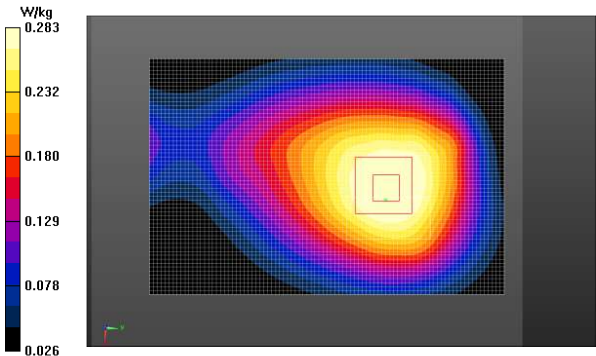
Fig.10 LTE Band 71
