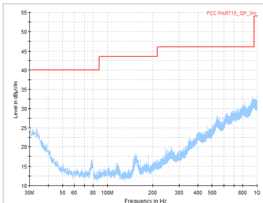
Fig.66 Radiated Spurious Emission (All Channels, 30MHz-1 GHz)
