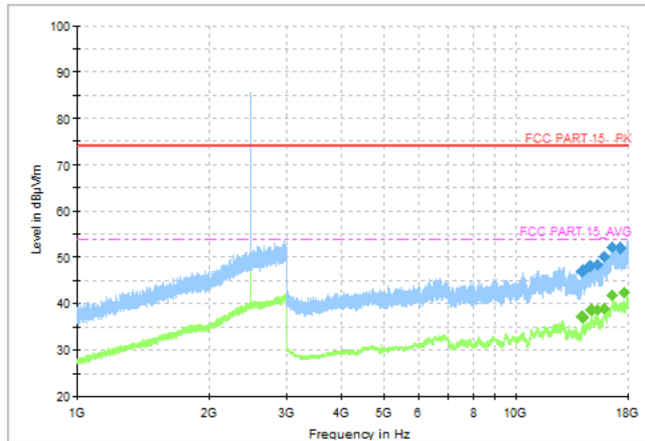
Fig.25 Radiated Spurious Emission (GFSK, Ch39, 1 GHz ~18 GHz)
