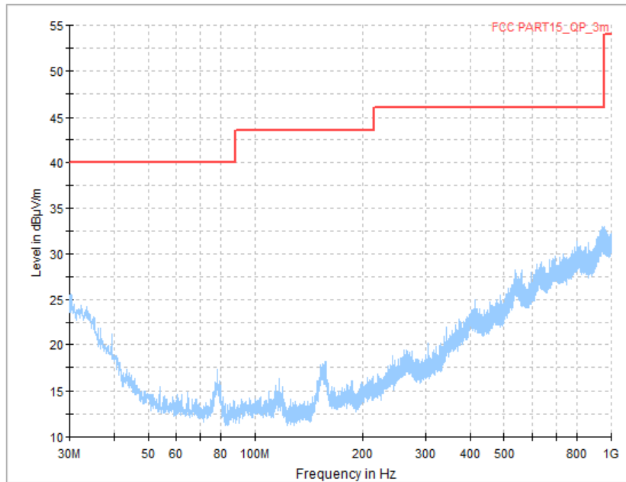
Fig.29 Radiated Spurious Emission (All Channels, 30 MHz-1 GHz)
