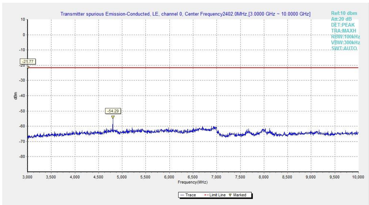
Fig.14 Conducted Spurious Emission (Ch0, 3 GHz-10 GHz)
