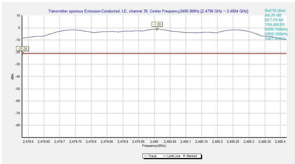
Fig.18 Conducted Spurious Emission (Ch39, Center Frequency)
