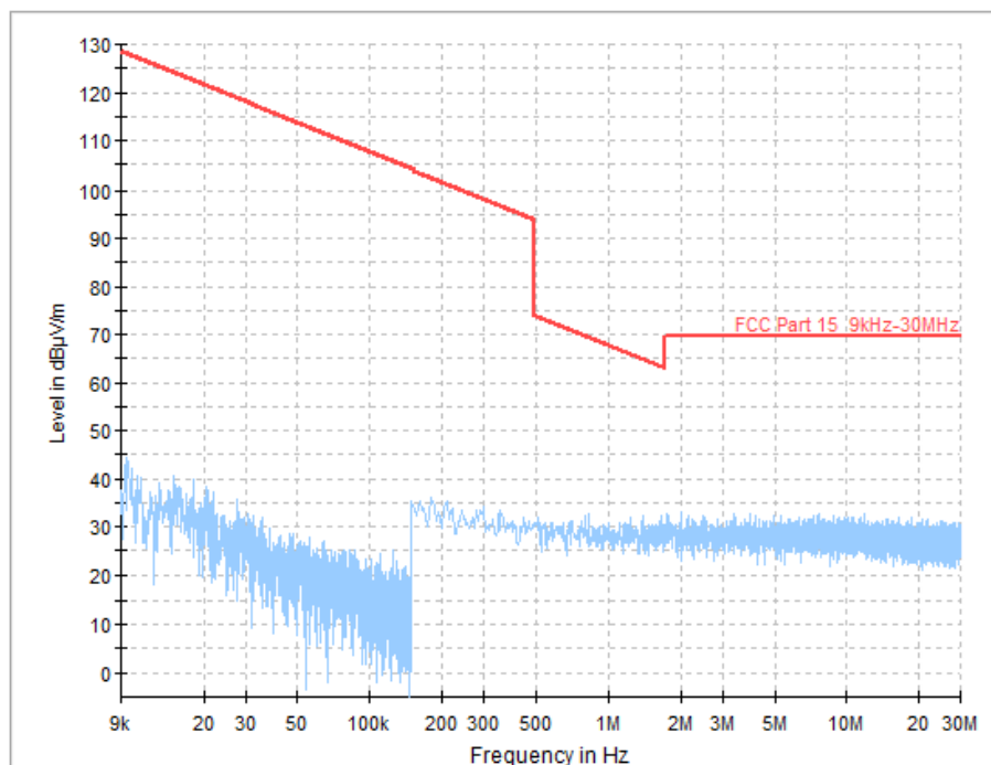
Fig.28 Radiated Spurious Emission (All Channels, 9 kHz-30 MHz)
