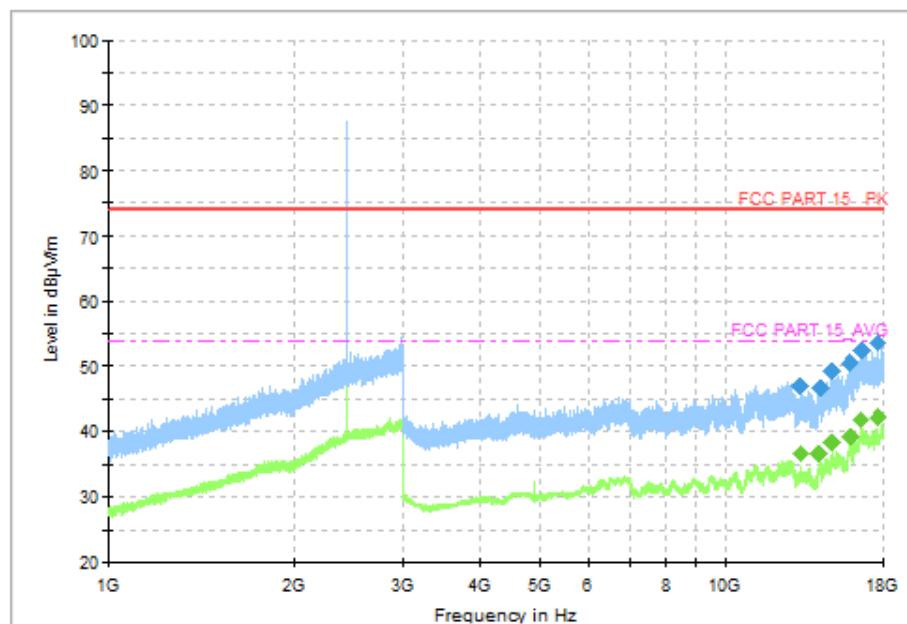
Fig.24 Radiated Spurious Emission (GFSK, Ch19, 1 GHz ~18 GHz)
