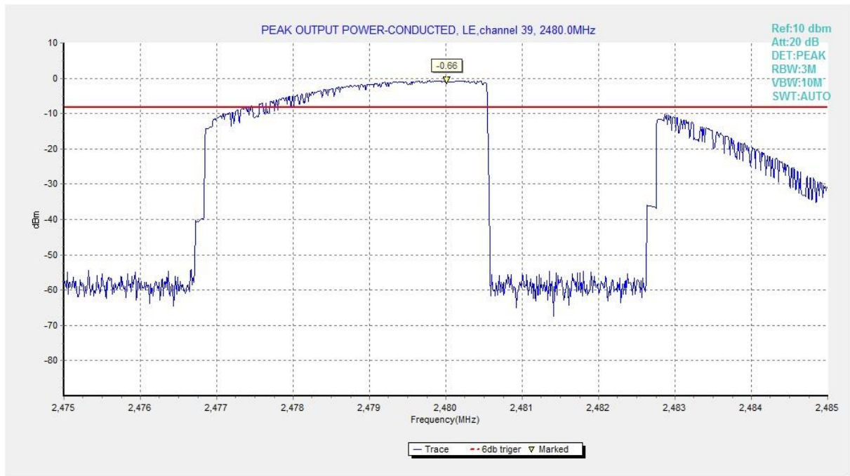
Fig.3 RF output power (Ch 39)
