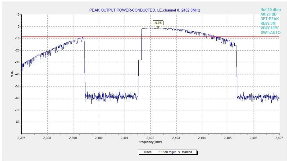
Fig.1 RF output power (Ch 0)
