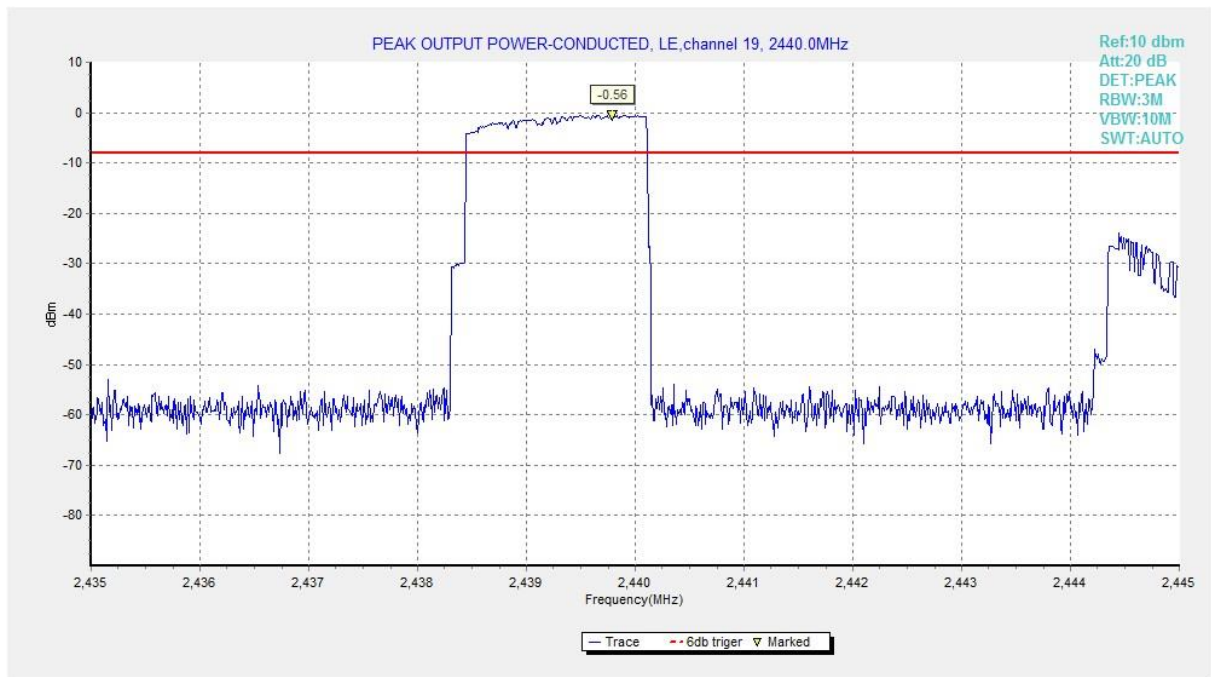
Fig.2 RF output power (Ch 19)
