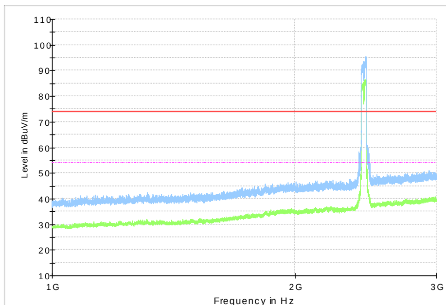
Fig.71 Radiated Spurious Emission (802.11n HT40, CH6, 1GHz-3GHz)
