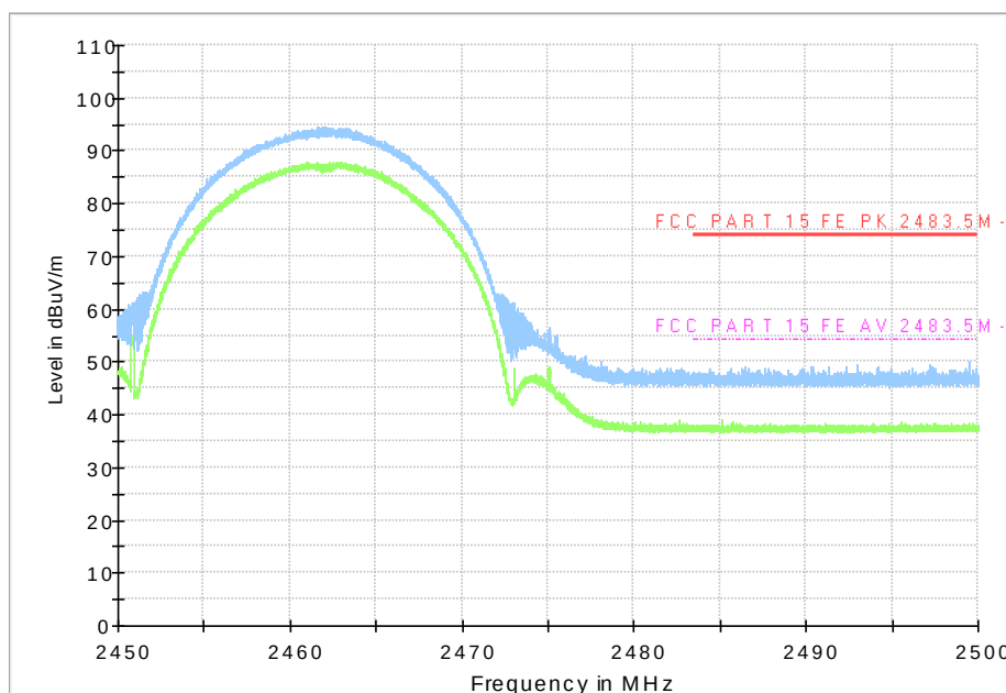
Fig.52 Radiated Restricted Band (802.11b, CH11, 2.45GHz~2.5GHz)
