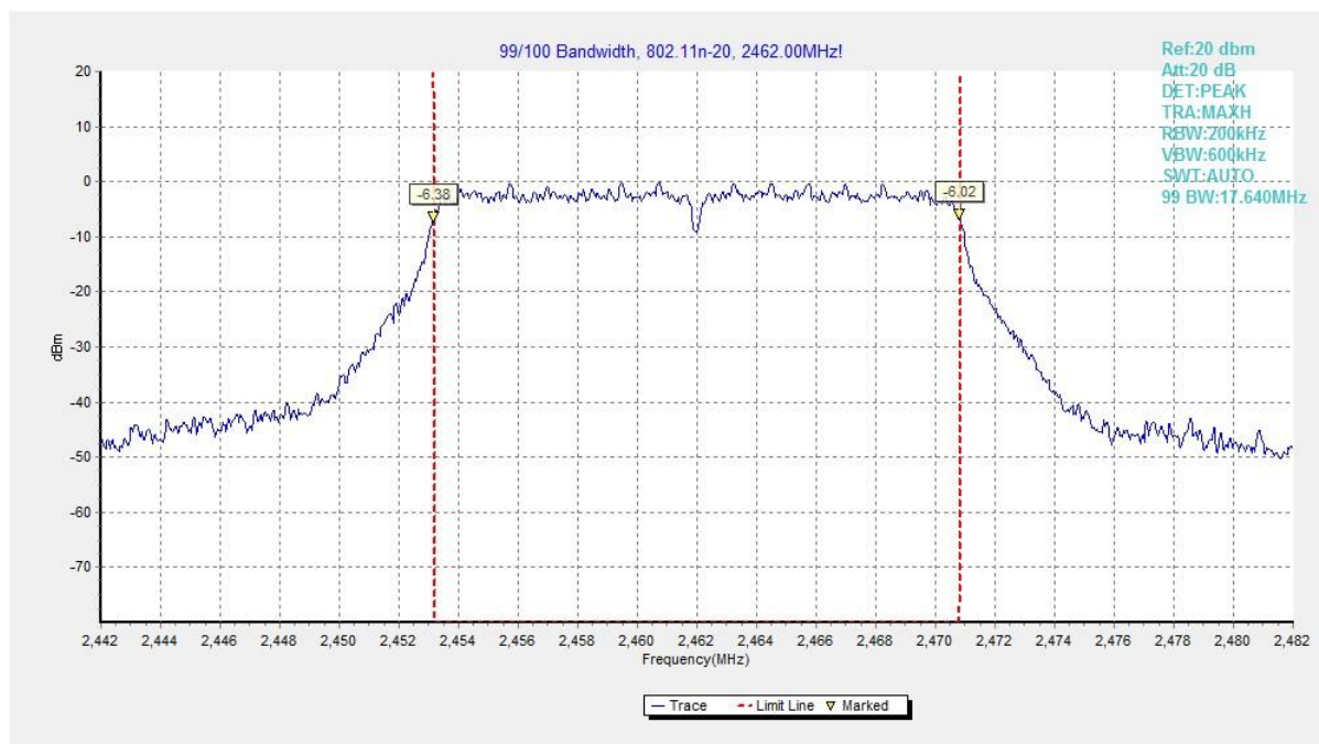
Fig.96 Occupied Bandwidth (802.11n HT20, CH11)
