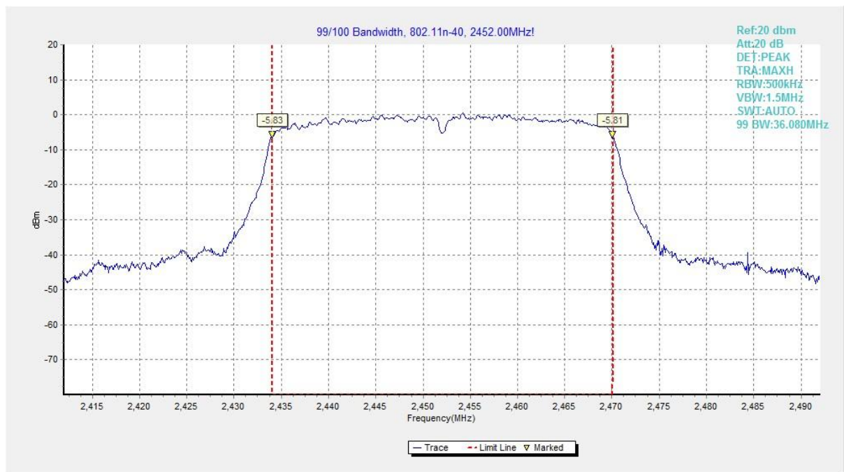
Fig.99 Occupied Bandwidth (802.11n HT40, CH9)
