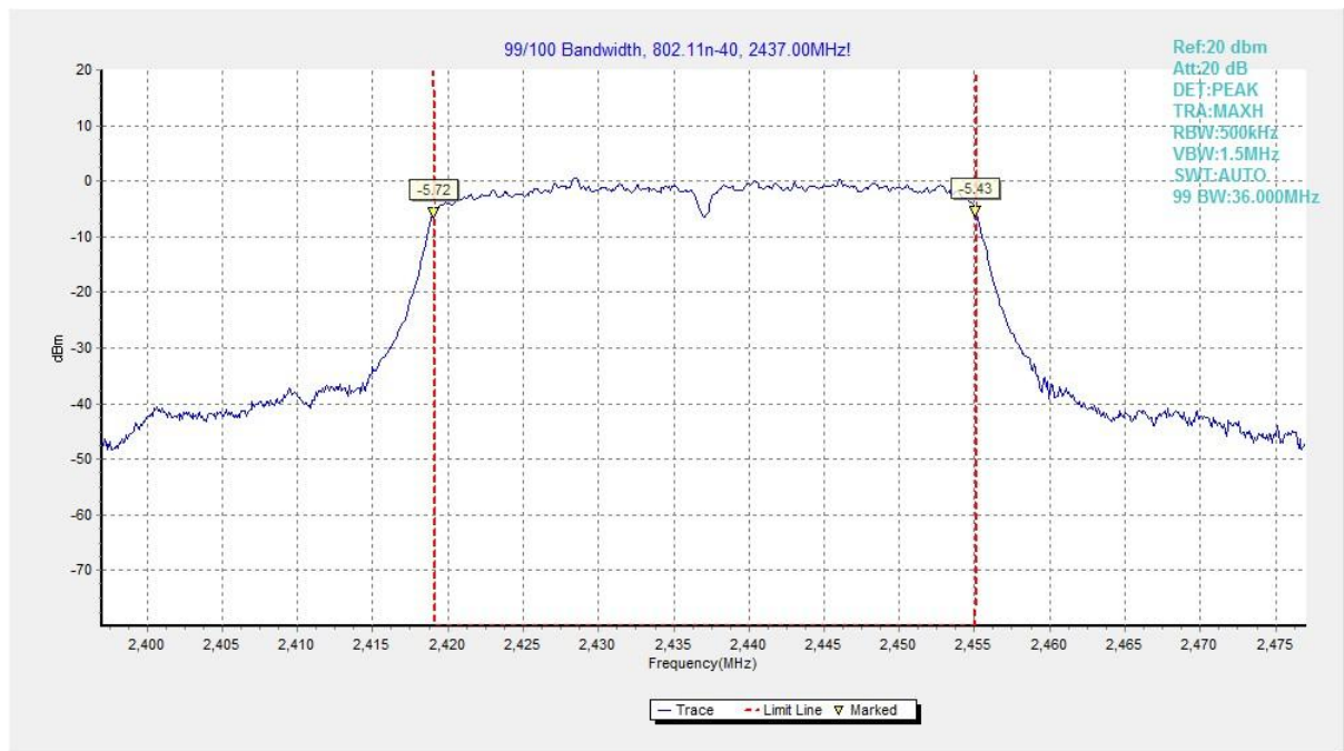
Fig.98 Occupied Bandwidth (802.11n HT40, CH6)
