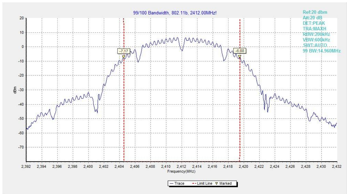
Fig.88 Occupied Bandwidth (802.11b, CH1)
