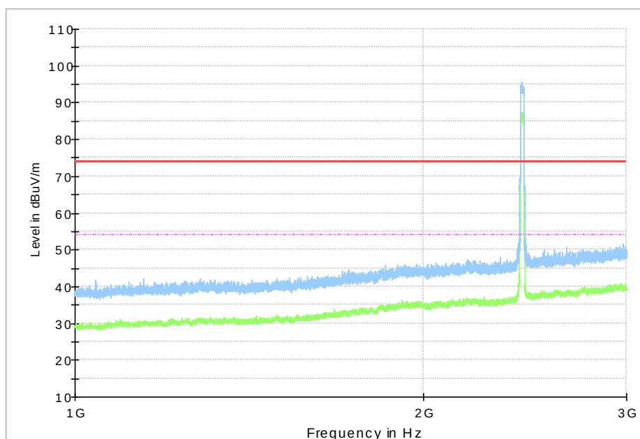
Fig.63 Radiated Spurious Emission (802.11n HT20, CH6, 1GHz-3GHz)
