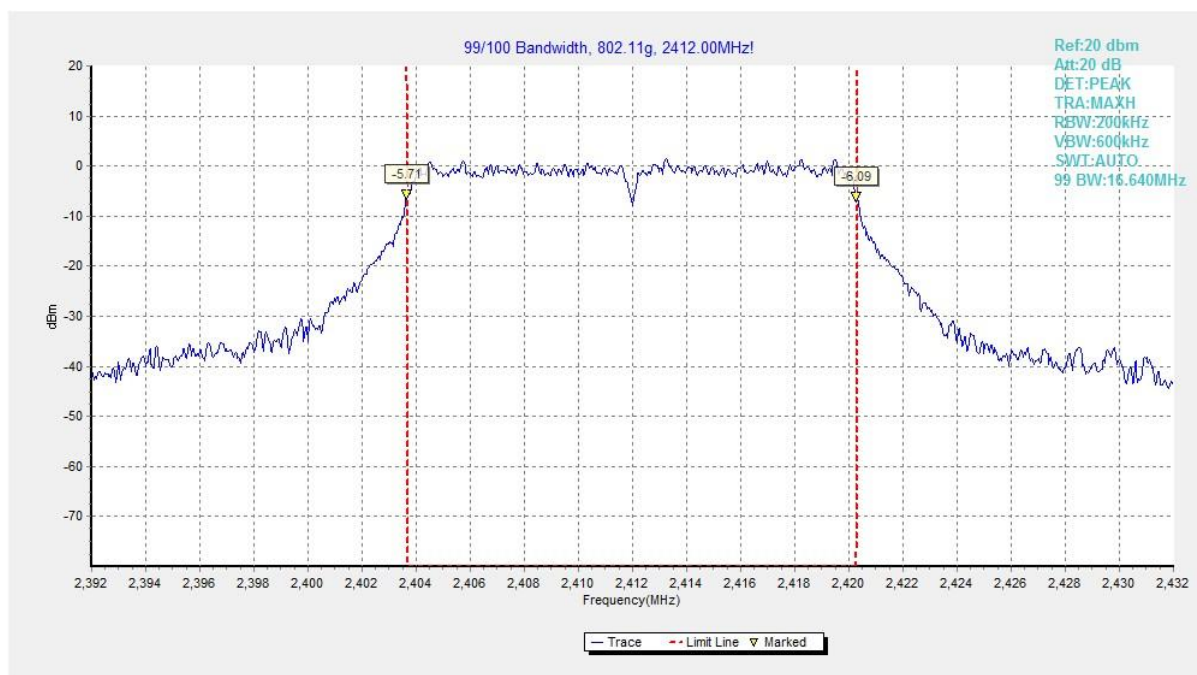
Fig.91 Occupied Bandwidth (802.11g, CH1)
