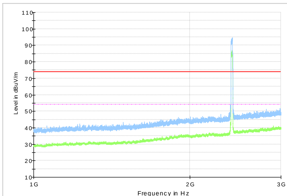
Fig.61 Radiated Spurious Emission (802.11n HT20, CH1, 1GHz-3GHz)
