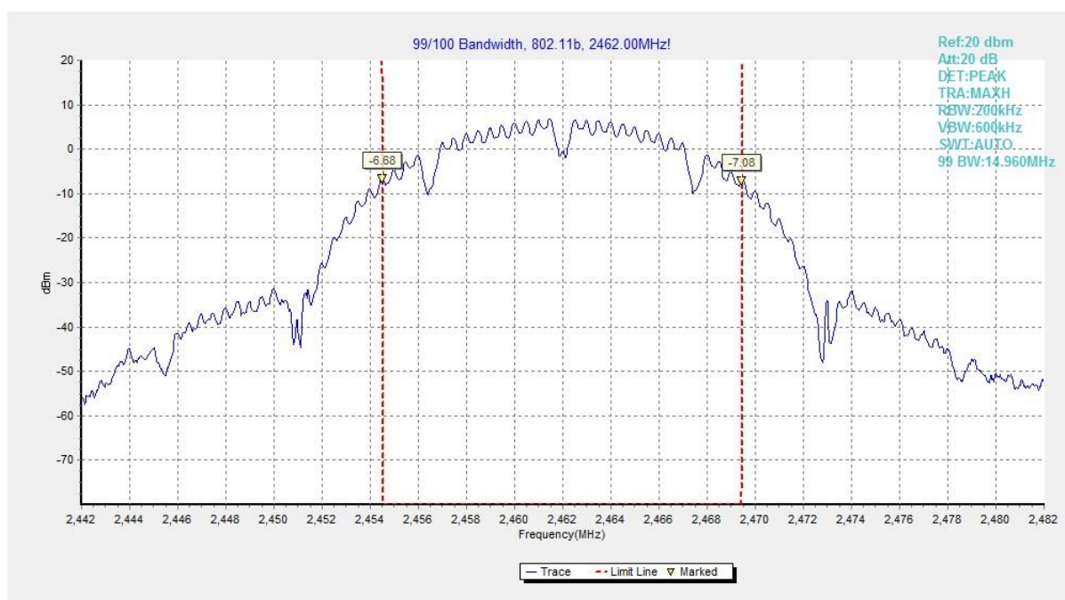
Fig.90 Occupied Bandwidth (802.11b, CH11)
