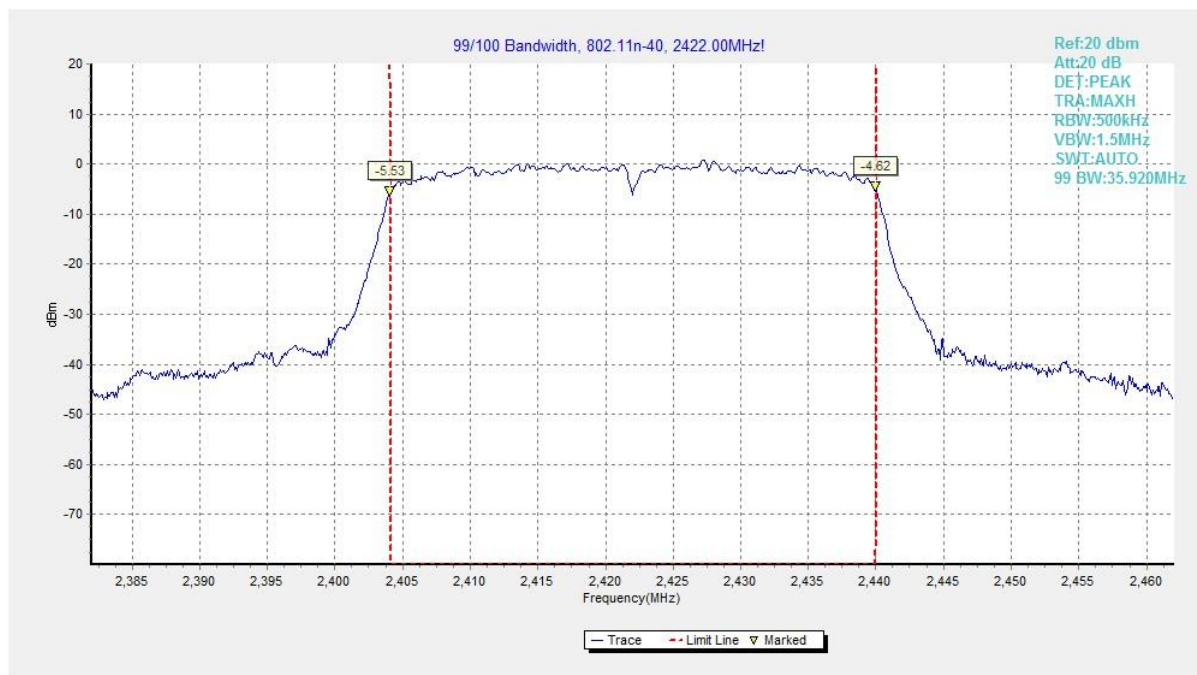
Fig.97 Occupied Bandwidth (802.11n HT40, CH3)
