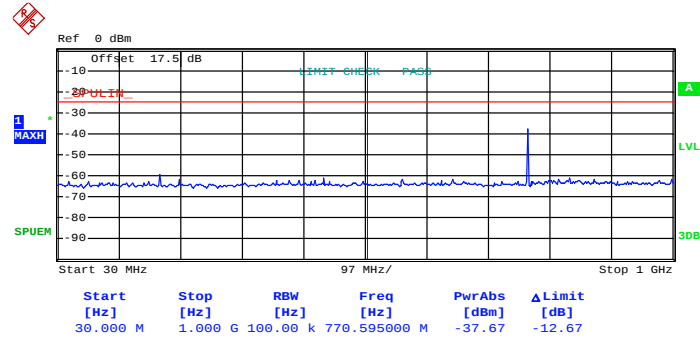
Conducted Emission Plot (30MHz ~ 1GHz) for QPSK (RB Size 1, RB Offset 24)
