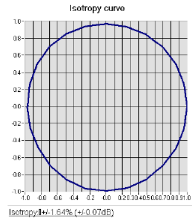
Isotropy at 1900 MHz
