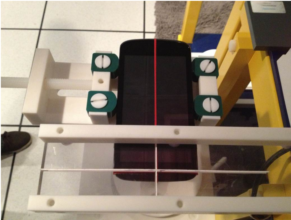
Fig.1 Test Configuration (Positioning)
