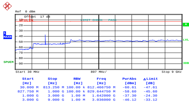
Conducted Emission Plot between on Channel 580 (820.50MHz)
