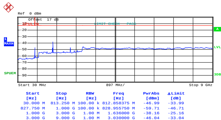
Conducted Emission Plot between on Channel 476 (817.90MHz)
