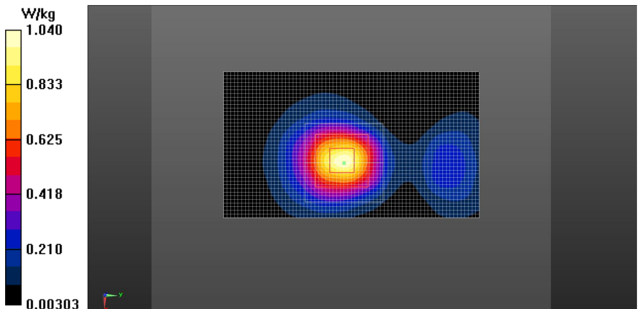
Fig.18 LTE Band 7
