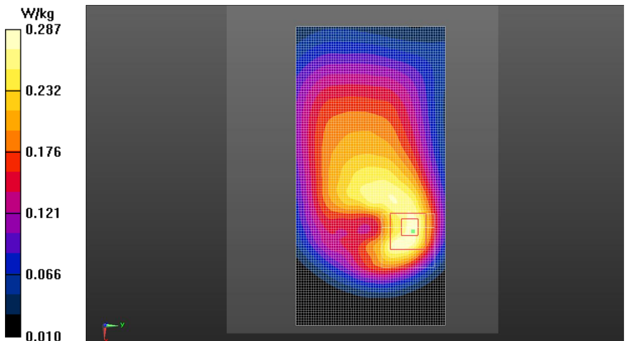
Fig.24 LTE Band 71
