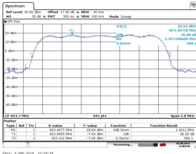
26dB Bandwidth Plot on Channel 1013 (824.7 MHz)
