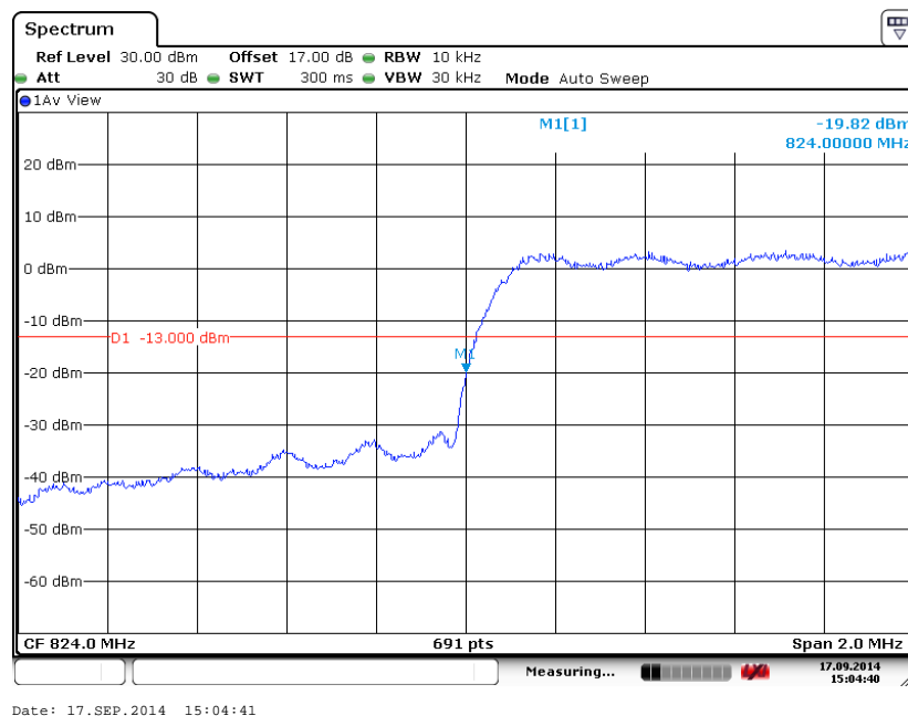
Lower Band Edge Plot on Channel 1013 (824.7 MHz)
