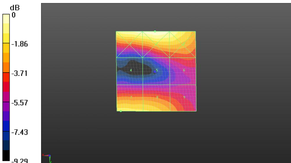
Fig B.4 HAC RF E-Field GSM 1900 High
