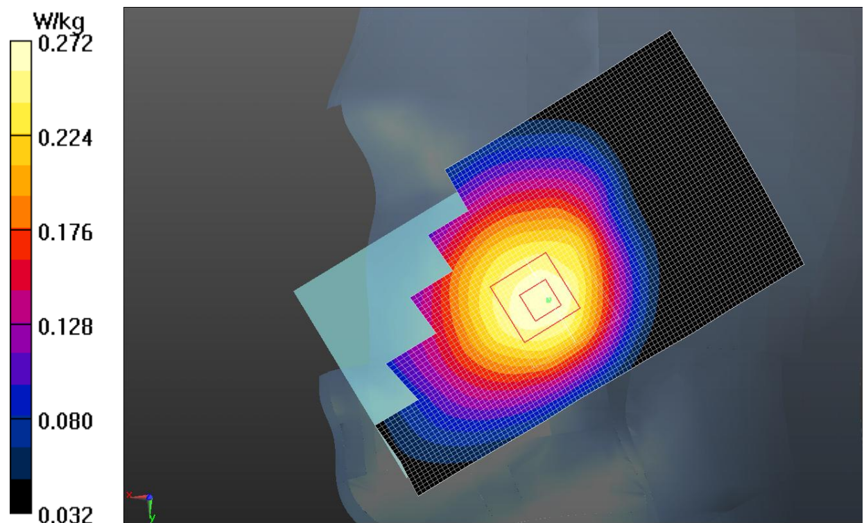
Fig.15 LTE Band 12
