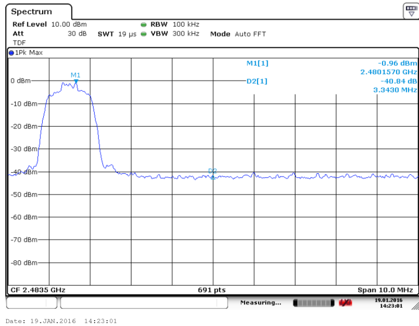
Fig. 19 Band Edges ( \pi/4 DQPSK, Ch 78, Hopping OFF)
