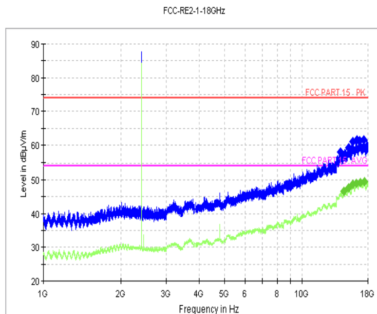
Fig.50 Radiated Spurious Emission (GFSK, Ch0, 1 GHz-18GHz)
