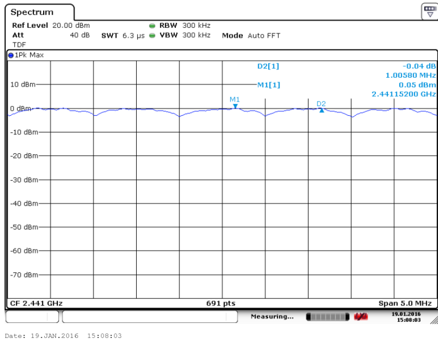
Fig. 95 Carrier Frequency Separation (8DPSK, Ch39)
