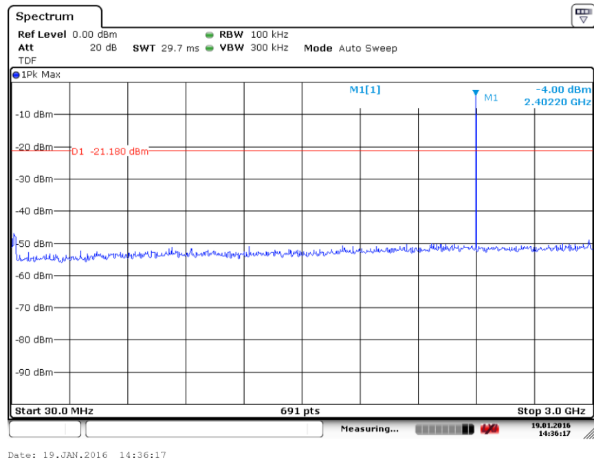
Fig. 41 Conducted Spurious Emission (8DPSK, Ch0, 30 MHz-3 GHz)
