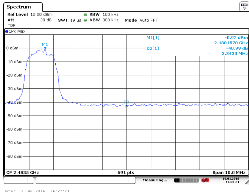
Fig. 21 Band Edges (8DPSK, Ch 78, Hopping OFF)
