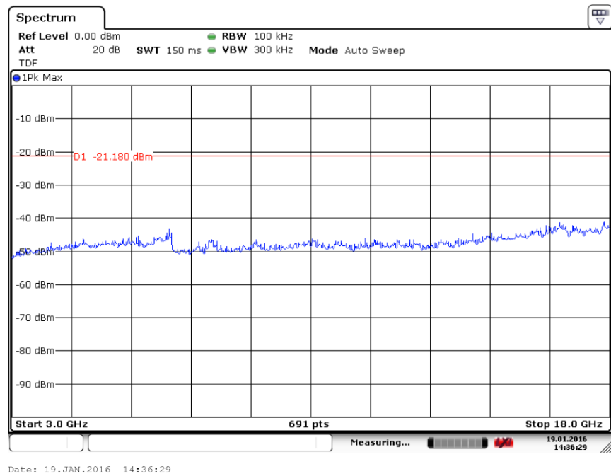
Fig. 42 Conducted Spurious Emission (8DPSK, Ch0, 3GHz-18 GHz)
