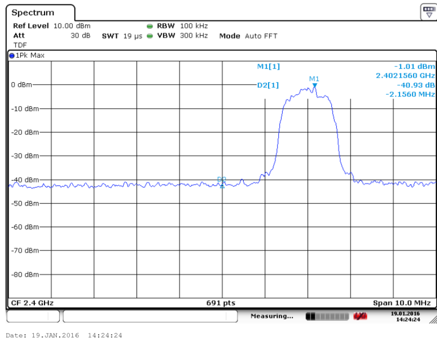
Fig. 20 Band Edges (8DPSK, Ch 0, Hopping OFF)
