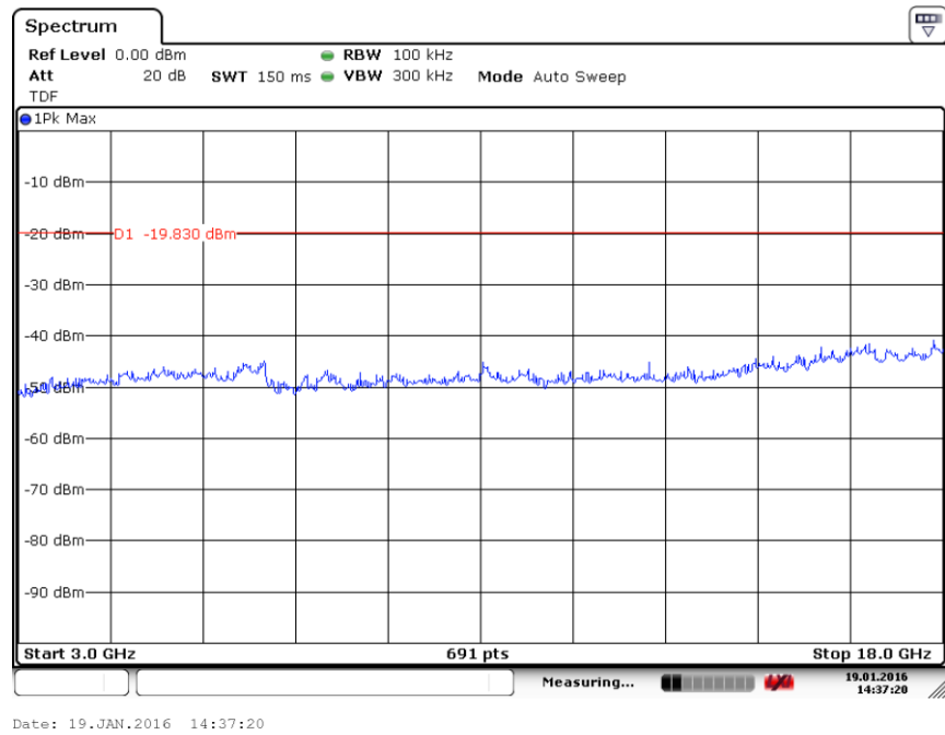
Fig. 45 Conducted Spurious Emission (8DPSK, Ch39, 3GHz-18 GHz)
