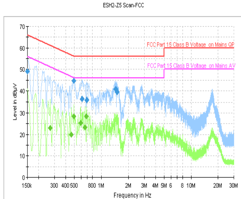
Fig. 97 AC Power line Conducted Emission (Idle, AE1)
