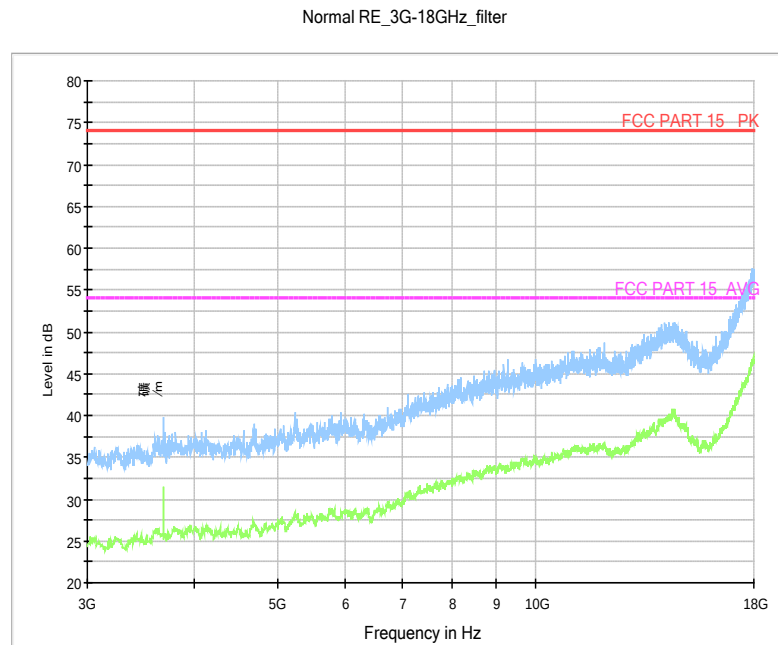
Fig.26 Radiated Spurious Emission (Ch19, 3 GHz-18 GHz)
