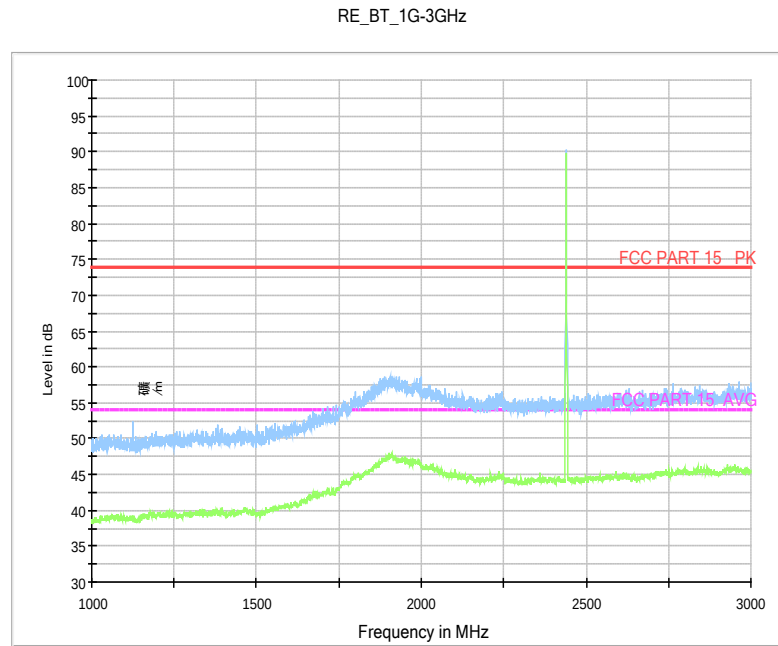
Fig.25 Radiated Spurious Emission (Ch19, 1 GHz-3 GHz)
