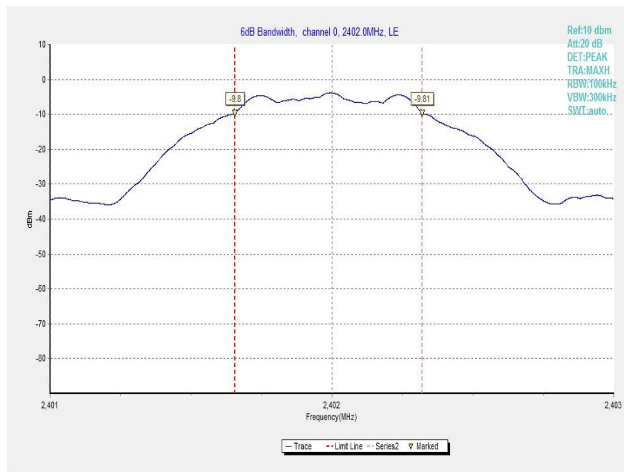
Fig.7 Occupied 6dB Bandwidth (Ch 0)
