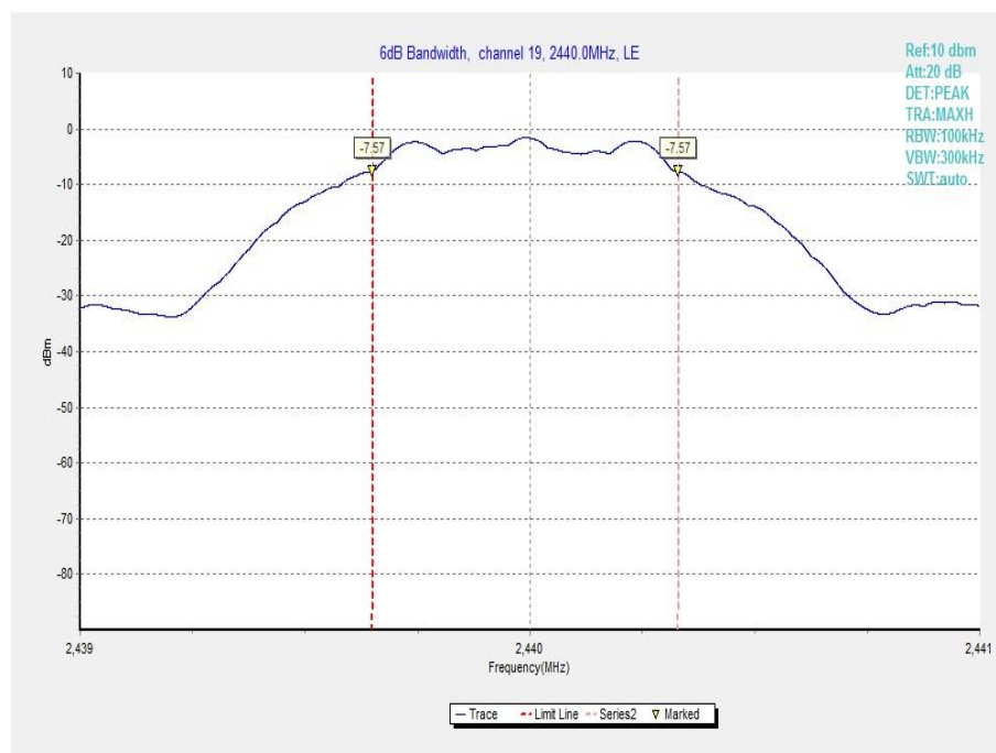
Fig.8 Occupied 6dB Bandwidth (Ch 19)
