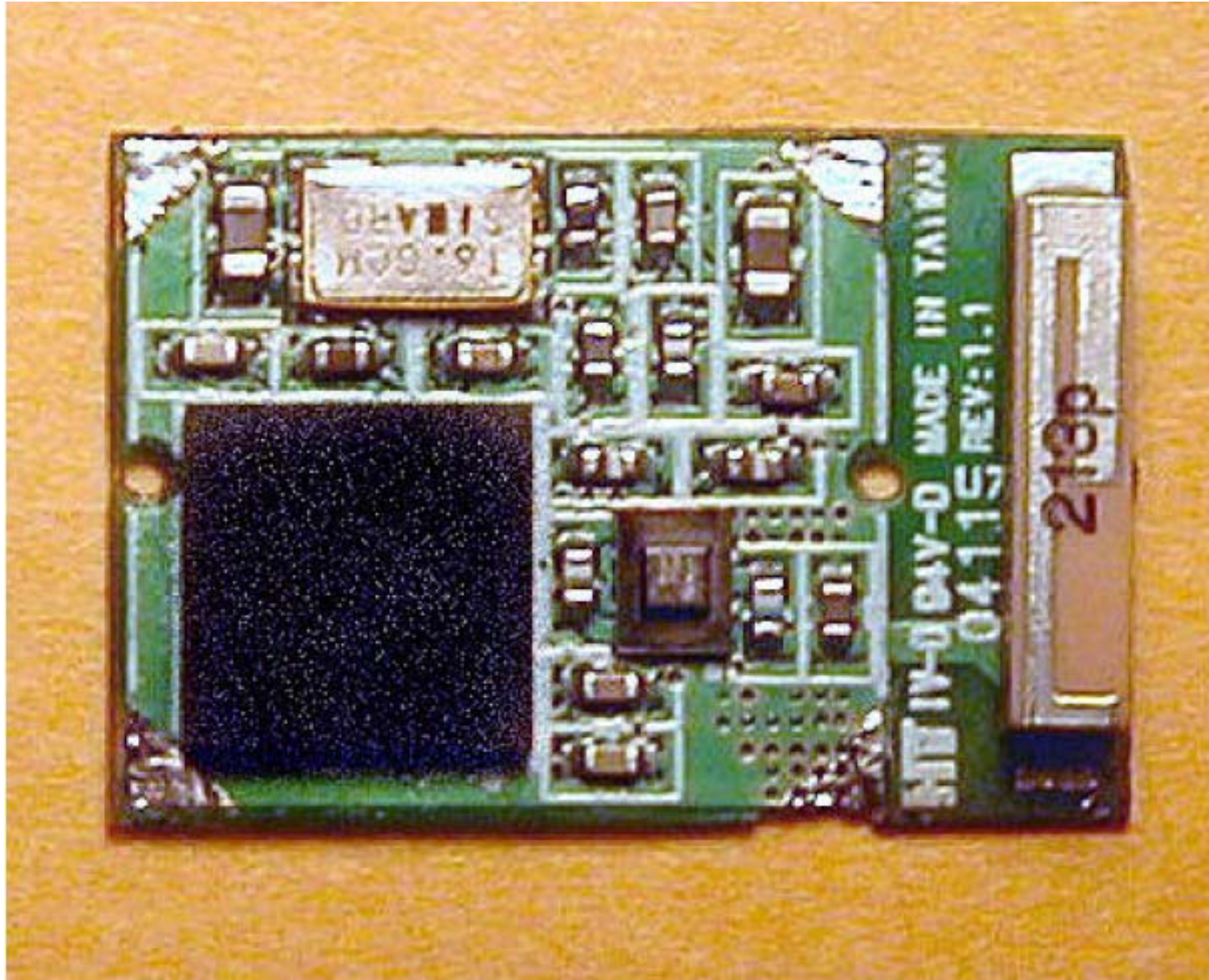
Annex 3 – Internal Photographs of EUT DATAWIND Bluetooth Module, Model No.: DW-SBTM1
