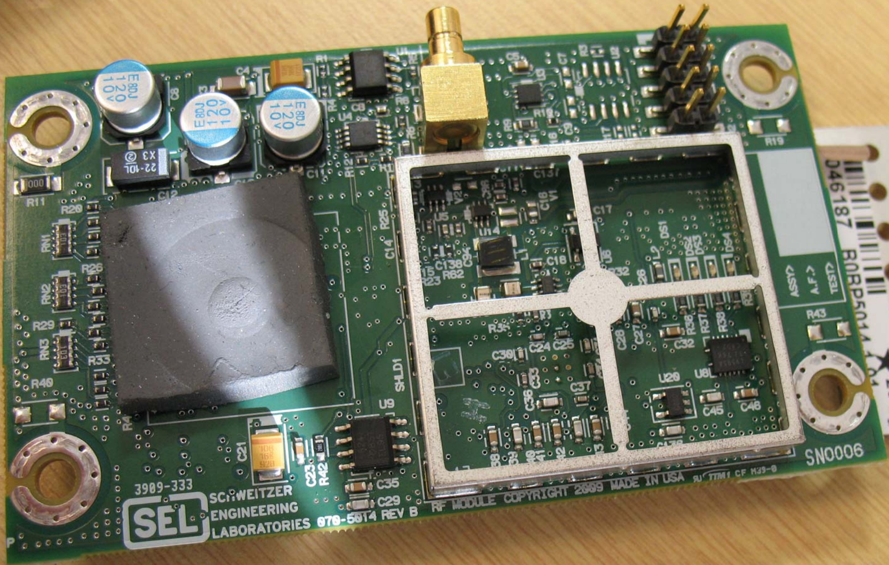
RF board without shield
