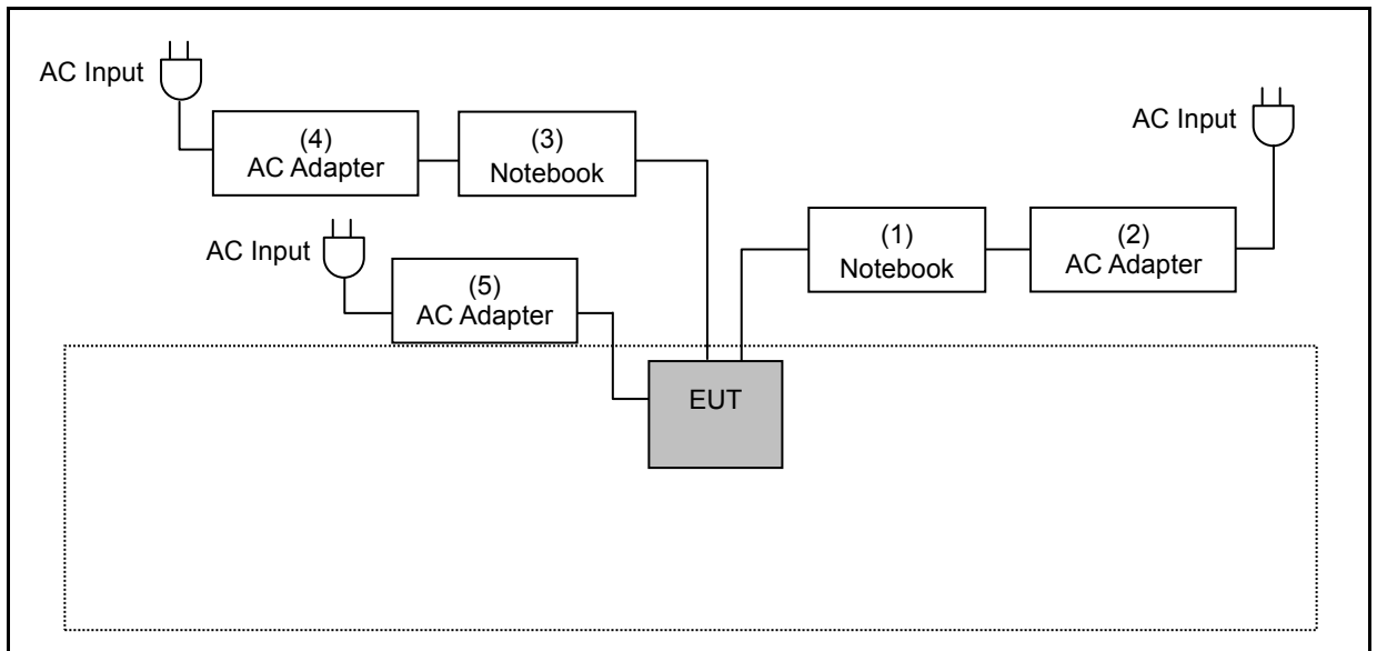
Radiated Emission
