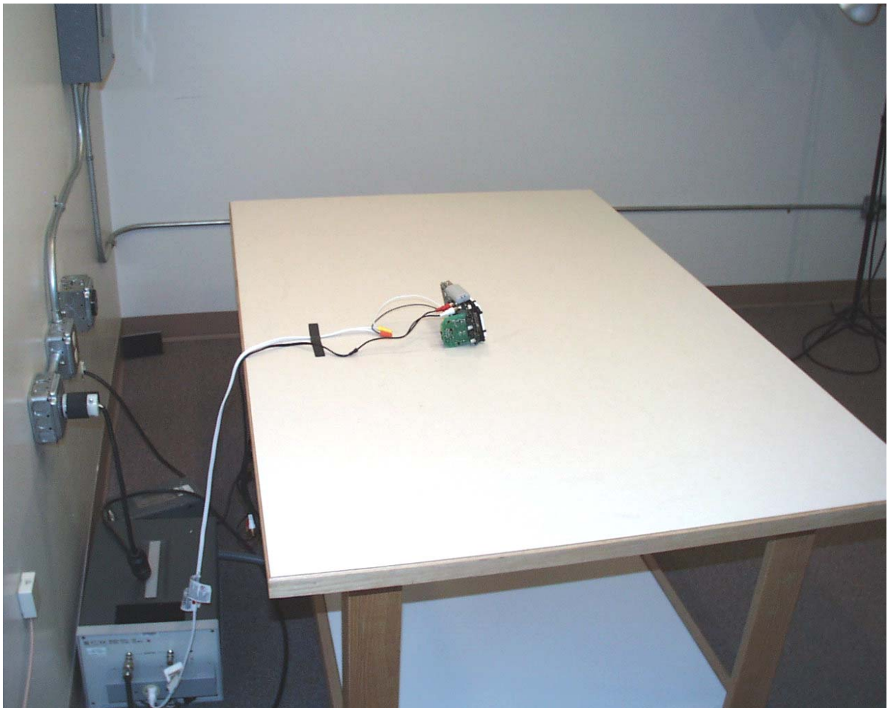
Back View Conducted Disturbance Worst Case Configuration
