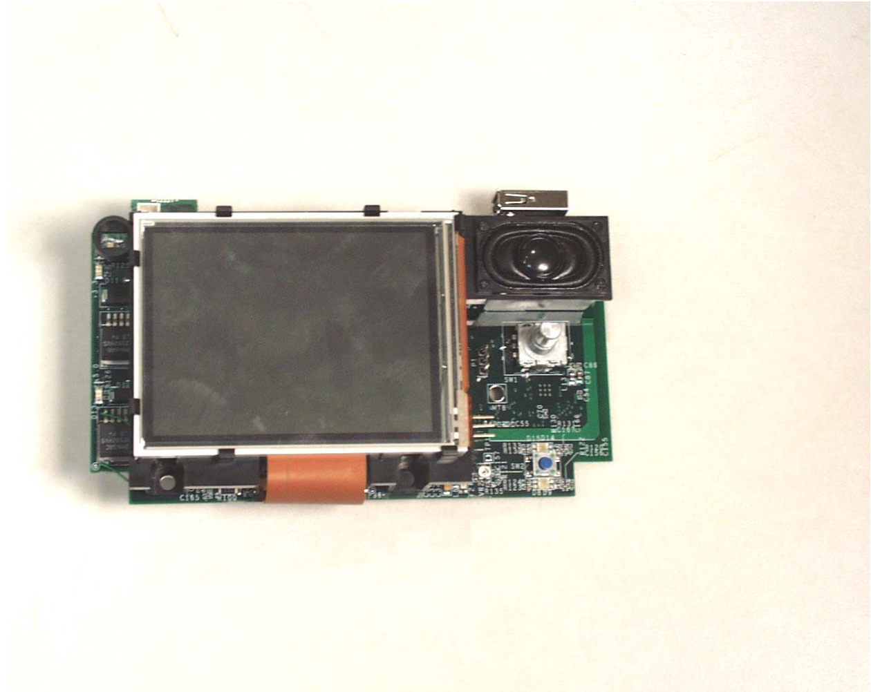
Photograph 7 - Front View of the EUT without the USB Devices Installed
