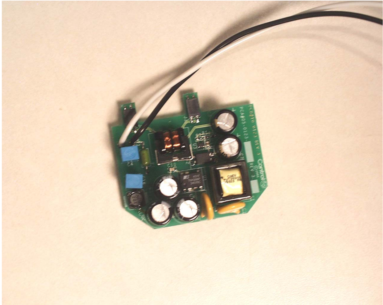
Photograph 12 - View of the Component Side of the Power Supply Module
