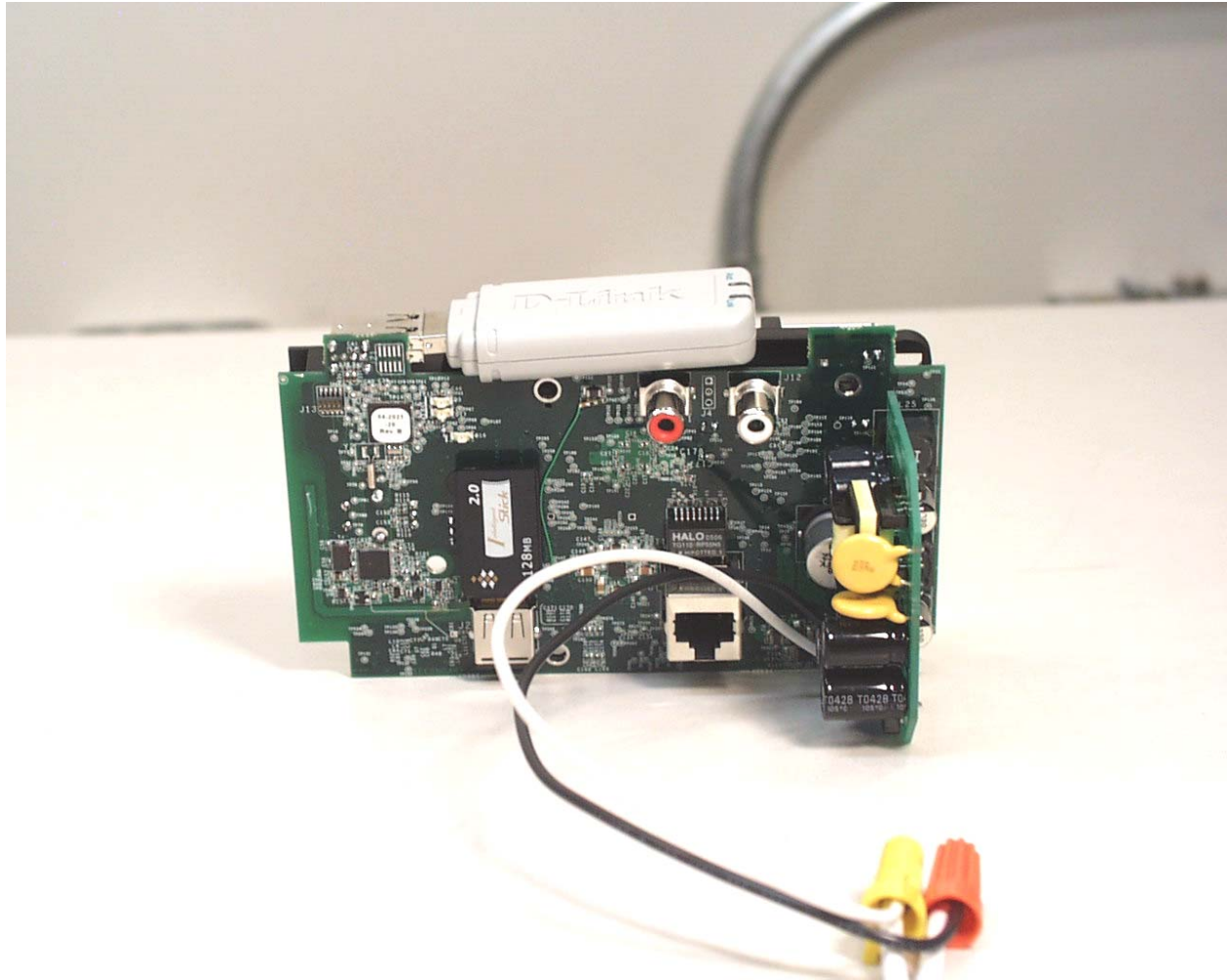
Photograph 6 - Back View of the EUT with the USB Devices Installed
