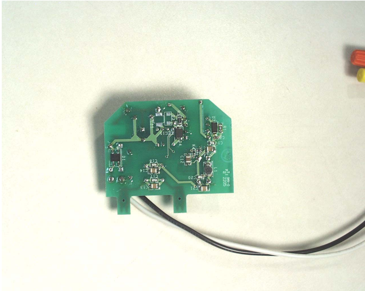
Photograph 13 - View of the Trace Side of the Power Supply Module
