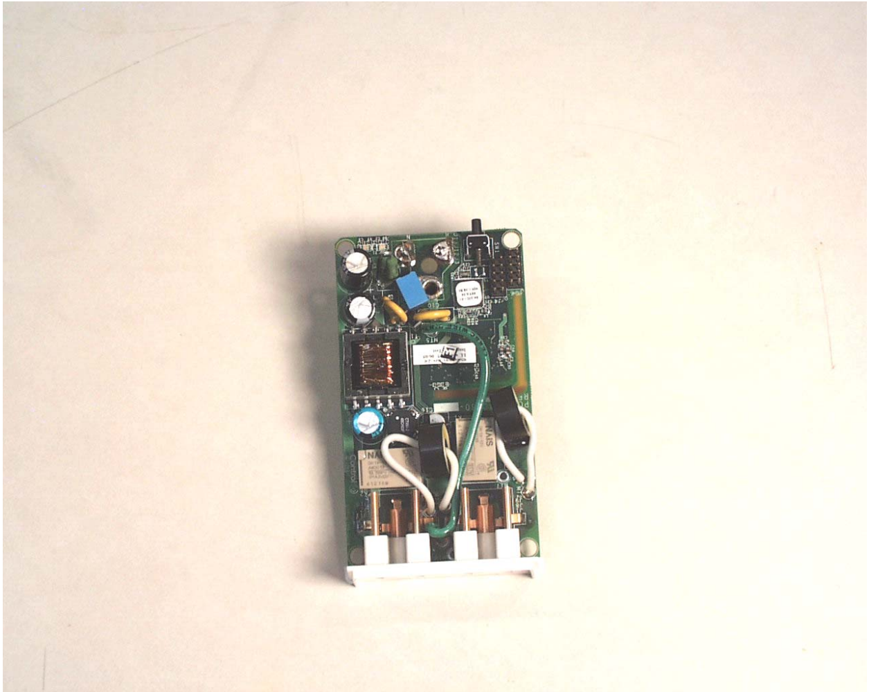
View Component Side of the EUT PCB
