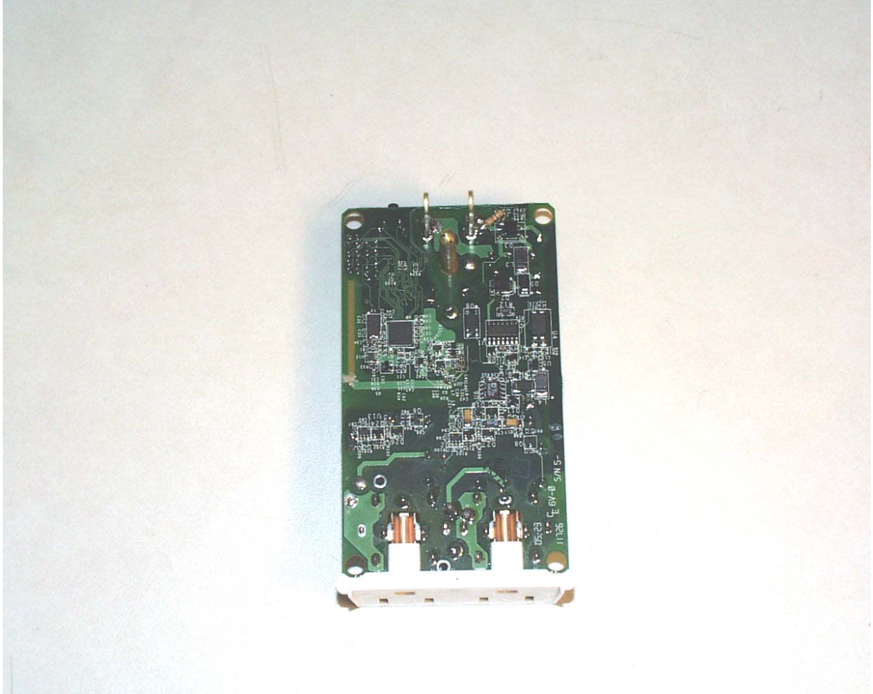
View of the Trace Side of the EUT PCB
