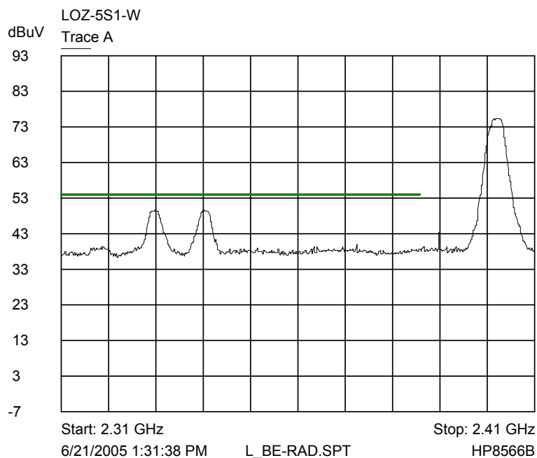
Trace A Lower channel corrected band edge plot - peak detection
