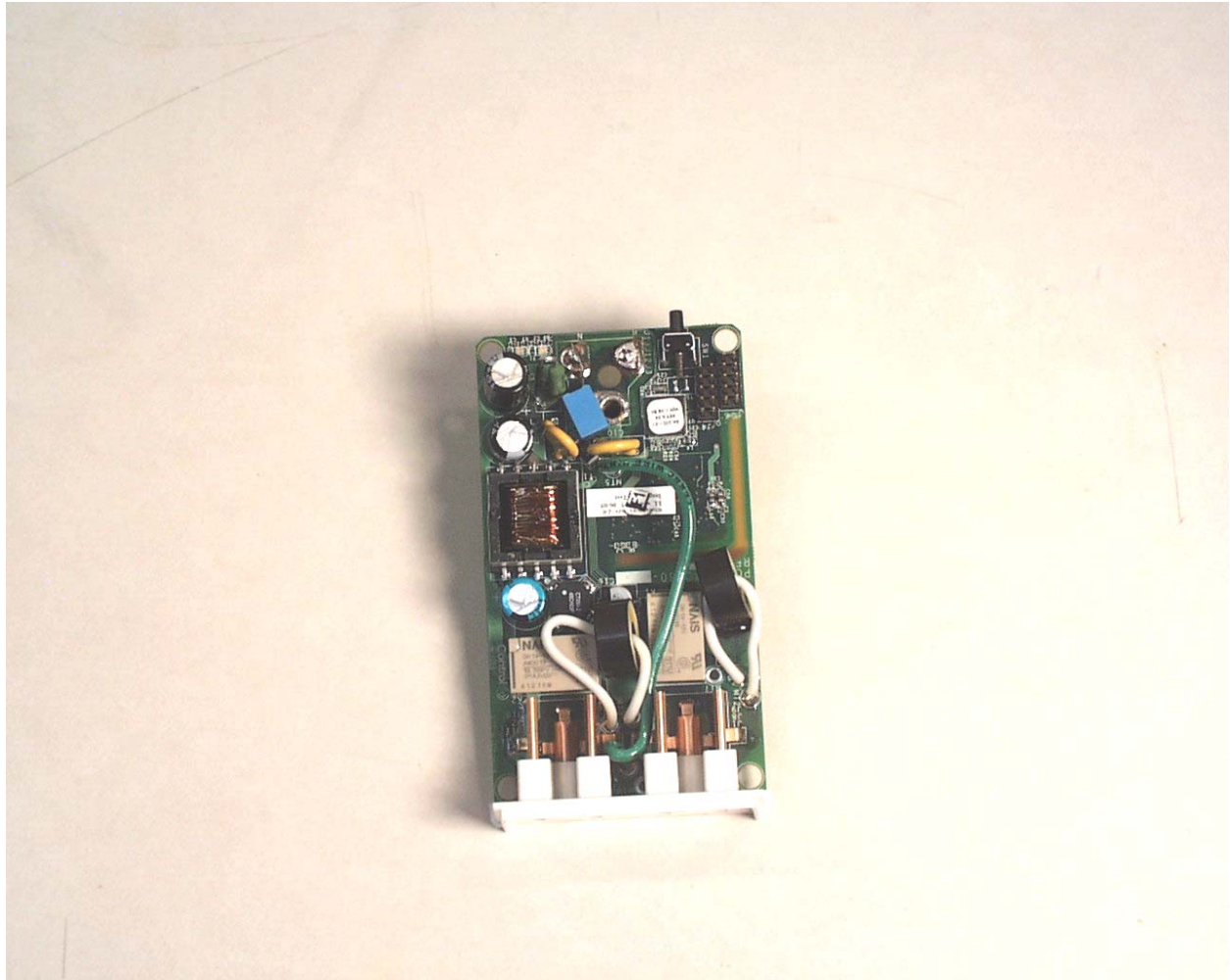
Photograph 5 -View Component Side of the EUT PCB
