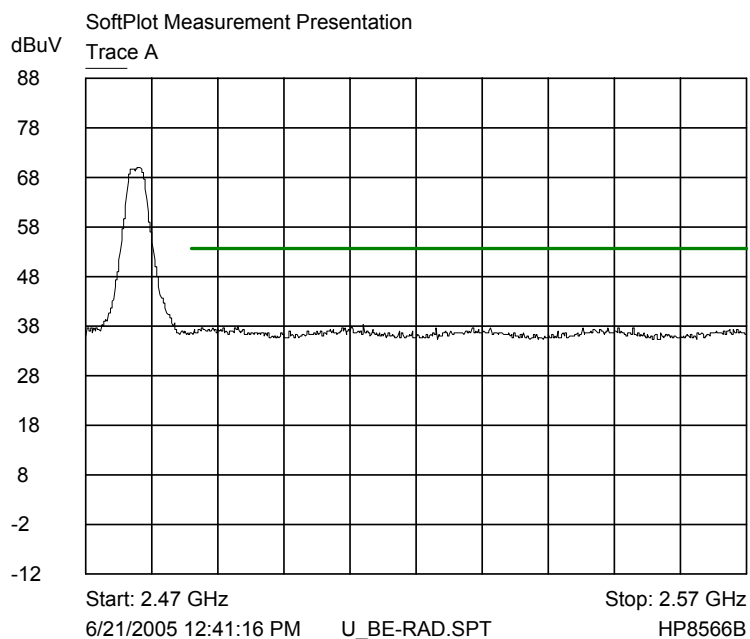
Trace A Upper channel corrected band edge plot - peak detection
