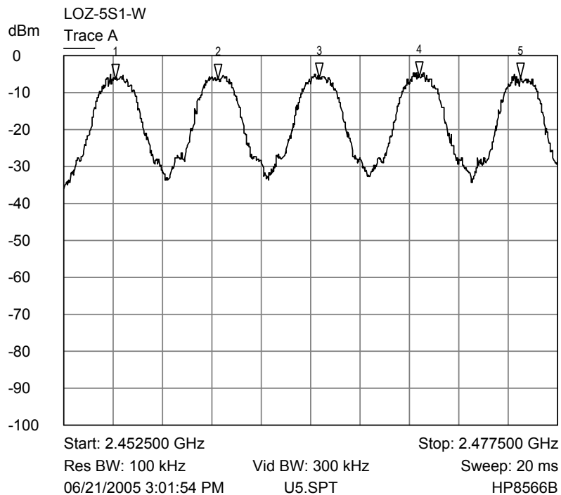
Trace A Upper 5 channel plot
