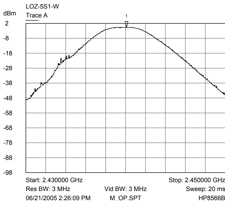
Trace A Middle channel output power plot
