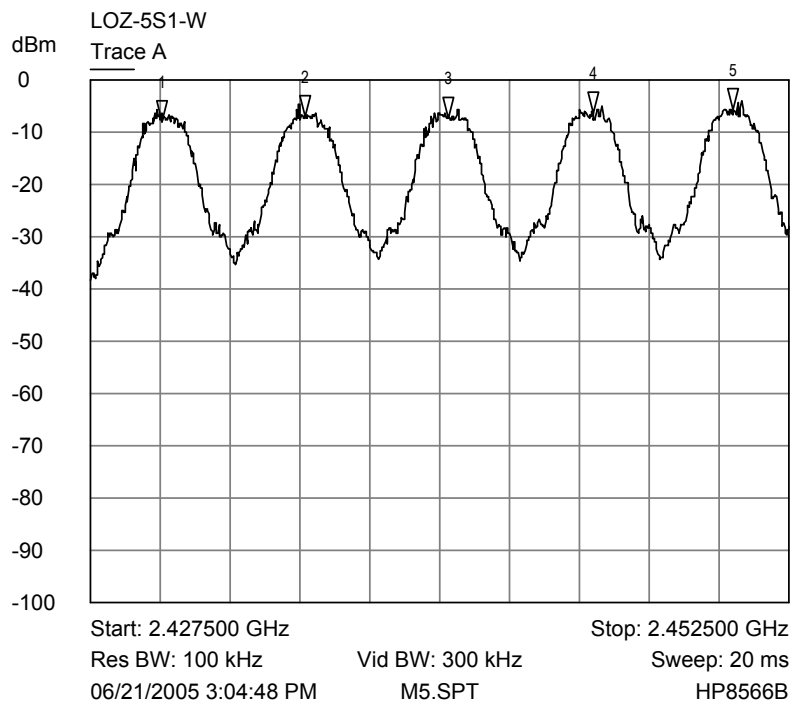
Trace A Middle 5 channel plot
