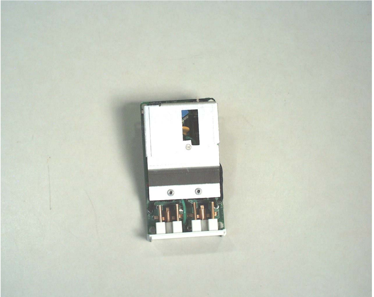
Top Side of the PCB with Heatsink
