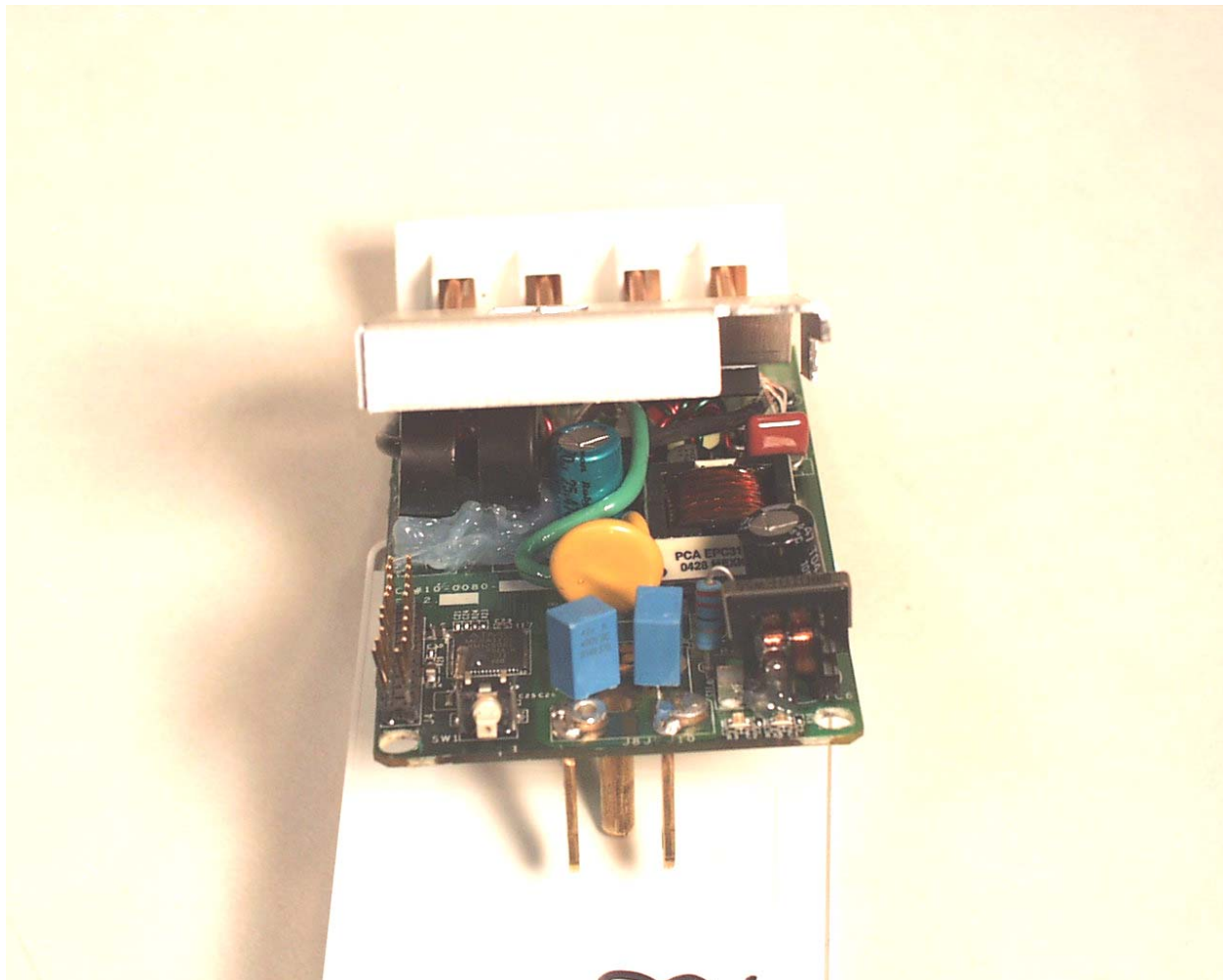
Top Side of the PCB Under Heatsink
