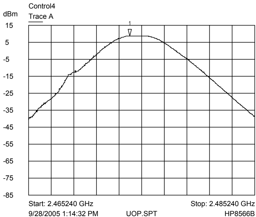
Trace A Upper channel output power plot
