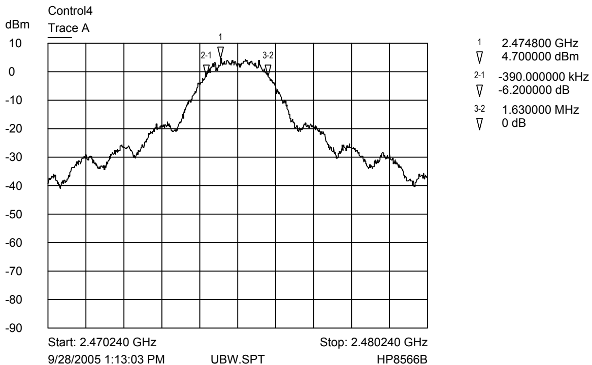
Trace A Upper channel bandwidth plot
