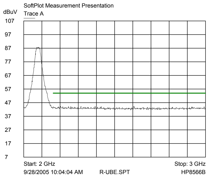
Trace A Upper band edge radiated &amp; corrected - peak detection plot
