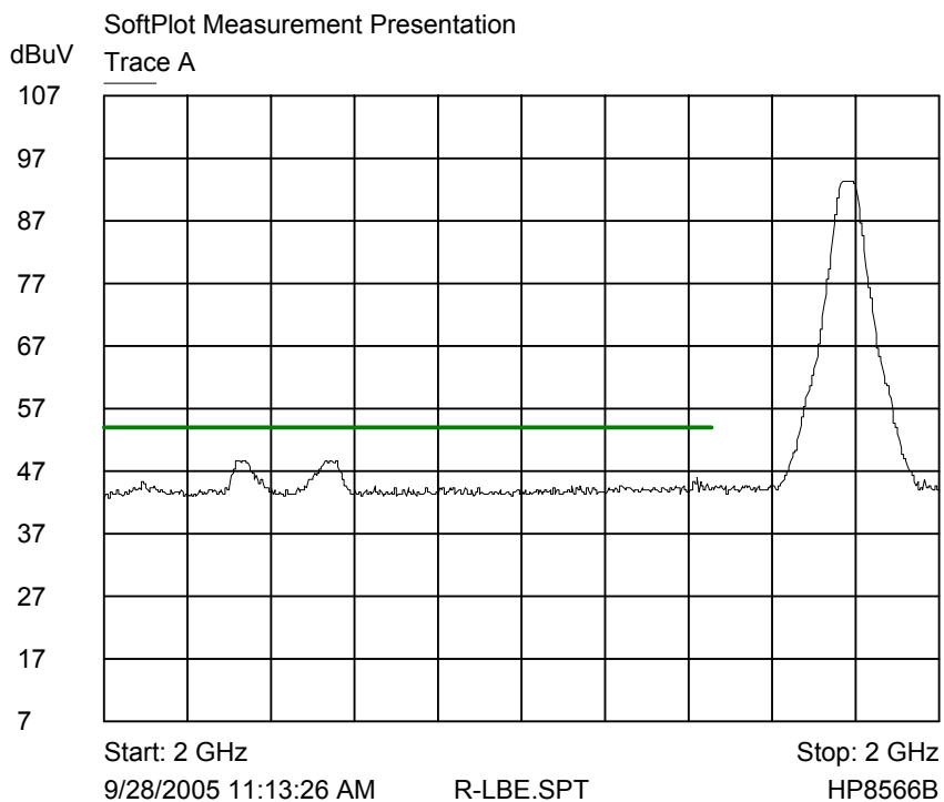
Trace A Lower band edge radiated &amp; corrected - peak detection plot
