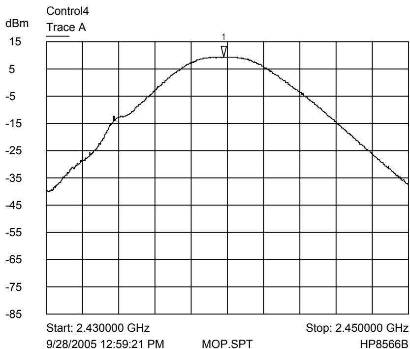
Trace A Middle channel output power plot
