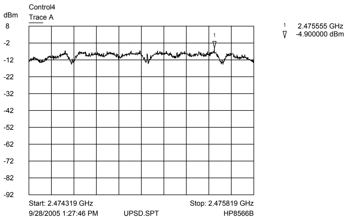
Trace A Upper channel 3kHz power spectral density plot
