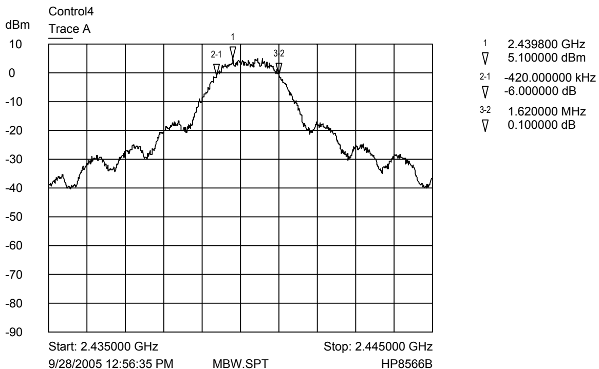
Trace A Middle channel bandwidth plot
