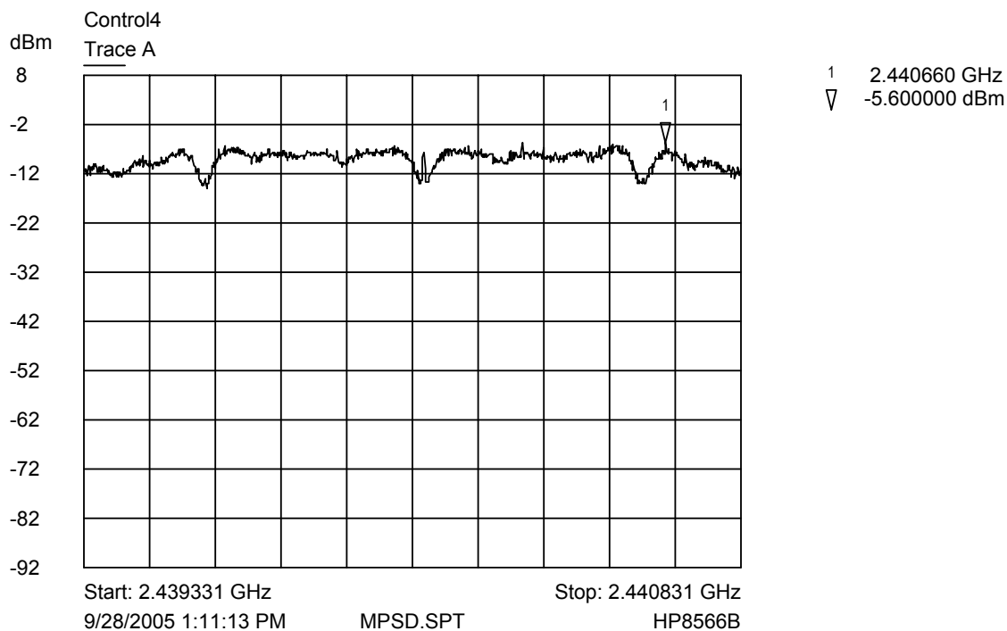
Trace A Middle channel 3kHz power spectral density plot
