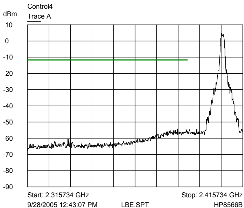
Trace A Lower channel band edge plot
