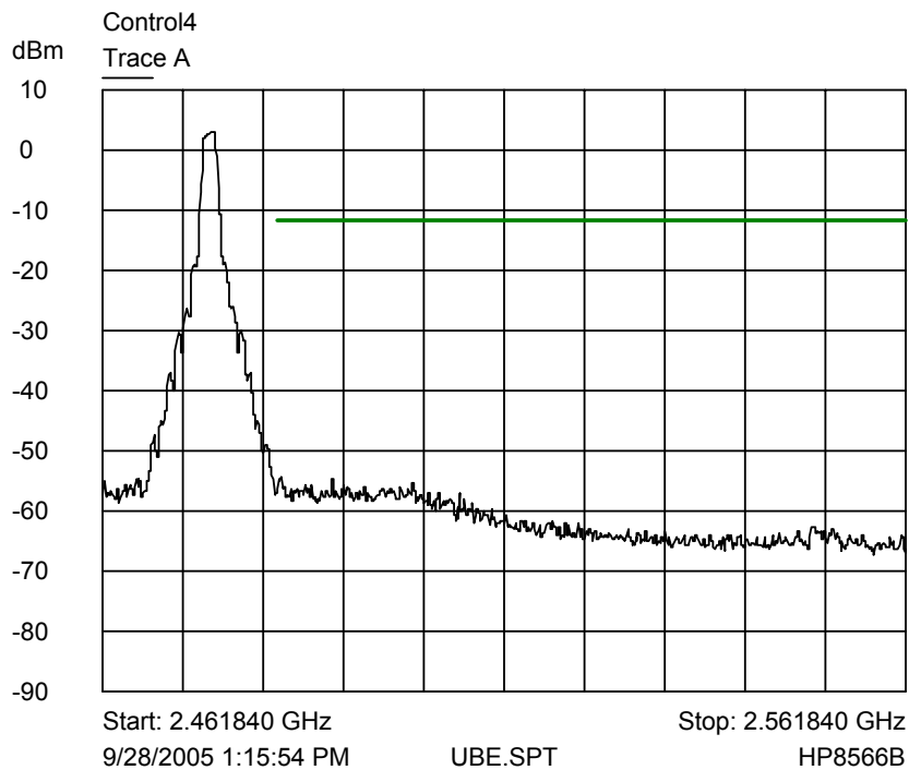
Trace A Upper channel band edge plot
