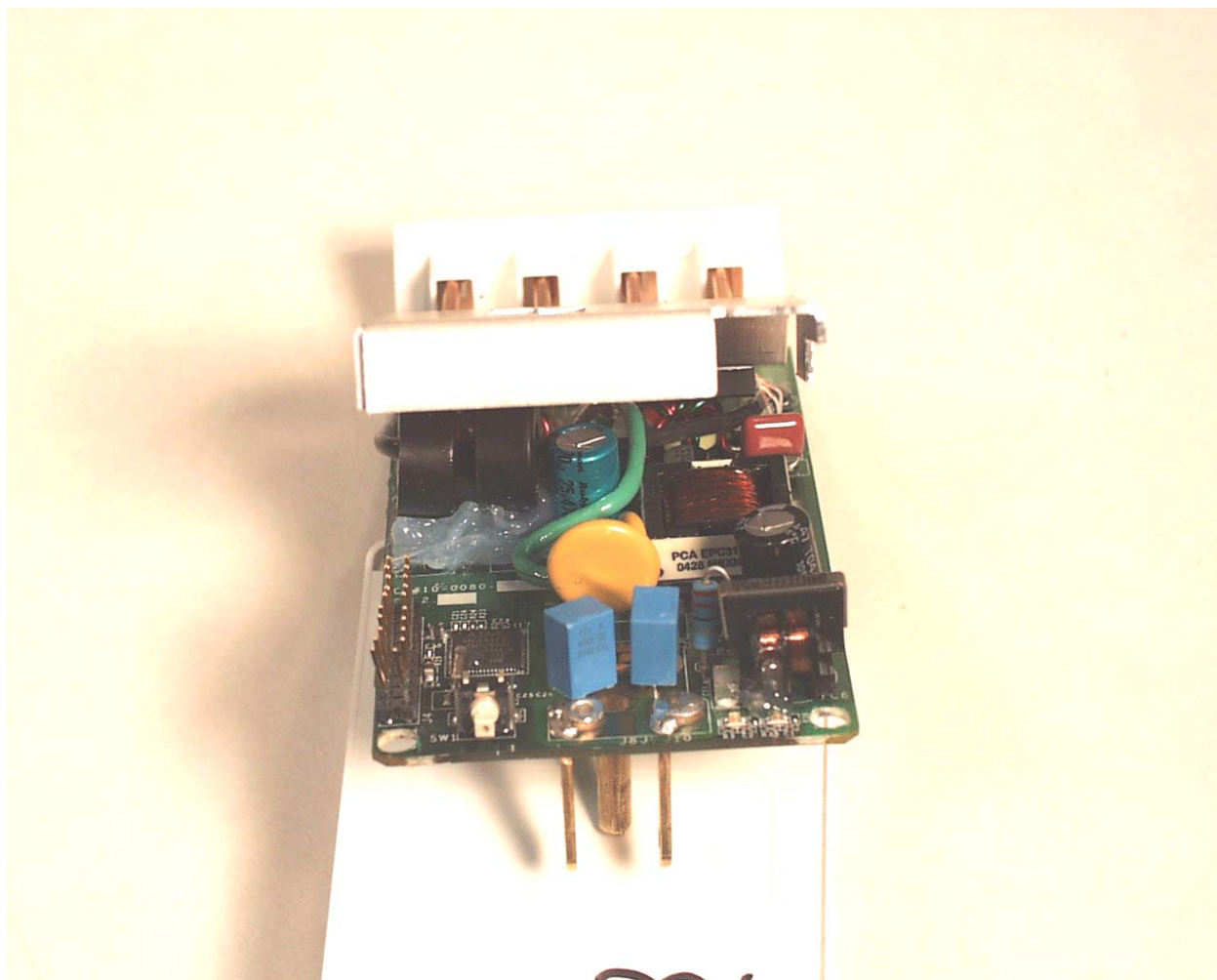
Photograph 9 - Top Side of the PCB Under Heatsink
