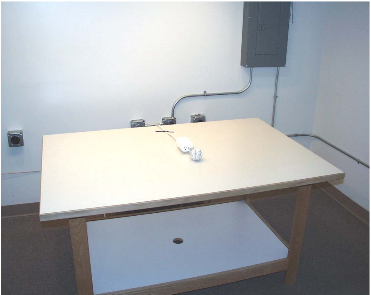
Front View Conducted Disturbance Worst Case Configuration
