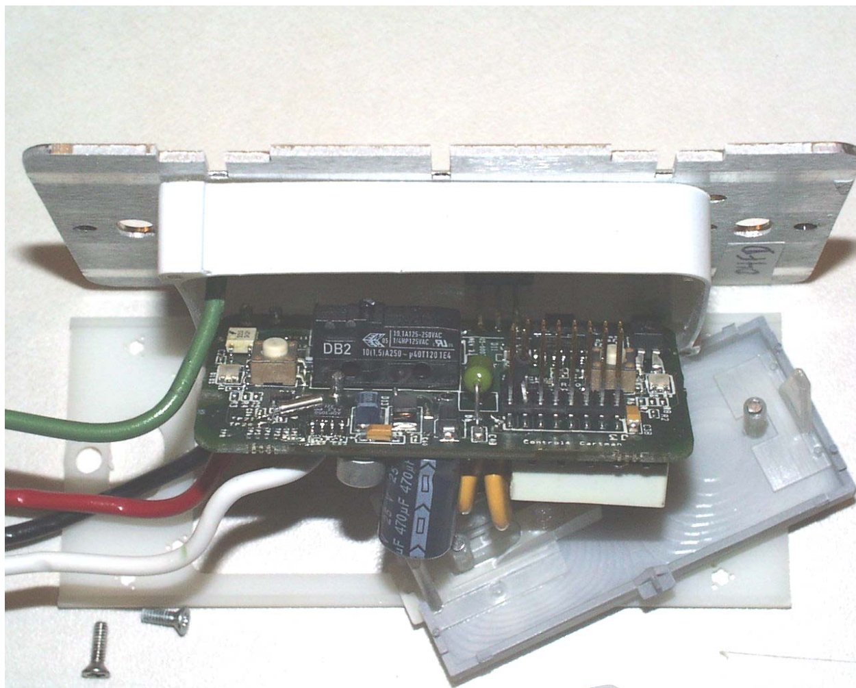
Photograph 8 - View of Side B of the Host Card
