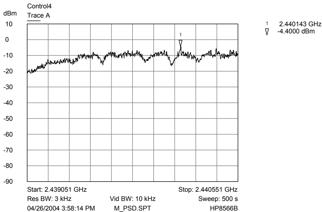
Middle channel power spectral density
