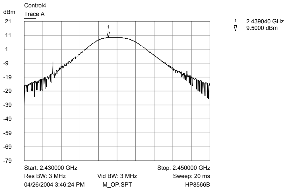
Middle channel output power
