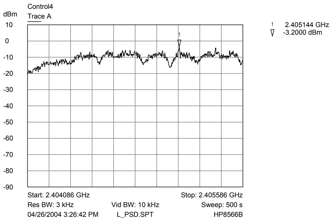
Low channel power spectral density
