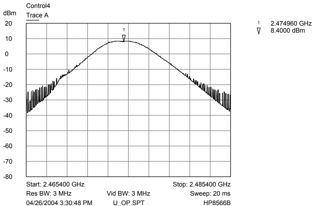
Upper channel output power
