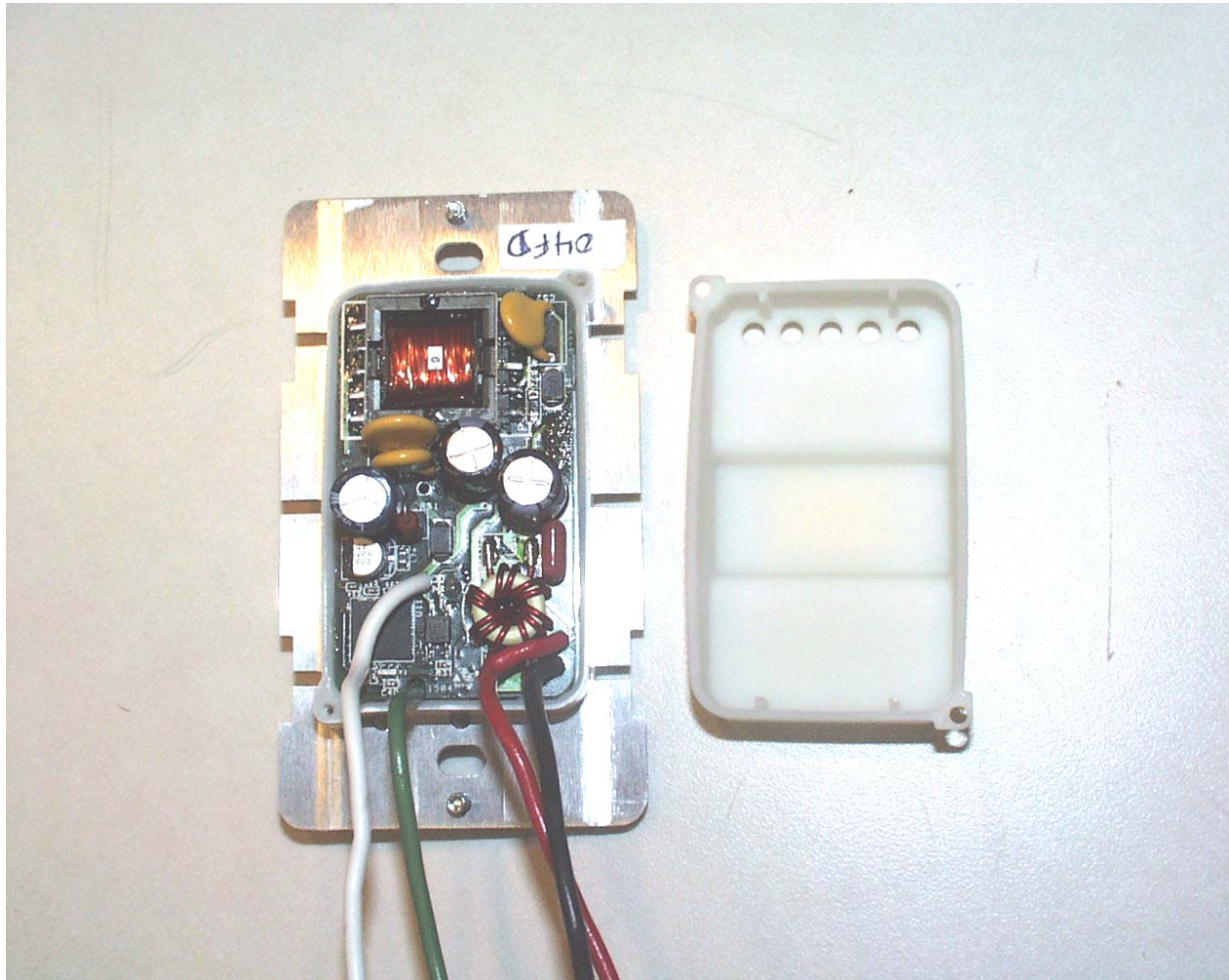
Photograph 7 - View of Side A of the Host Card
