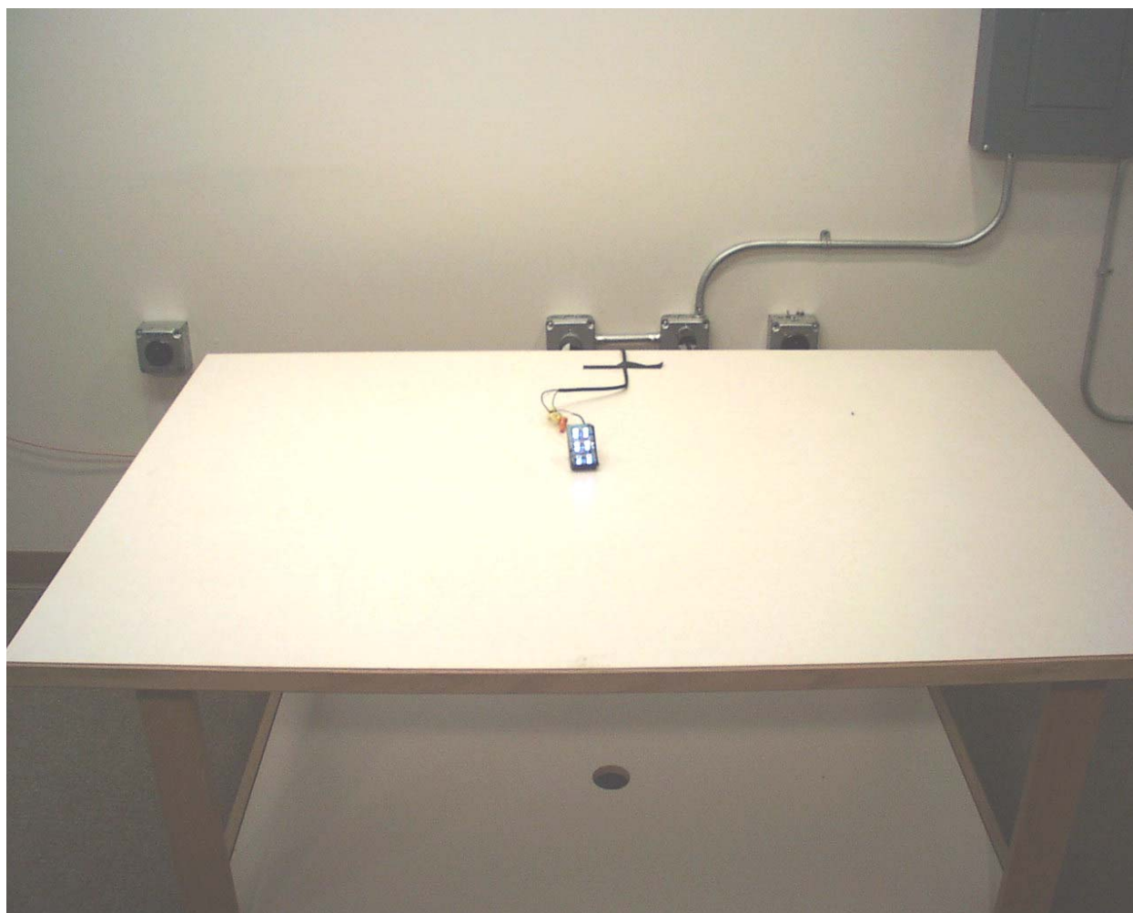
Photograph 3 – Front View Conducted Disturbance Worst Case Configuration
