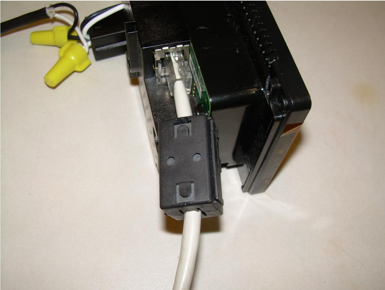
Ferrite Placement on Ethernet Cable
