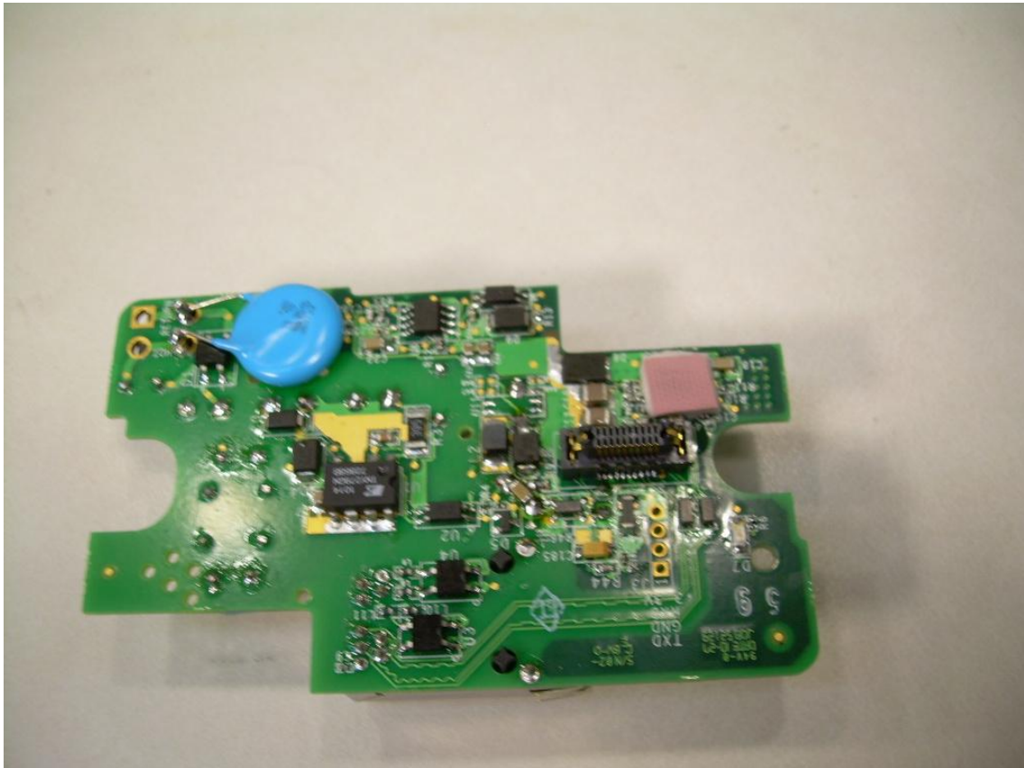
Photograph 15 - View of the Interface Side of the Power Supply/Interface PCB with Heatsink Removed
