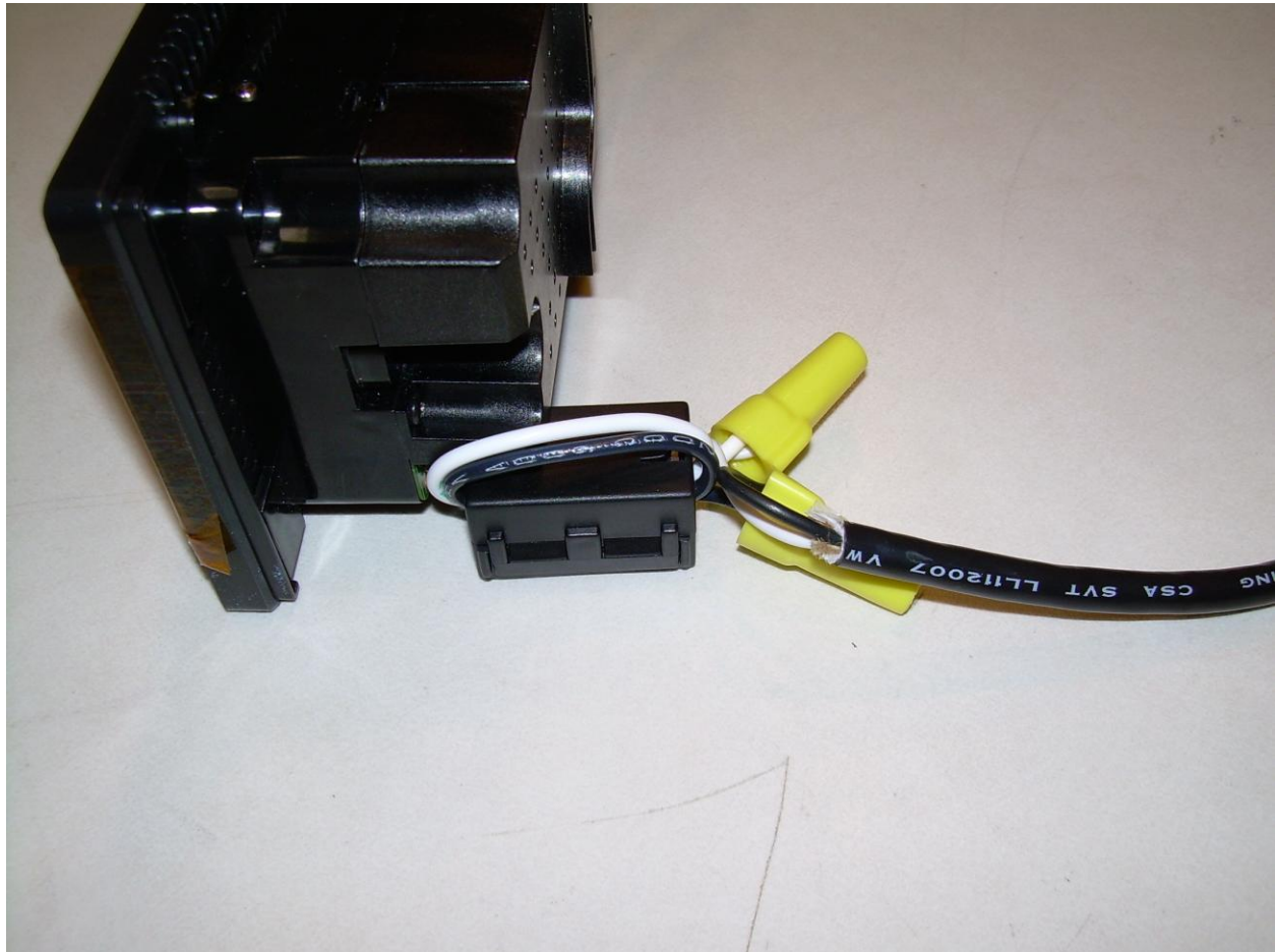
Photograph 5 – Ferrite Placement on AC Mains Flying Leads
