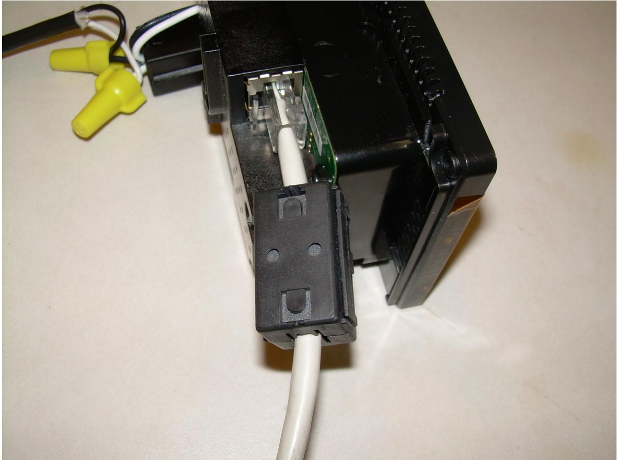
Photograph 6 - Ferrite Placement on Ethernet Cable
