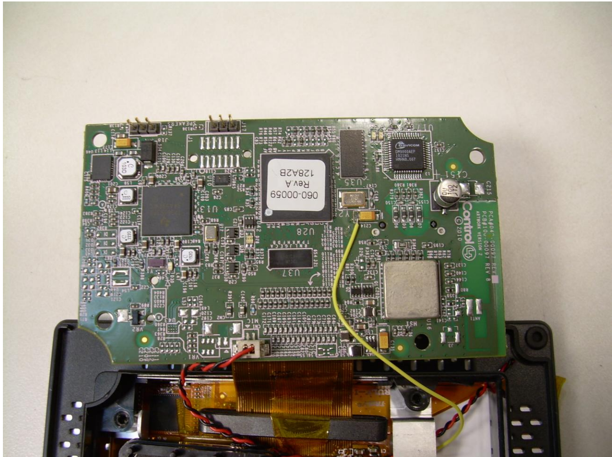
Photograph 11 – View of the Component Side of the Main PCB
