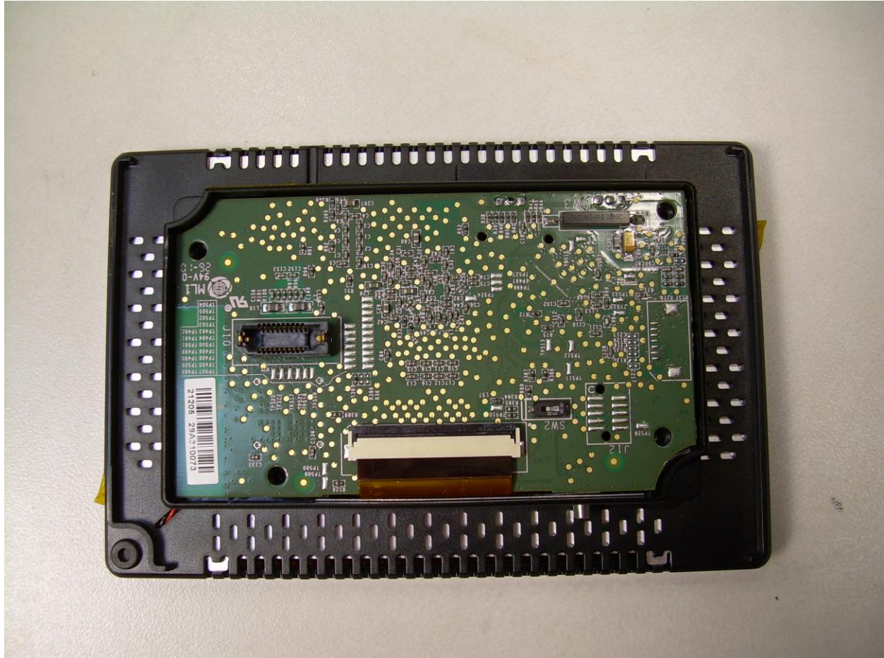
Photograph 10 – View of the Interface Side of the Display PCB
