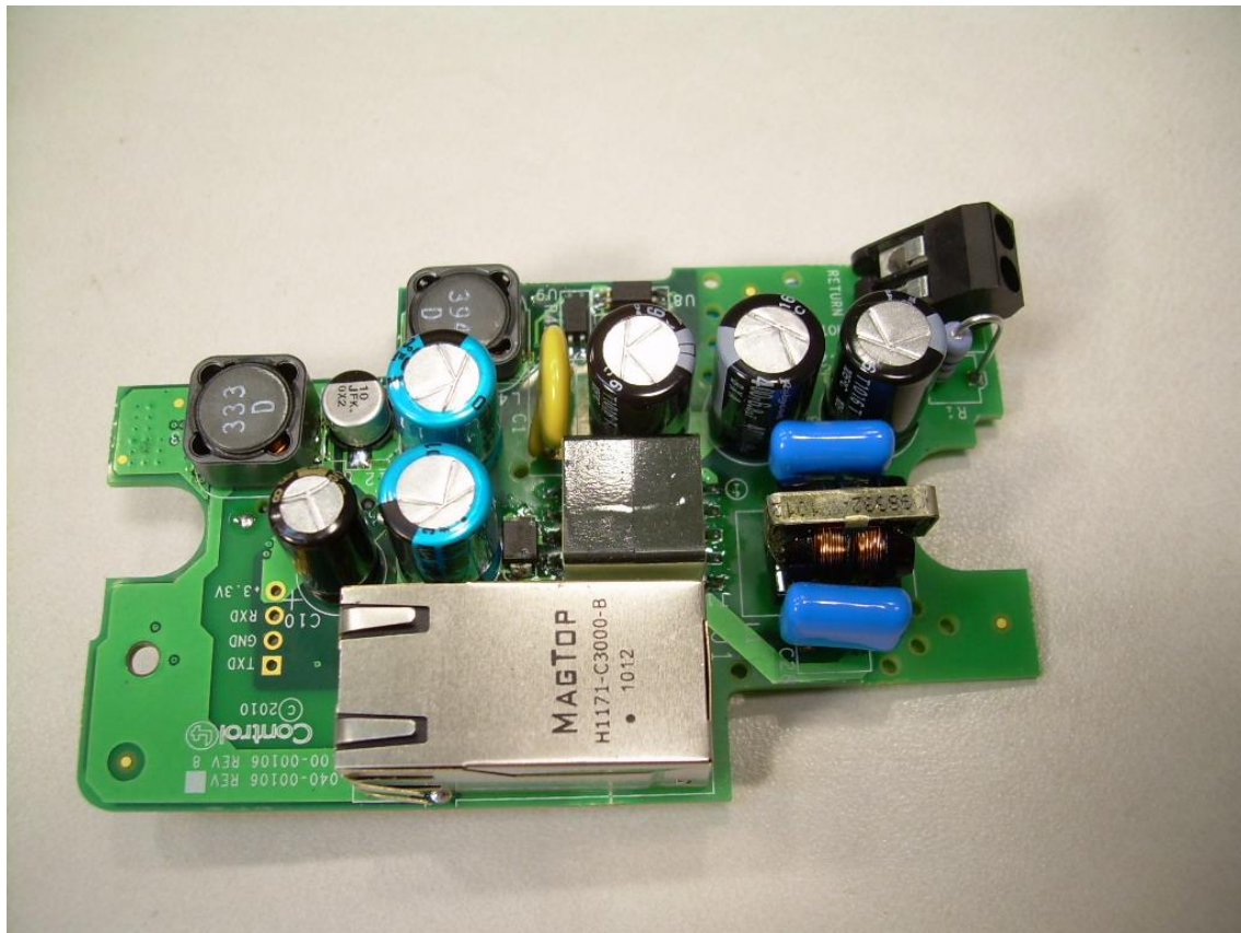
Photograph 17 - View of the Component Side of the Power Supply/Interface PCB with Heatsink Removed
