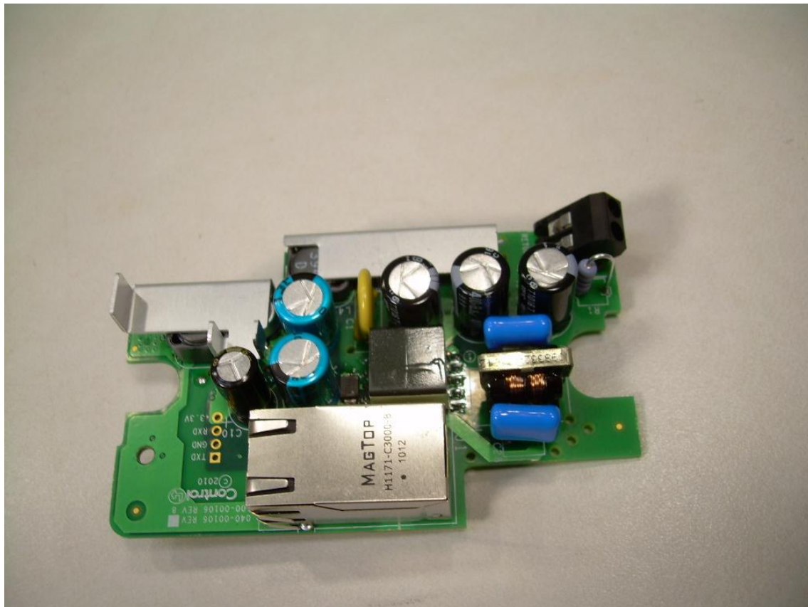
Photograph 16 - View of the Component Side of the Power Supply/Interface PCB with Heatsink in Place
