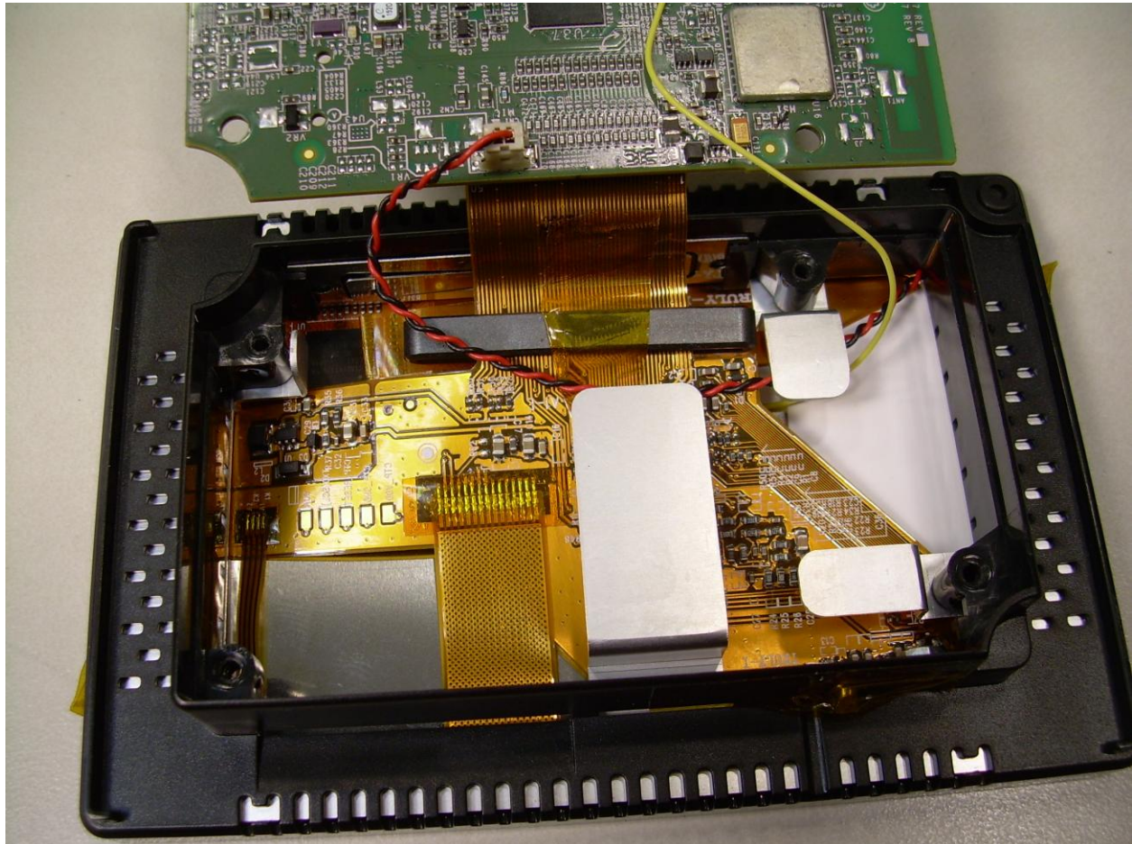
Photograph 9 – View of the Component Side of the Display PCB showing Ferrite on Flex Cable
