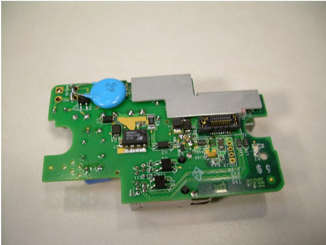
View of the Interface Side of the Power Supply/Interface PCB with Heatsink in Place
