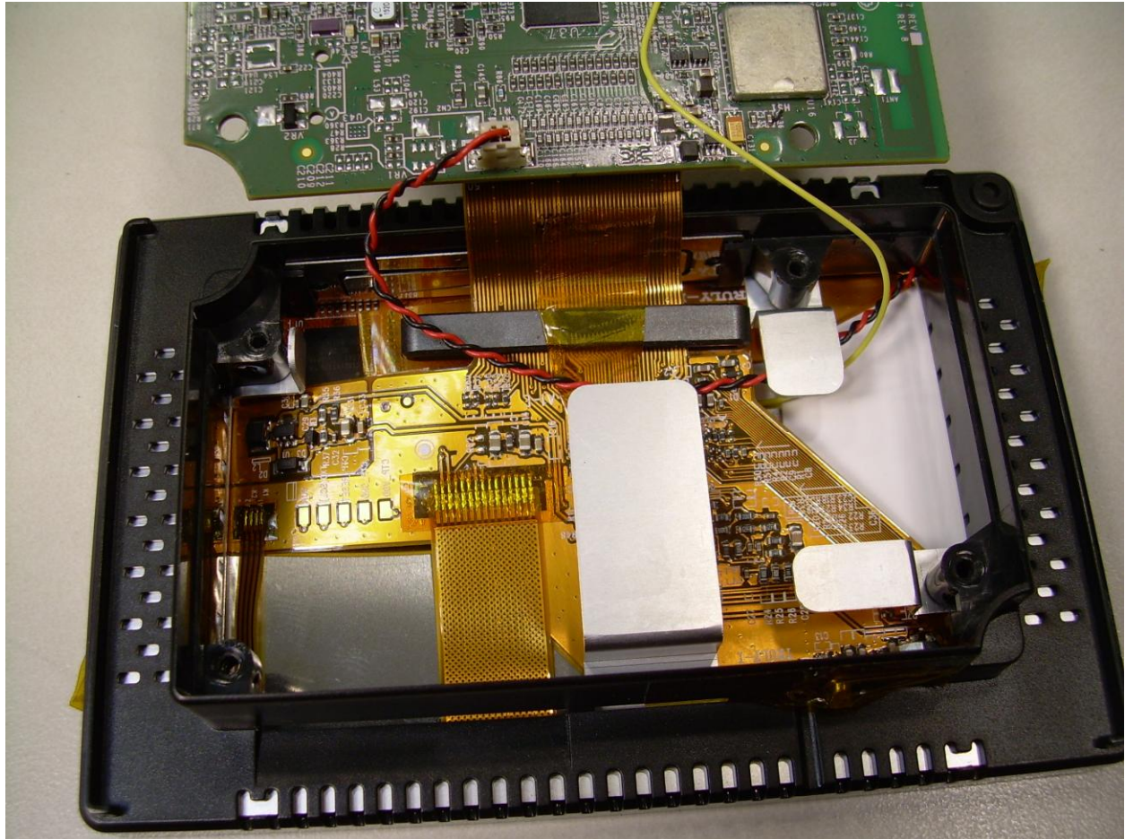
View of the Component Side of the Display PCB showing Ferrite on Flex Cable
