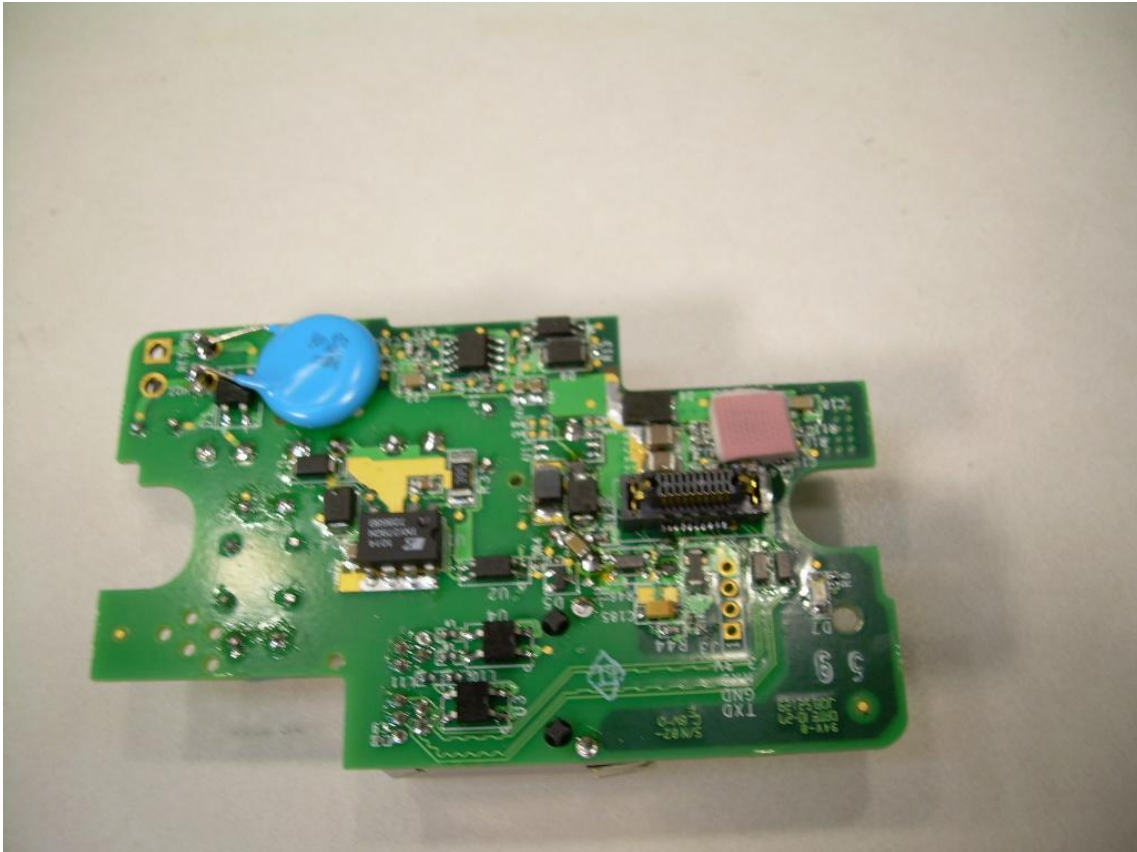
View of the Interface Side of the Power Supply/Interface PCB with Heatsink Removed
