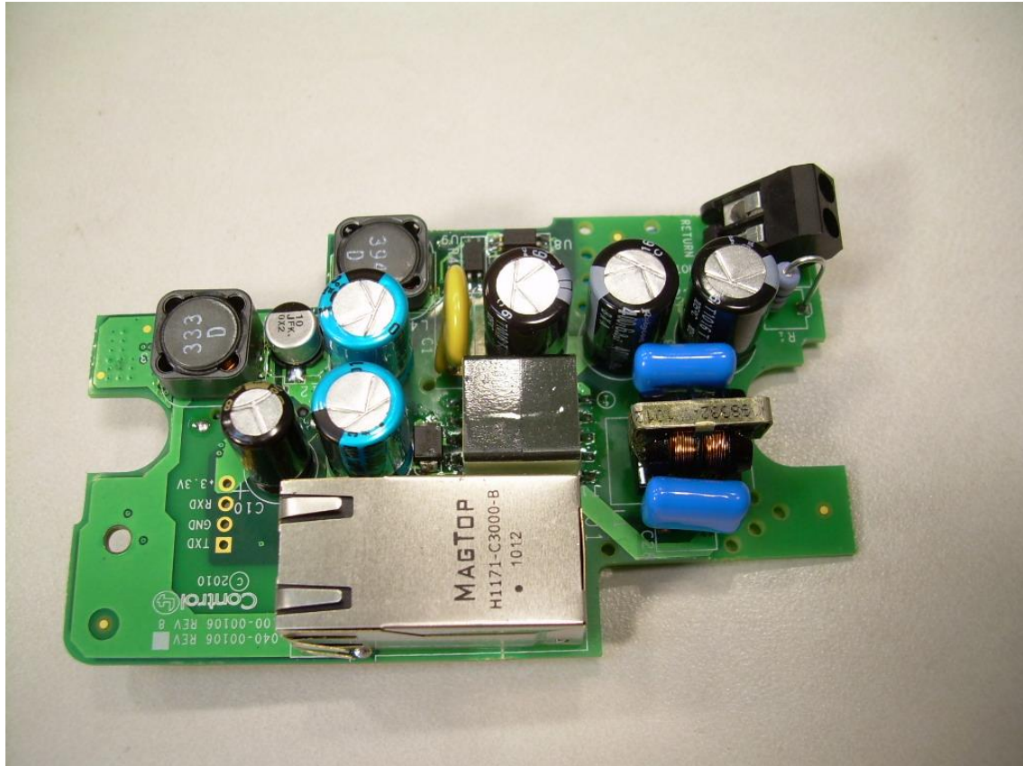
View of the Component Side of the Power Supply/Interface PCB with Heatsink Removed
