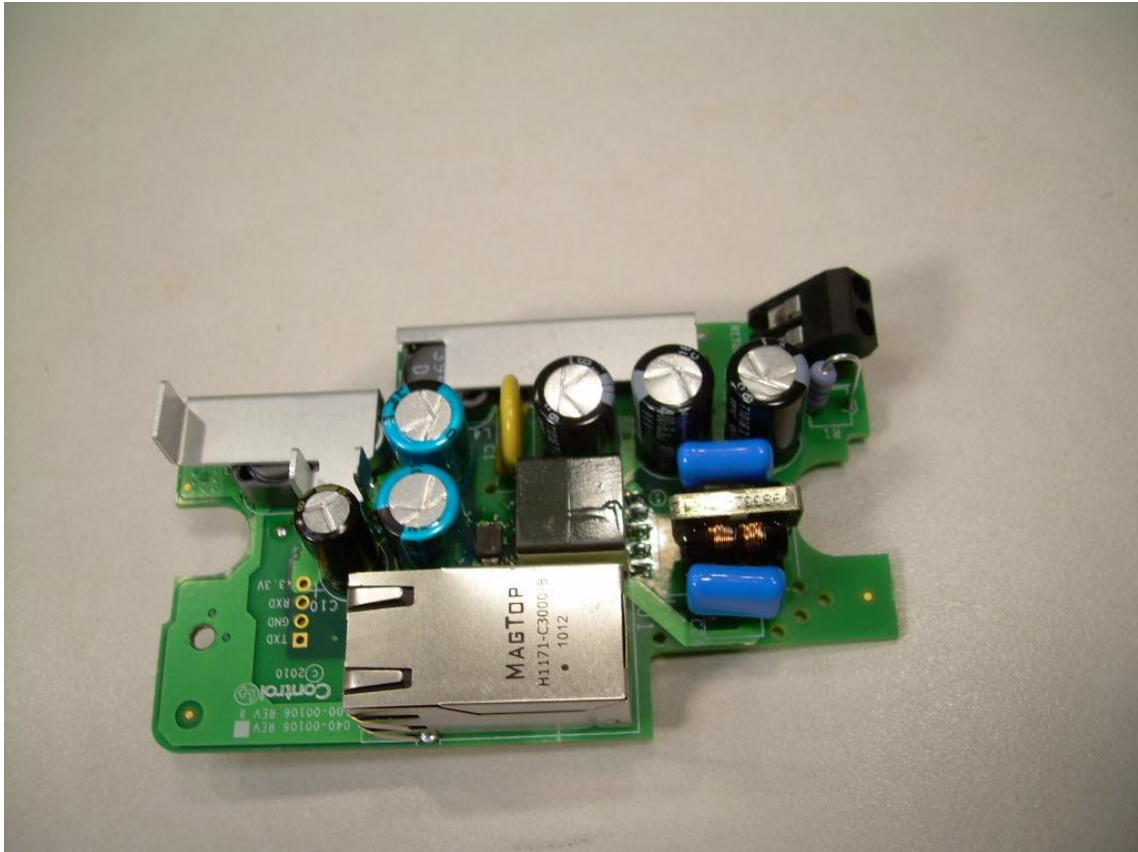
View of the Component Side of the Power Supply/Interface PCB with Heatsink in Place
