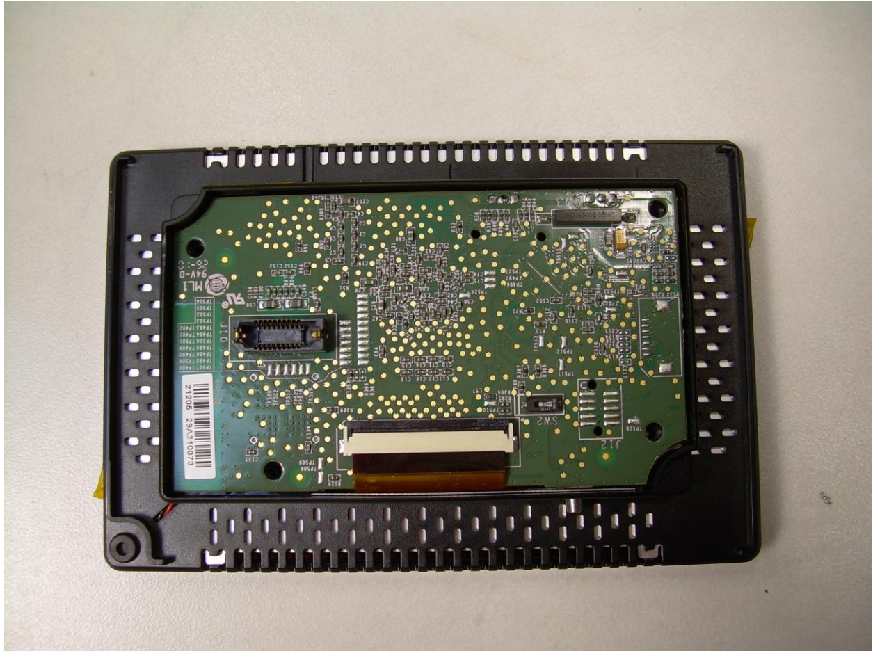
View of the Interface Side of the Display PCB
