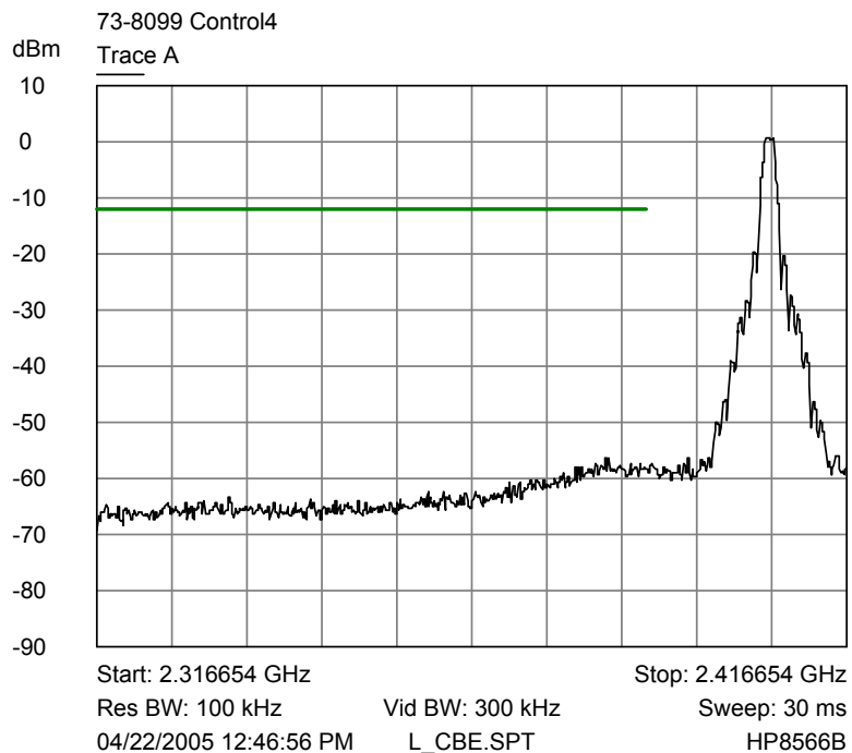
Trace A Lower Channel Conducted Band Edge Plot
