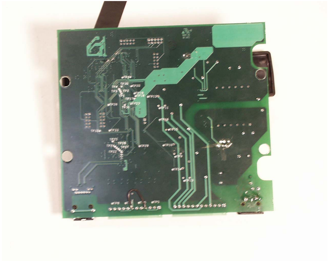
Photograph 8 - View of the Trace Side of the PCB
