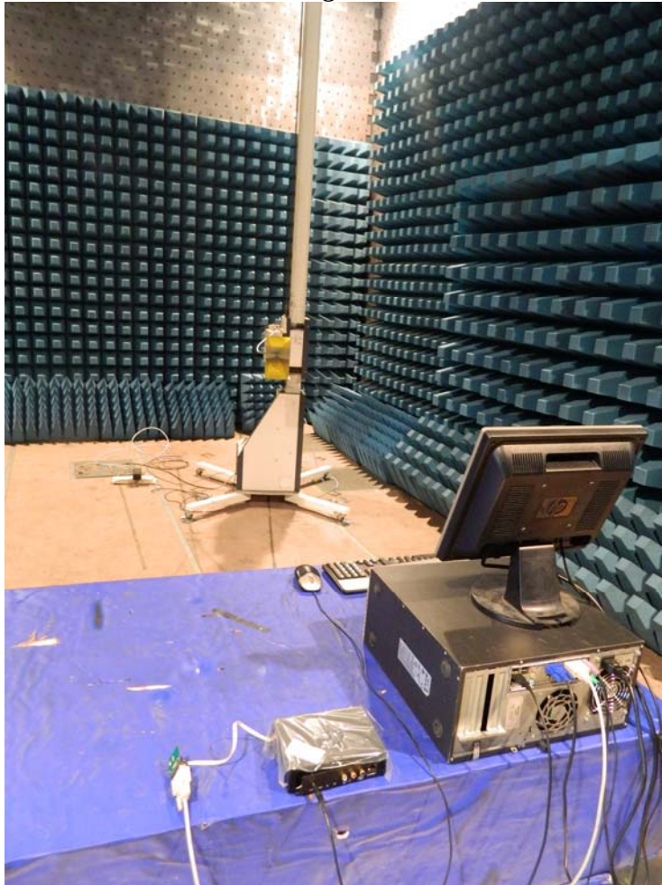
Wi-Fi test, higher than 1GHz
