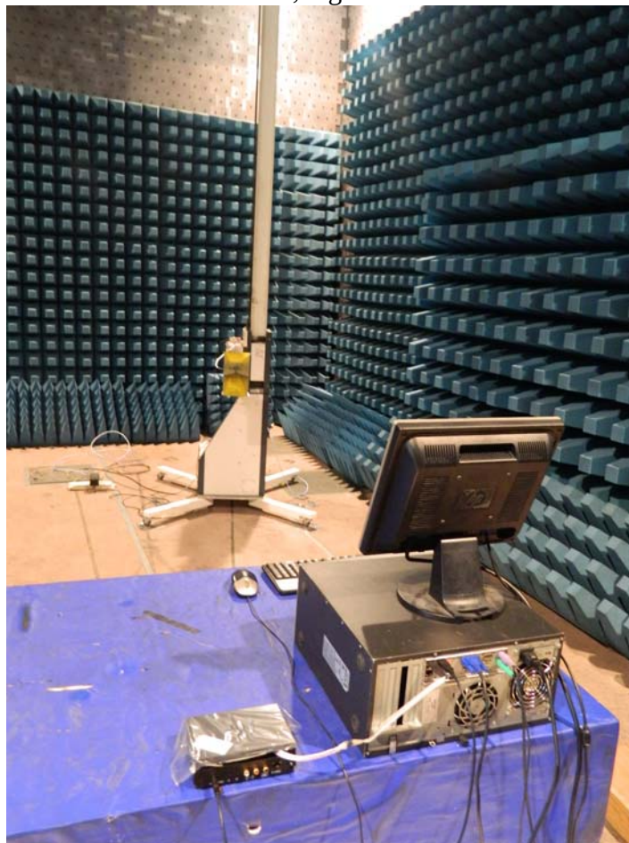
Bluetooth test, higher than 1GHz
