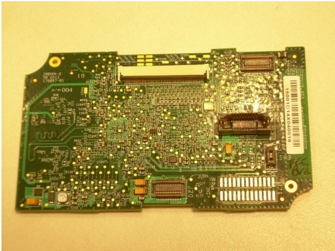
Photograph 19 – View of the Back Side of the Display PCB
