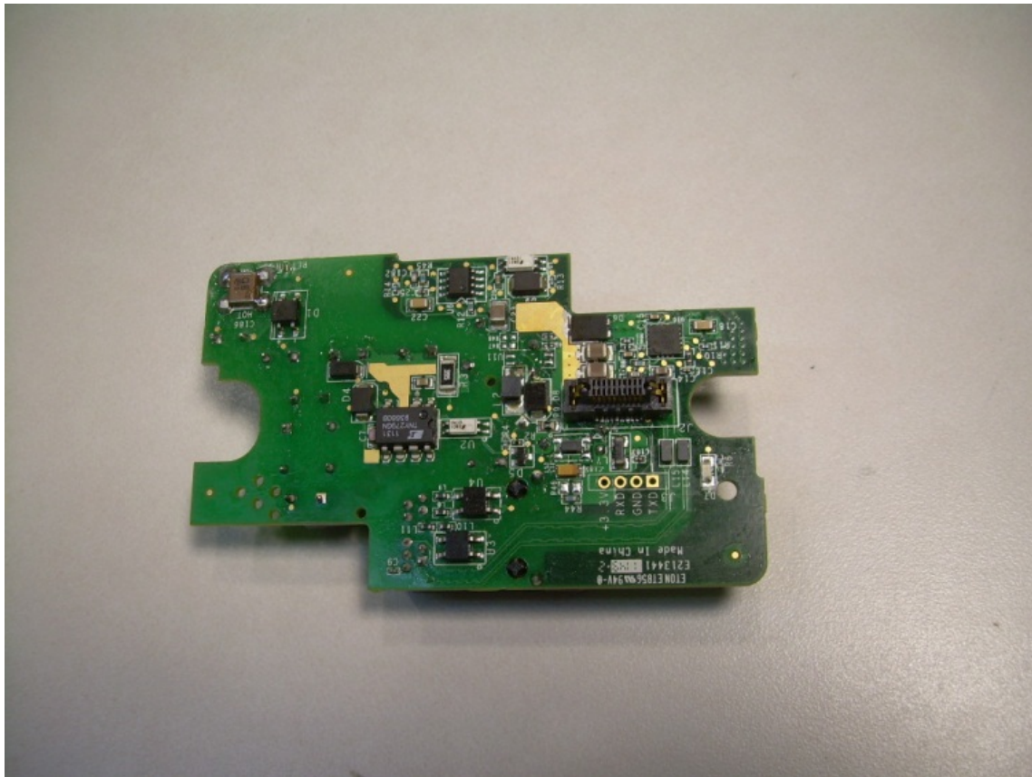
Photograph 15 – View of Component Side of Back Box PCB with Heatsink Removed
