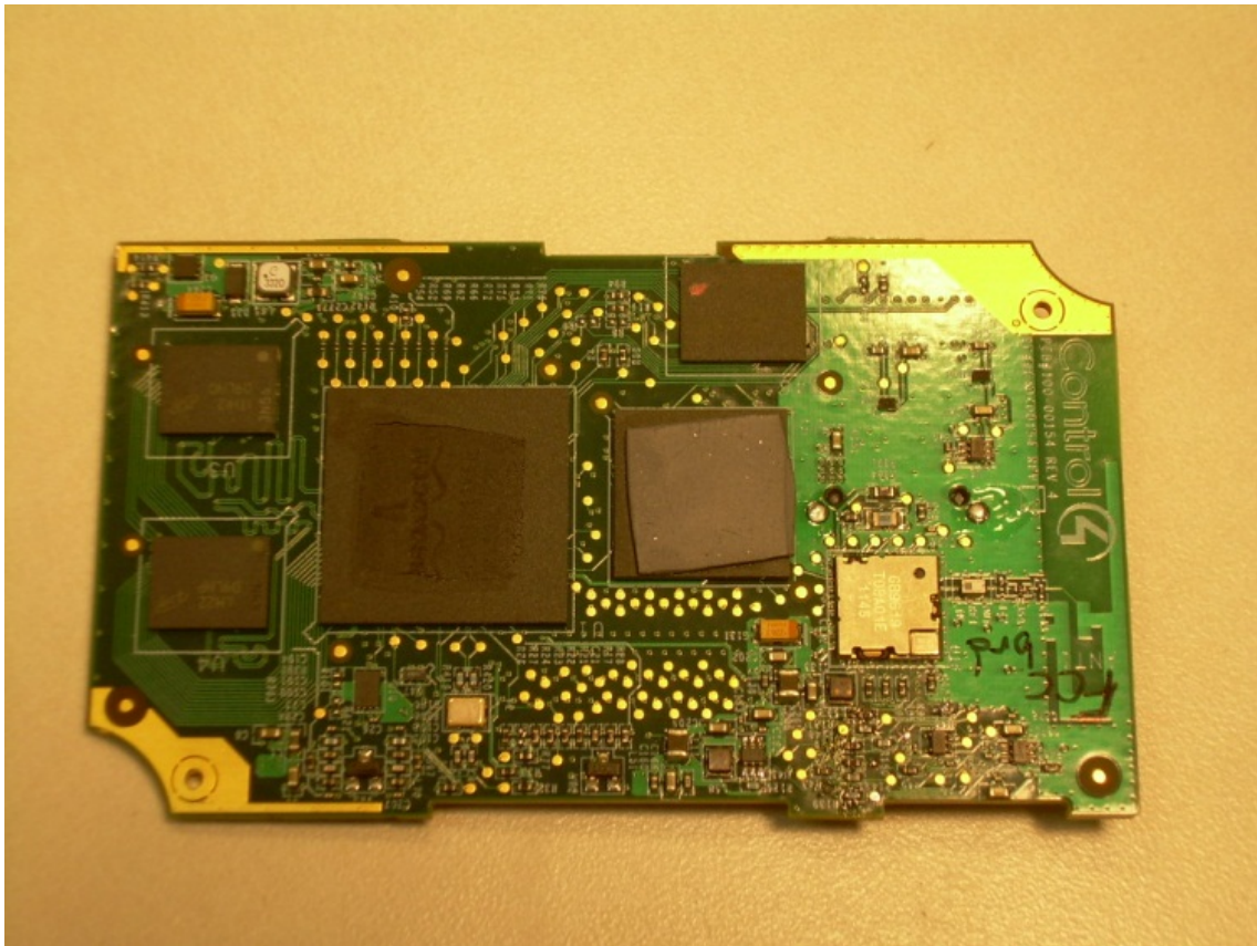
Photograph 20 – View of the Front Side of the Display PCB
