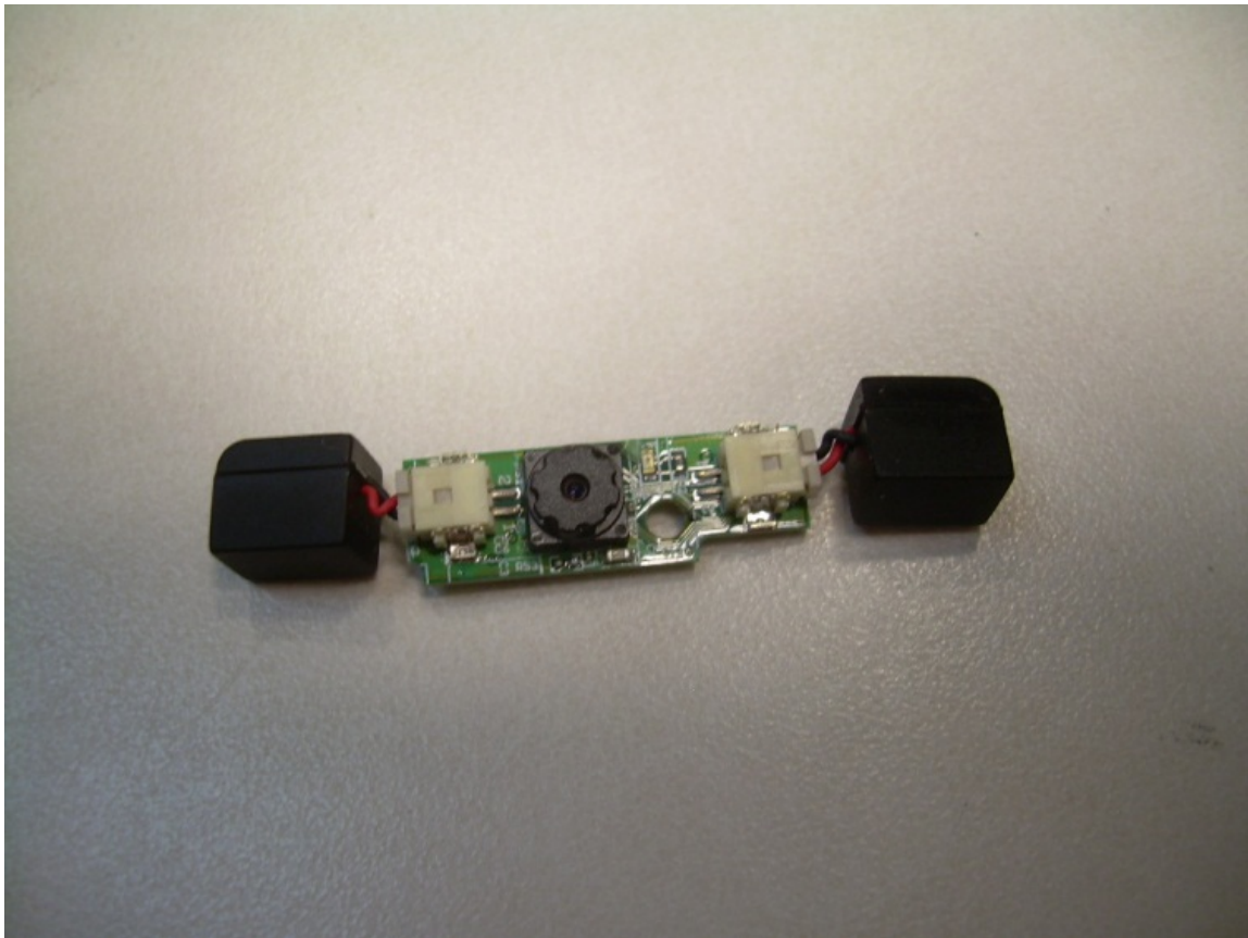
Photograph 22 – View of the Front Side of the Camera/Microphone PCB
