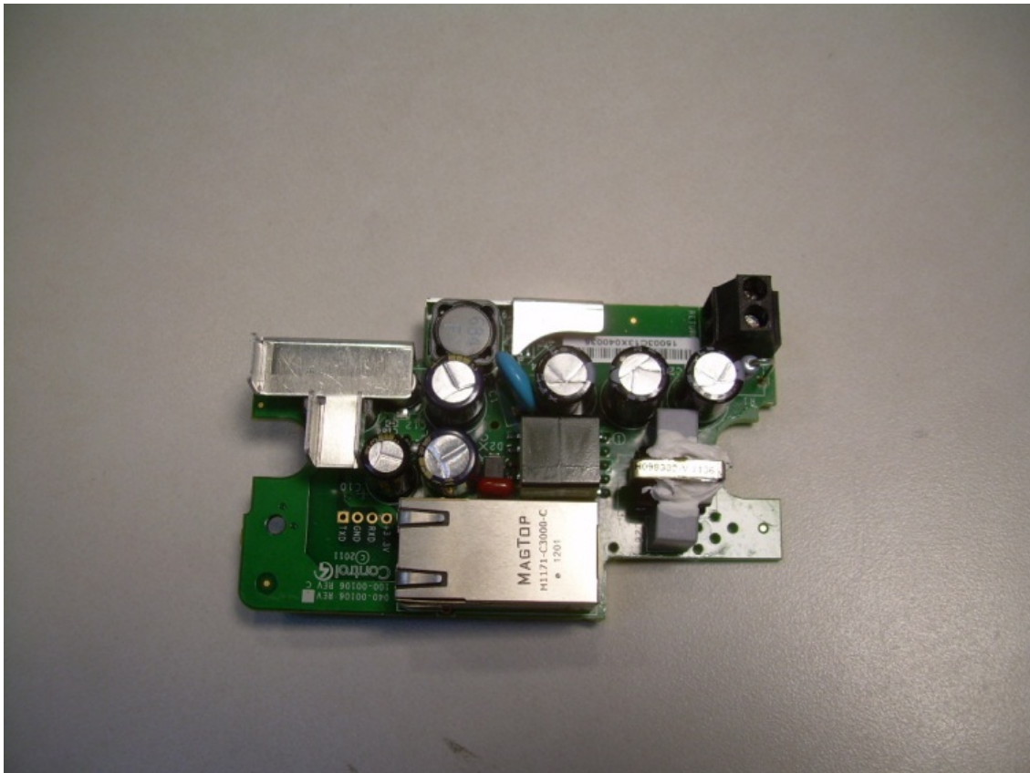
Photograph 13 – View of Component Side of Back Box PCB
