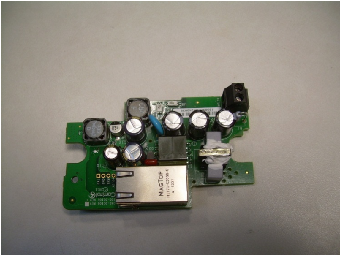
Photograph 16 – View of Trace Side of Back Box PCB with Heatsink Removed
