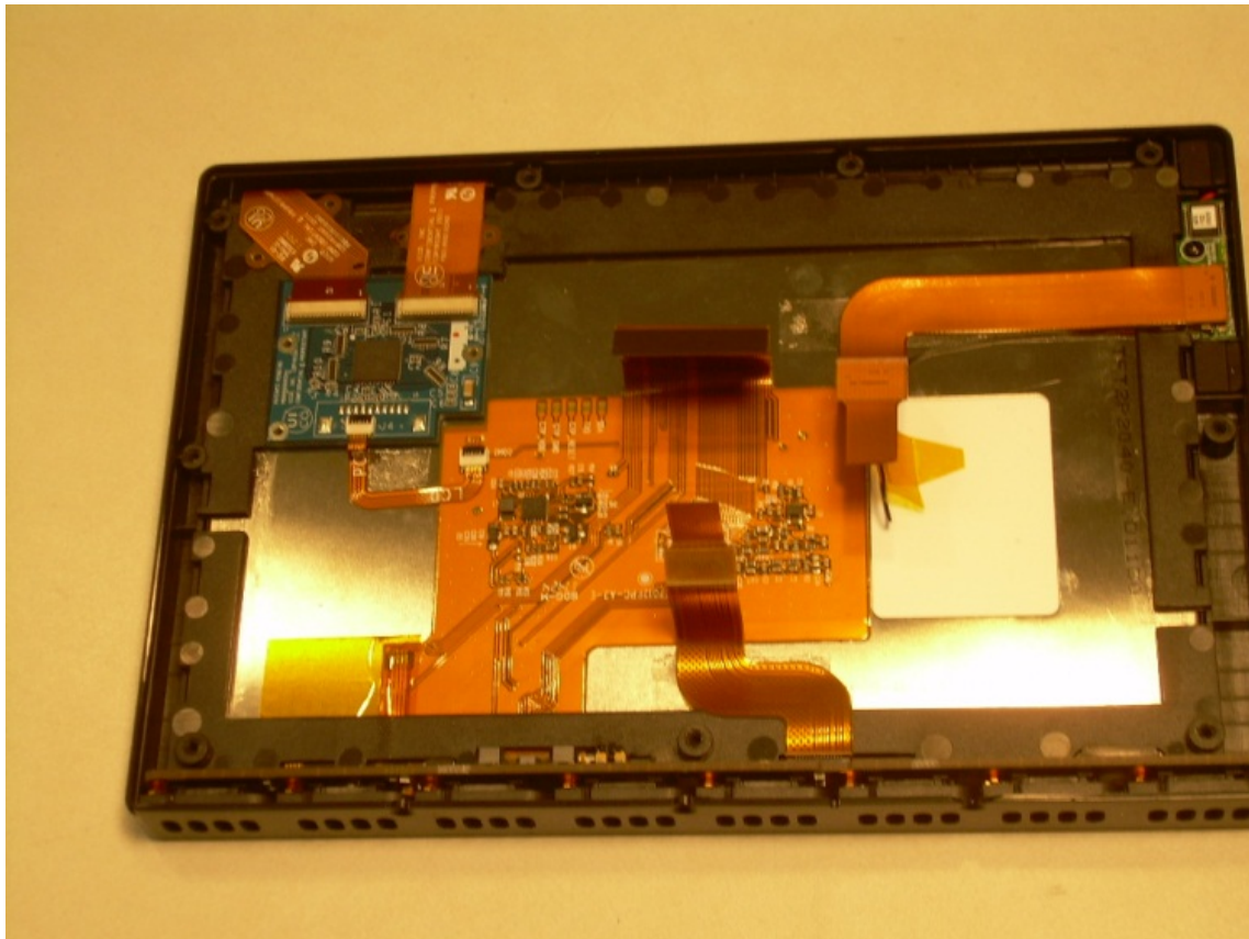
Photograph 18 – Back View of Display with Cover Removed
