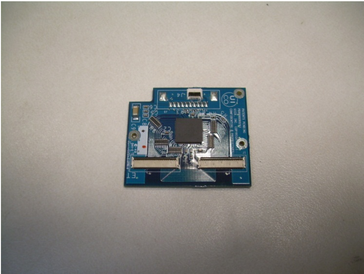
Photograph 23 – View of the Component Side of the Touch Interface PCB
