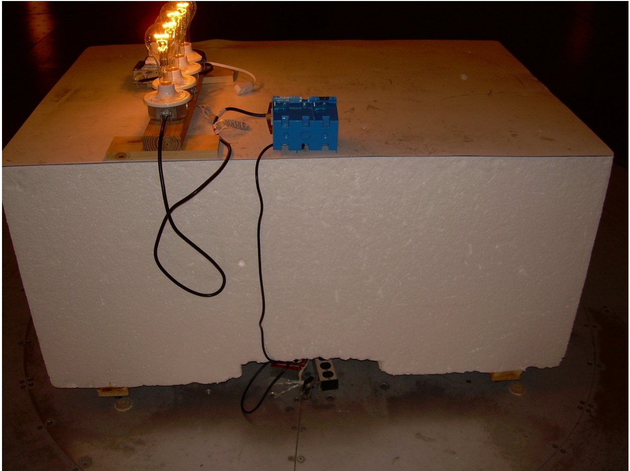
Back View Radiated Disturbance – C4-SW120277
