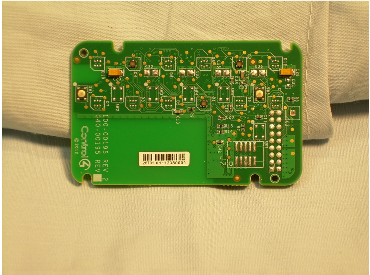
Front View of the RF PCB of the EUT
