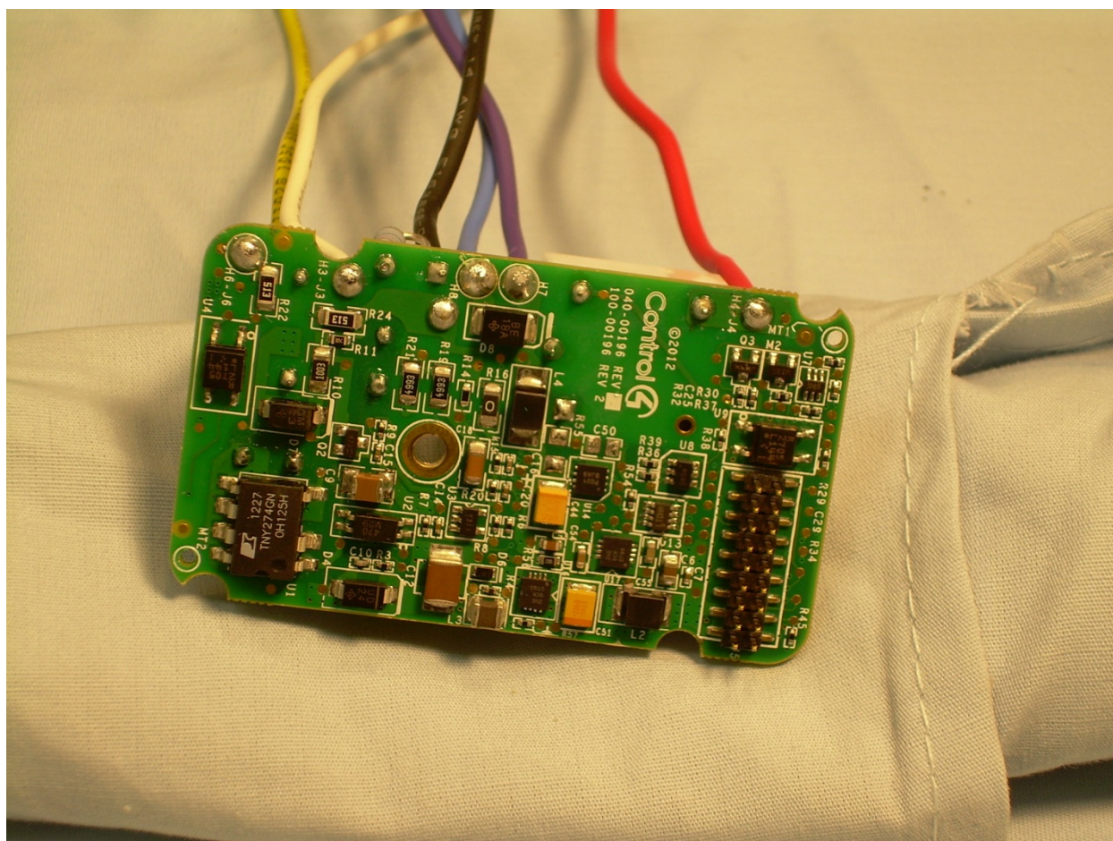
Front View of the C4-TV120277 Load PCB
