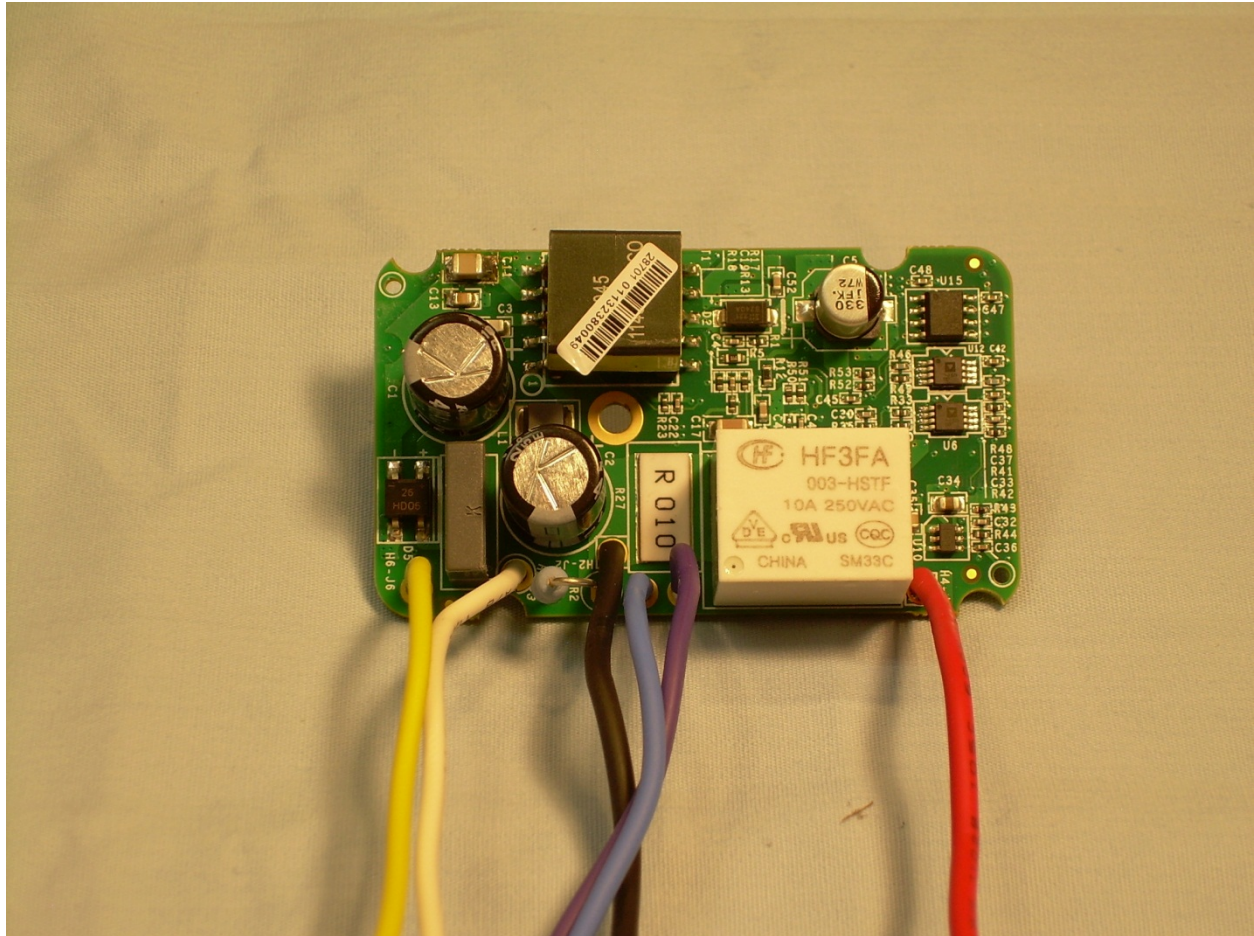
Back View of the C4-TV120277 Load PCB
