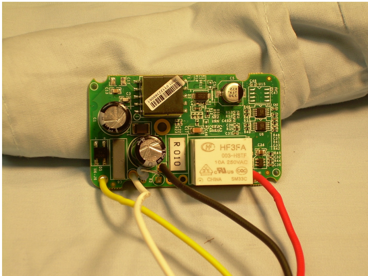
Back View of the C4-SW120277 Load PCB
