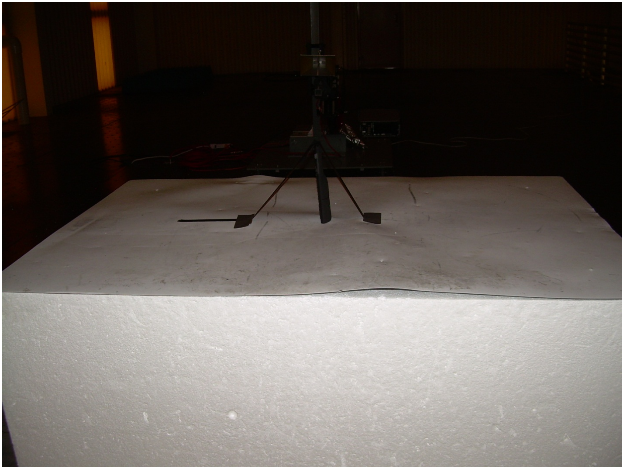
Photograph 5 – View Radiated Disturbance Configuration
