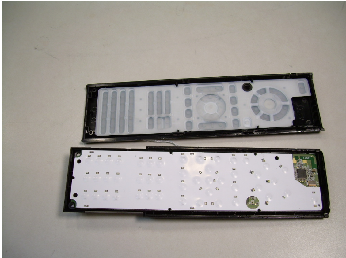
Photograph 6 – EUT Housing Separated
