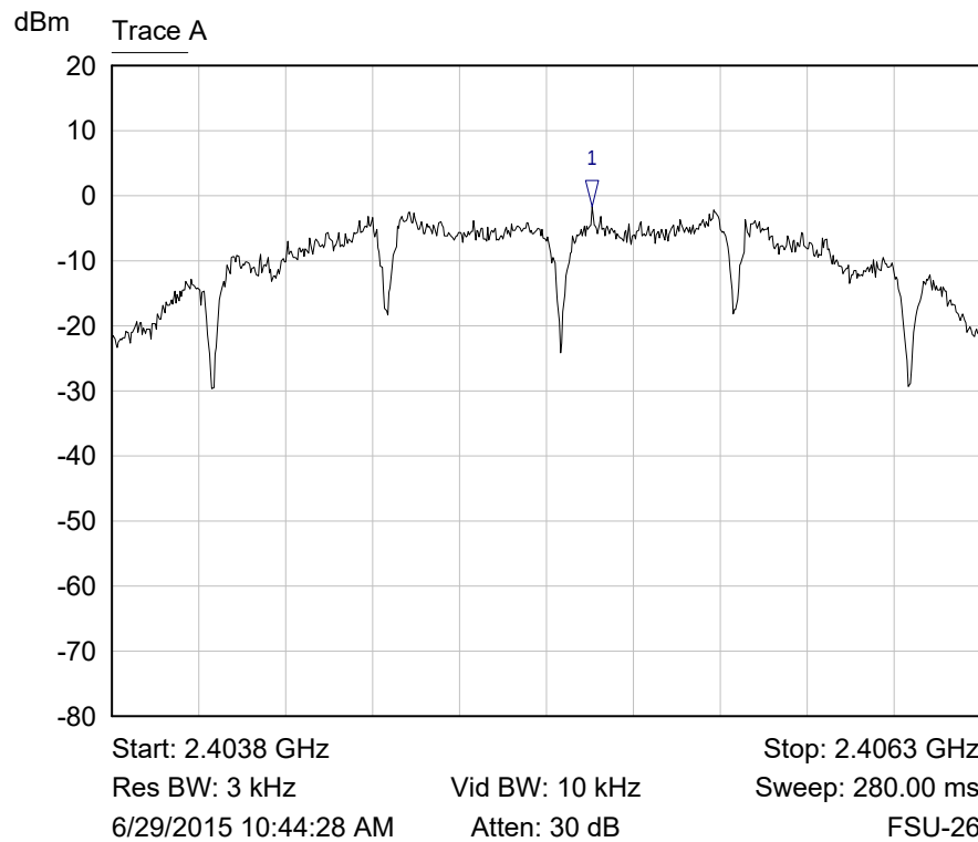
Lowest Channel 3 kHz PSD Plot
