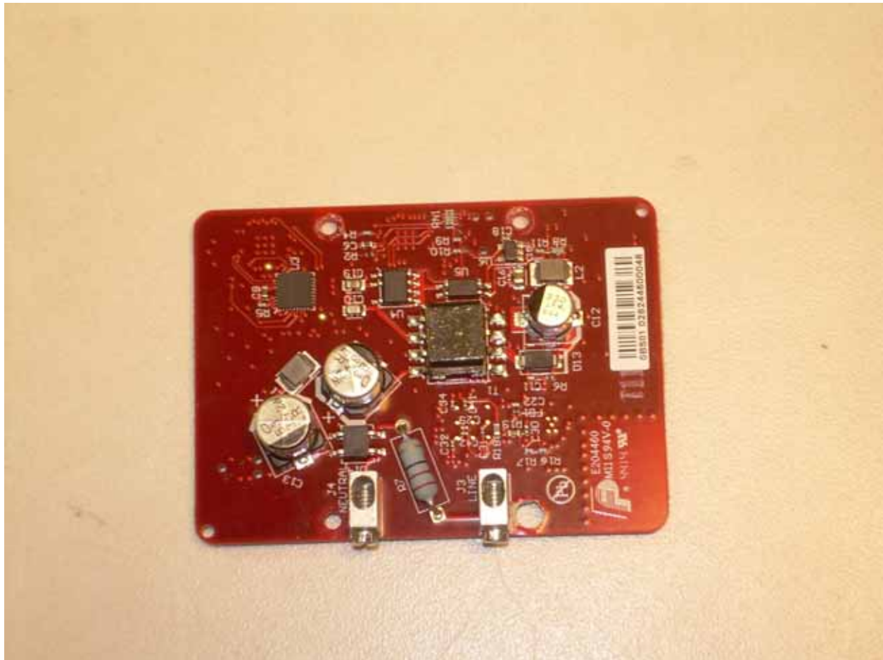
Photograph 8 – View of the Back of the PCB
