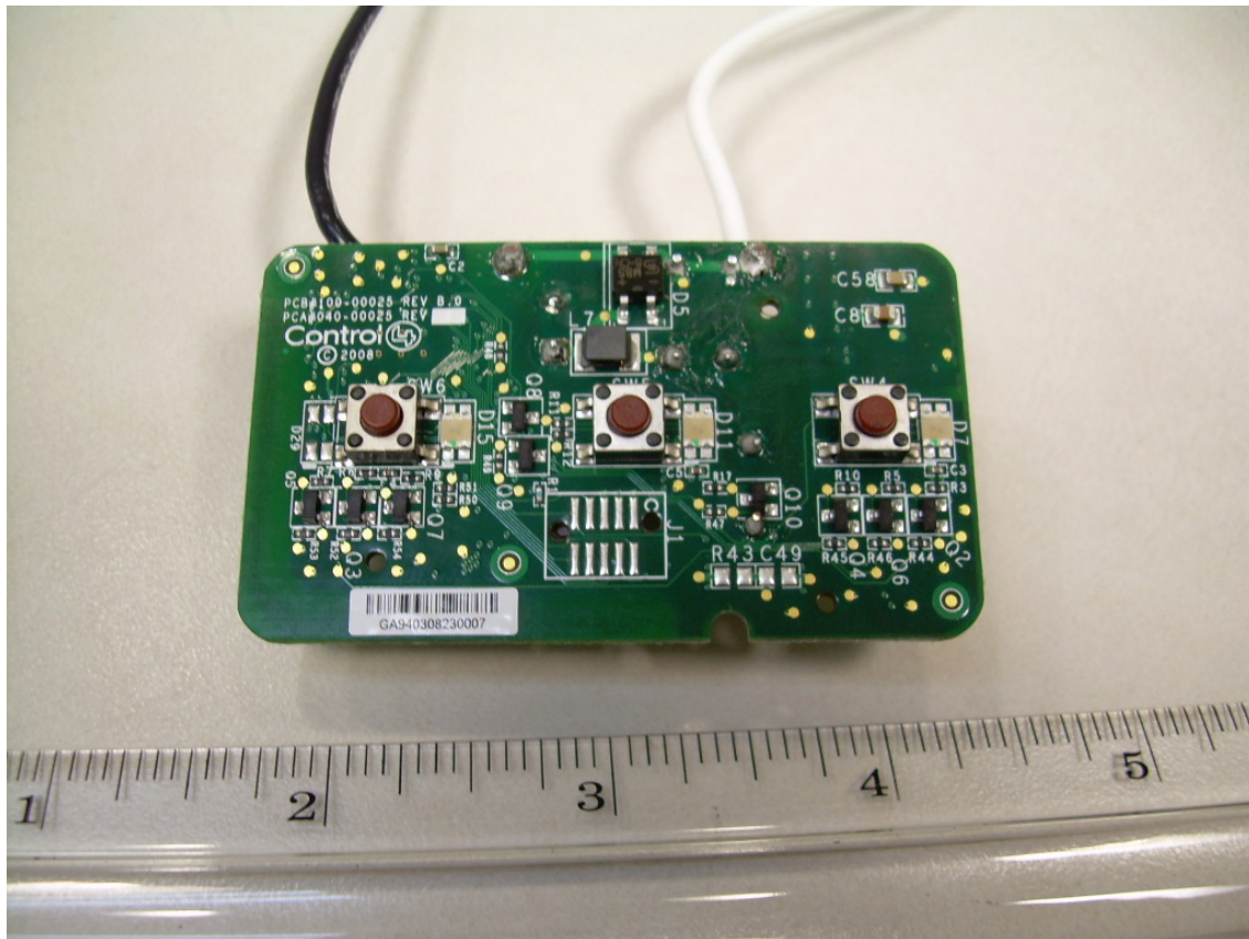
Front View of the C4-KP3-Z-x PCB
