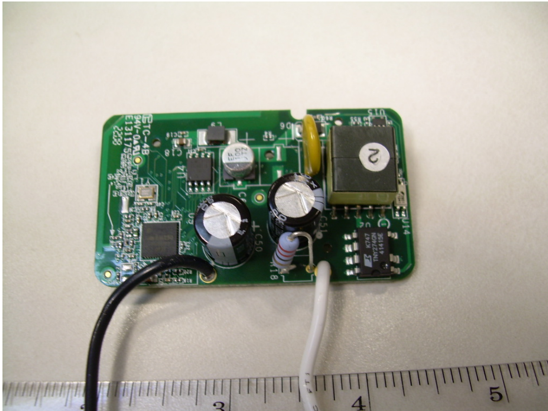
Back View of the C4-KP3-Z-x PCB
