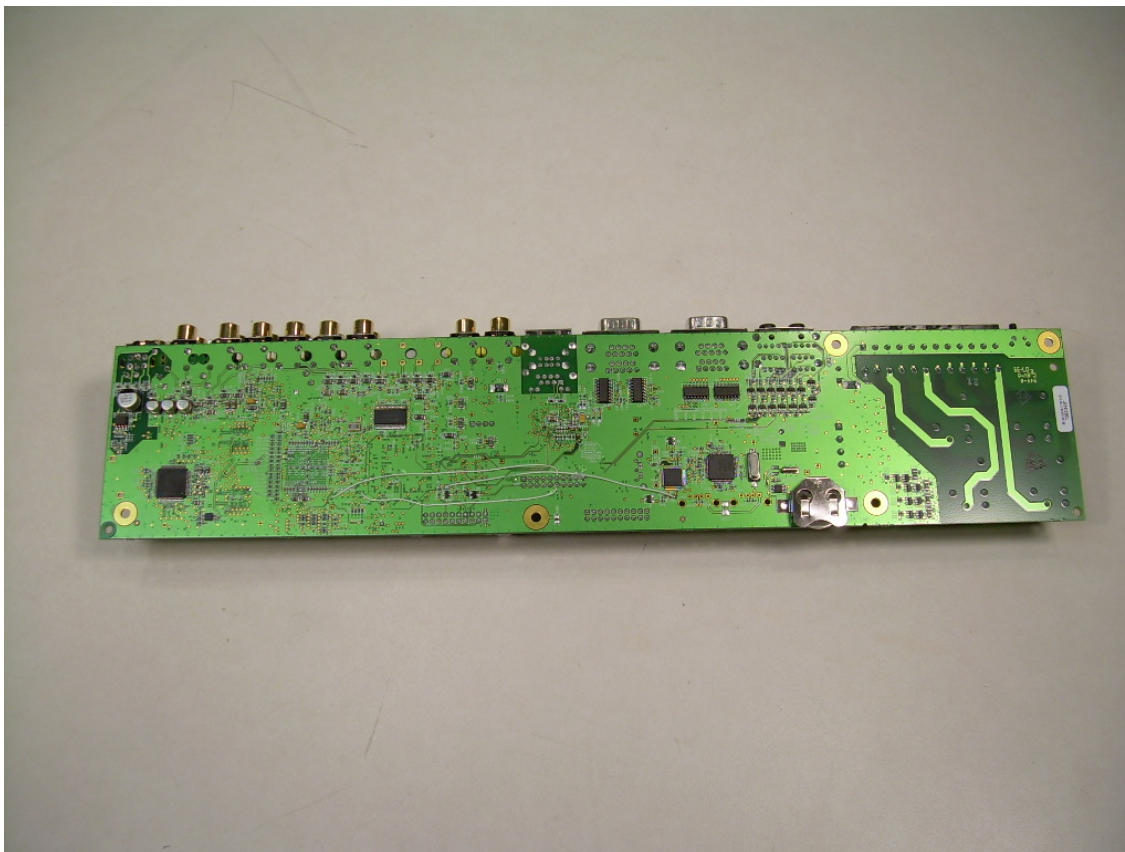
Photograph 9 - Trace Side of the Main PCB
