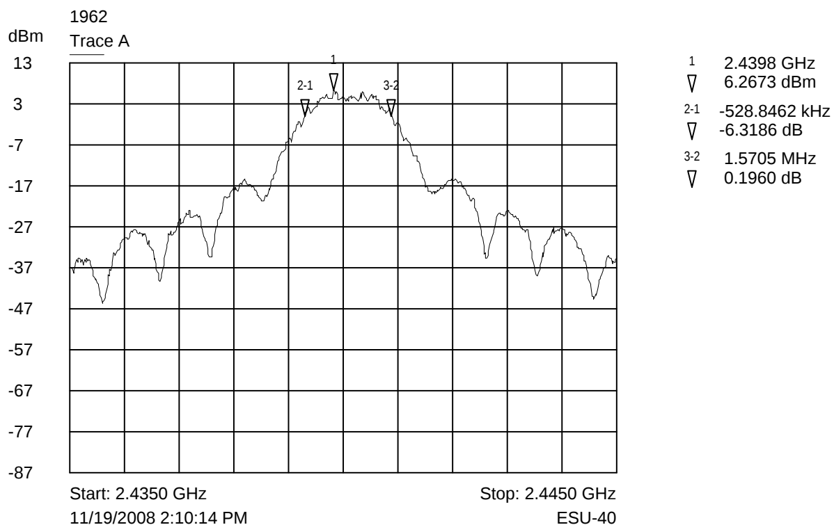
Trace A Middle channel bandwidth plot
