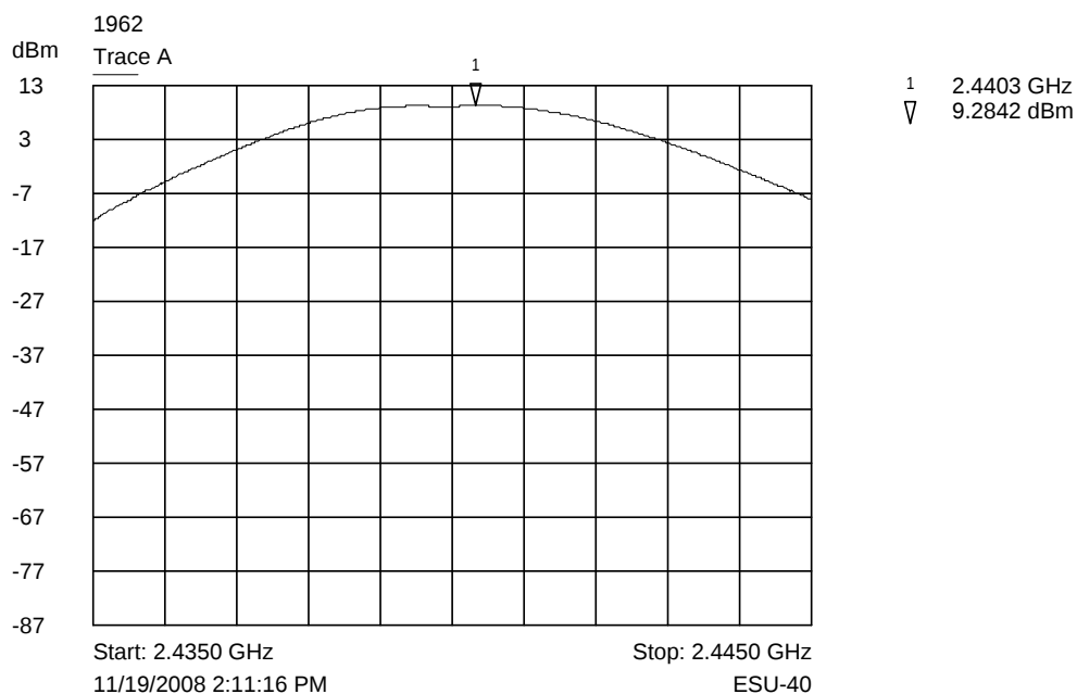
Trace A Middle channel output power plot
