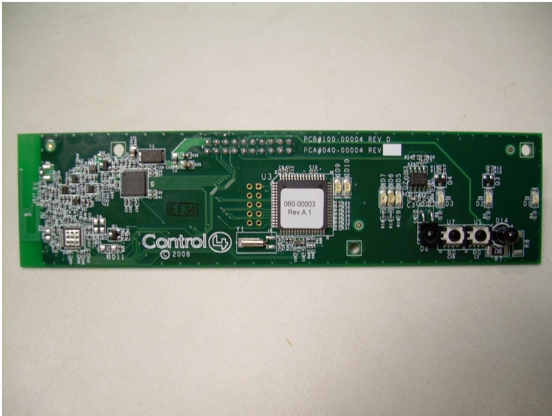
Photograph 10 - Component Side of the Front Panel/Transceiver PCB
