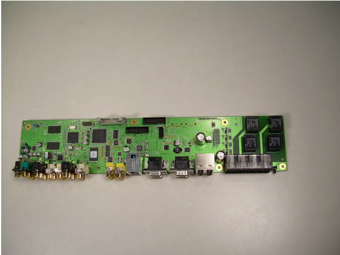
Photograph 8 - Component Side of the Main PCB
