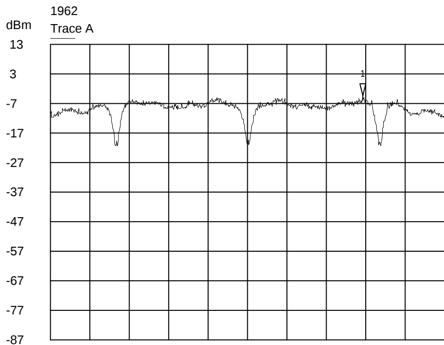
Trace A Lower channel 3 kHz power spectral density plot
