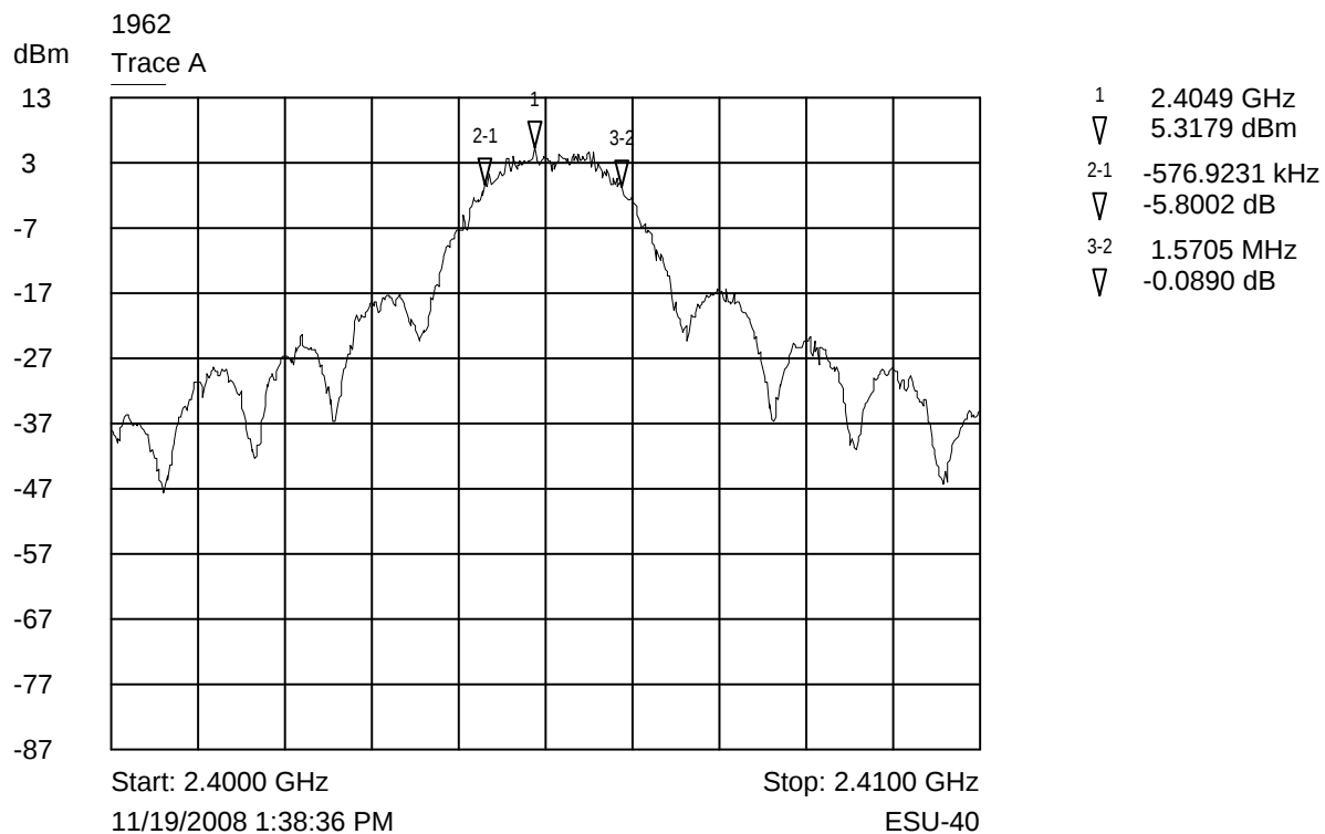
Trace A Lower channel bandwidth plot
