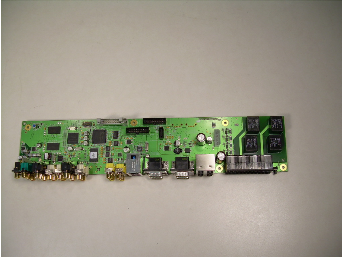
Component Side of the Main PCB
