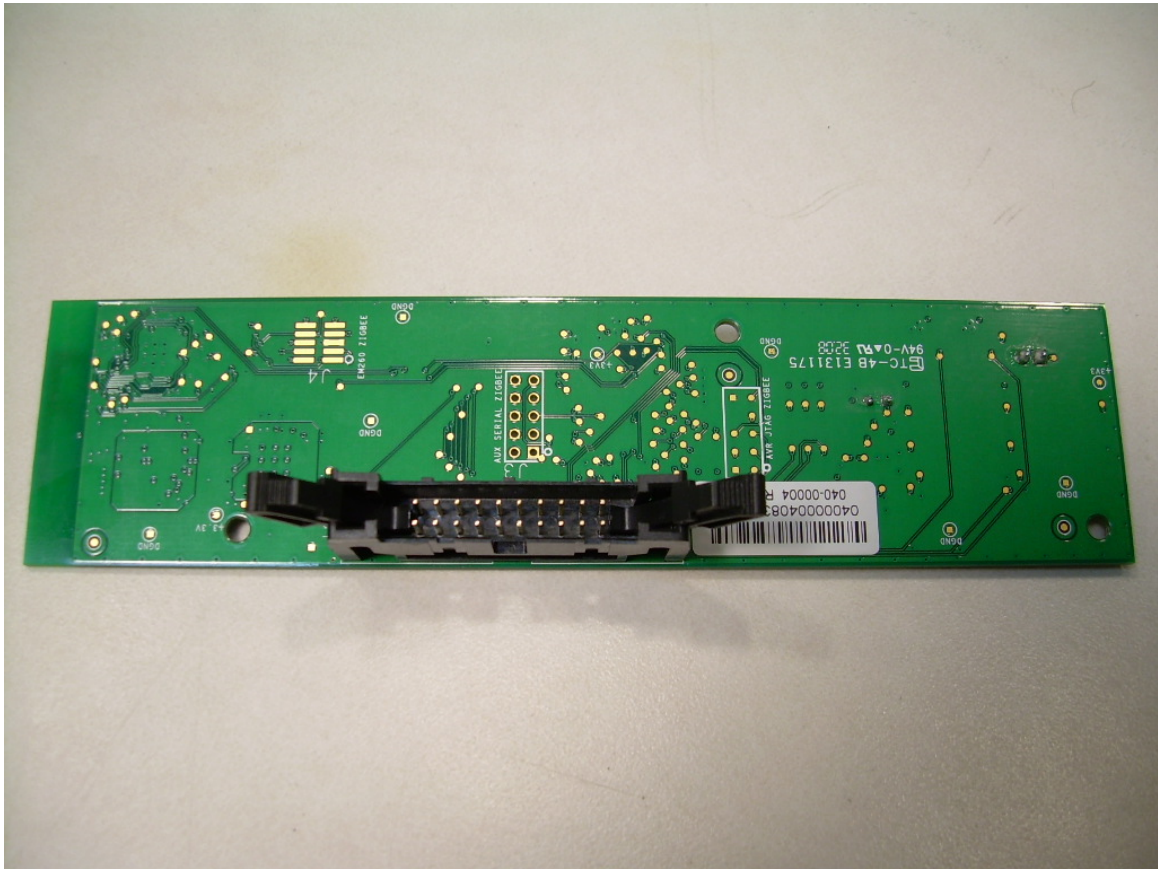
Trace Side of the Front Panel/Transceiver PCB
