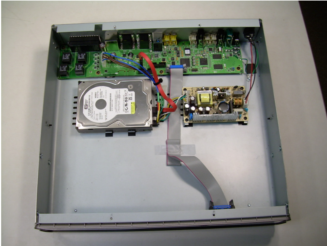
Photograph 7 - Internal View Front of the EUT
