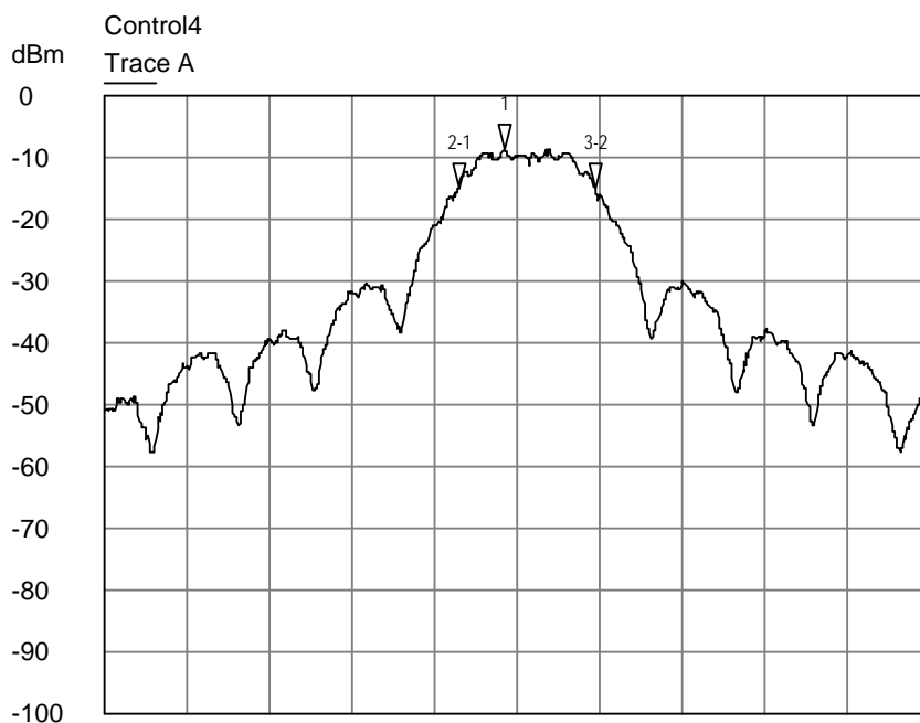
Trace A Lower channel - Bandwidth plot
