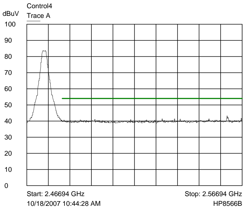
Trace A Upper channel band edge plot - corrected - radiated
