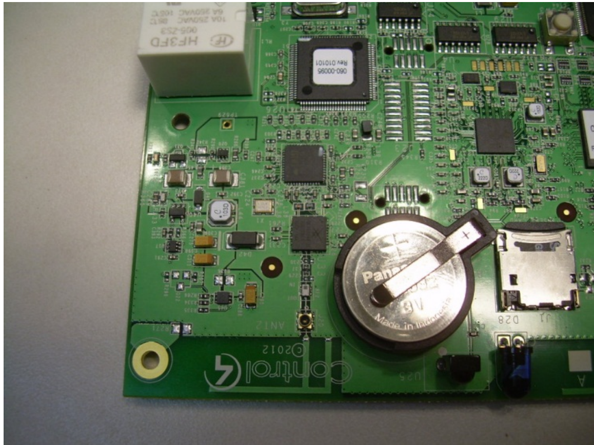
View of the 802.15.4 Radio Circuitry
