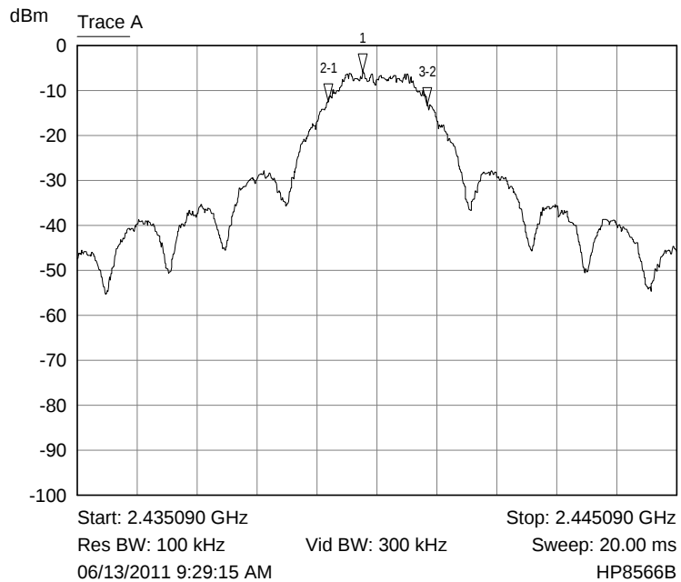
Trace A Band width plot
