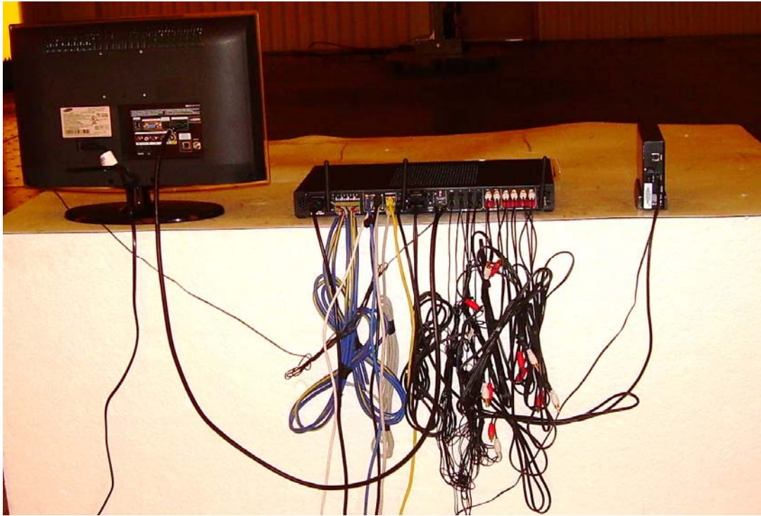
Back View of the Radiated Emission Setup
