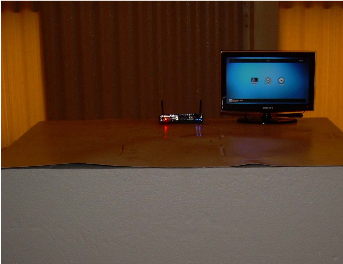
Front View of the Radiated Emission Setup
