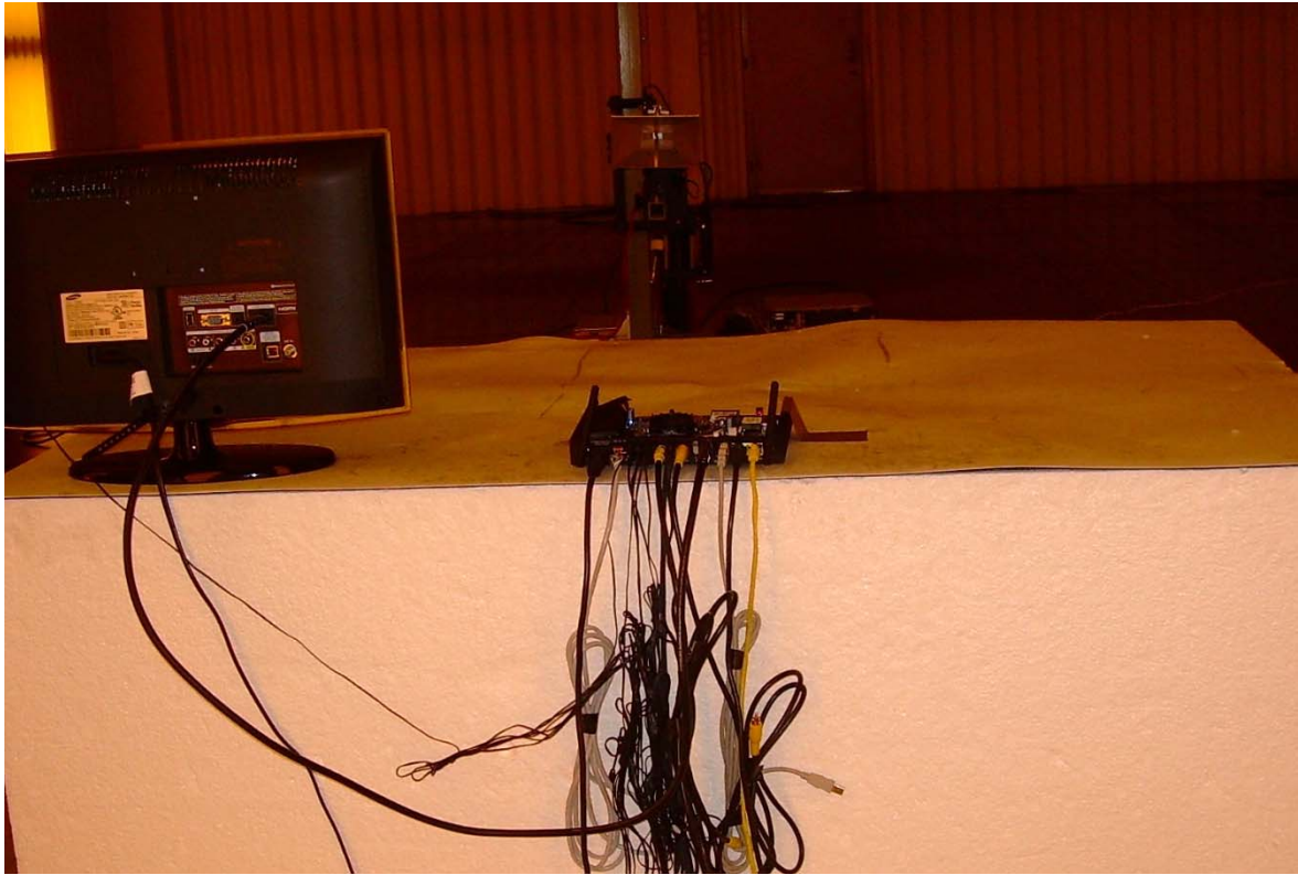
Back View of the Radiated Emission Setup
