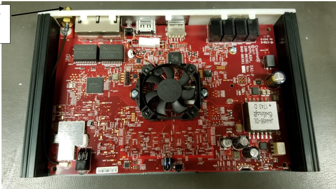
Photograph 11 – Top View of the PCB
