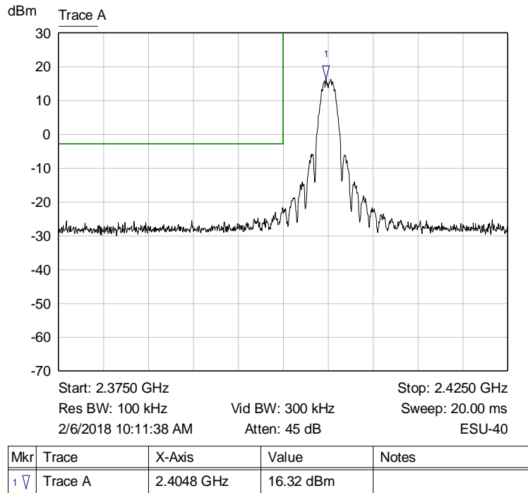
Graph 9: Lower Band Edge Plot (2405 MHz)
