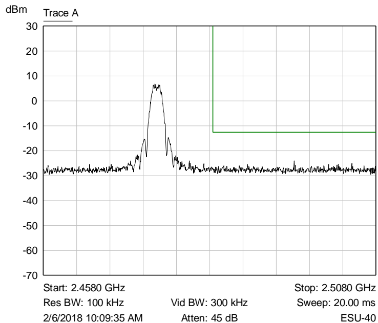
Graph 11: Upper Band Edge Plot (2475 MHz)
