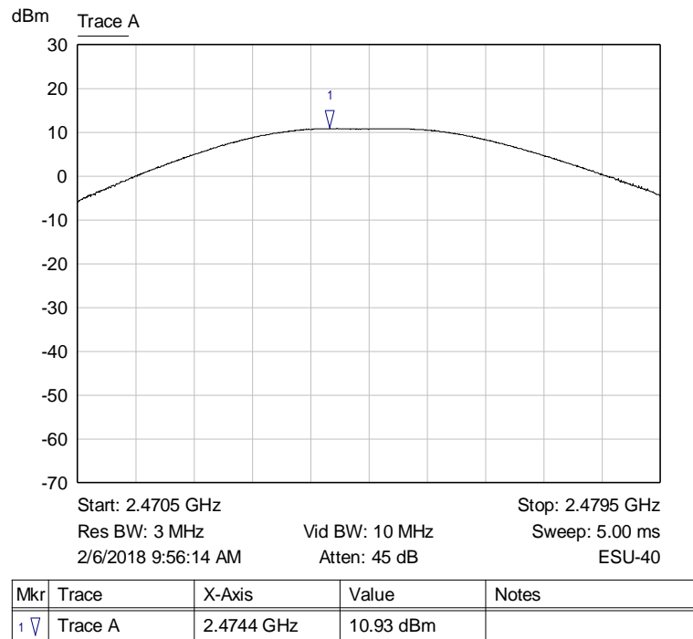
Graph 8: Highest Channel Output Power Plot (2475 MHz)
