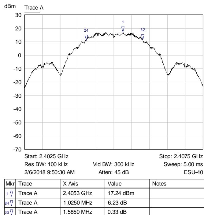
Graph 1: Lowest Channel Bandwidth (2405 MHz)
