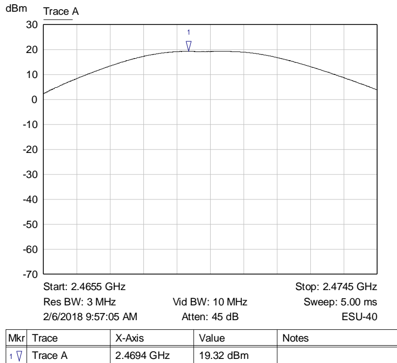
Graph 7: Channel 24 Output Power (2470 MHz)
