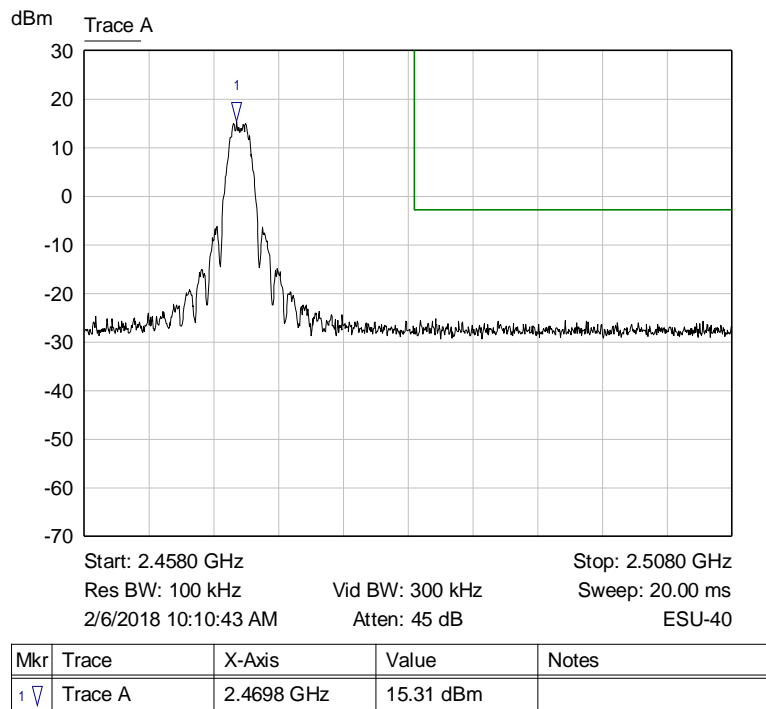
Graph 10: Upper Band Edge Plot (2470 MHz)
