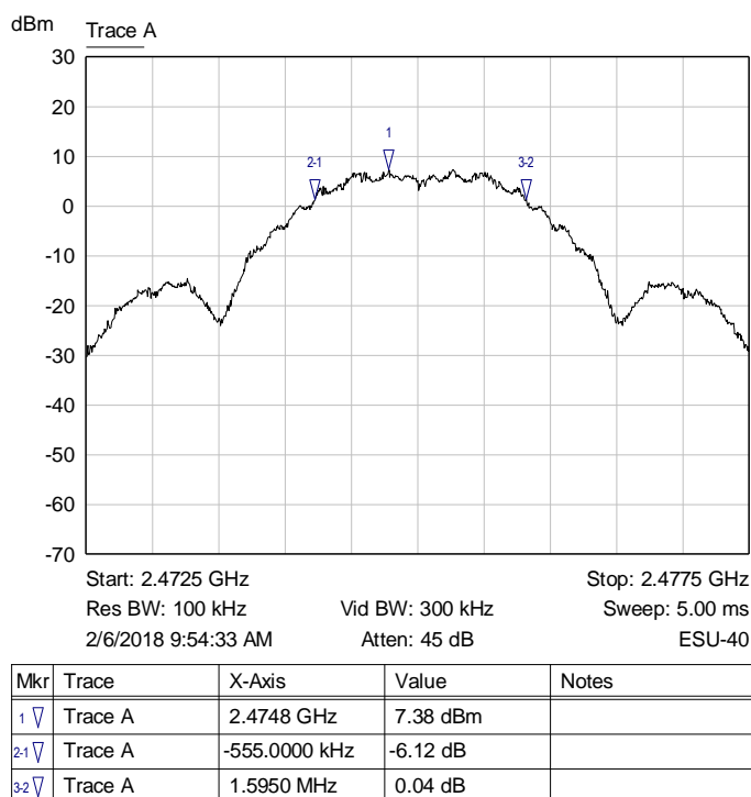
Graph 4: Highest Channel Bandwidth (2475 MHz)
