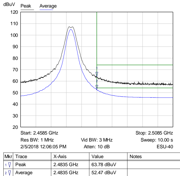
Graph 14: Radiated Upper Band Edge Plot (2475 MHz)
