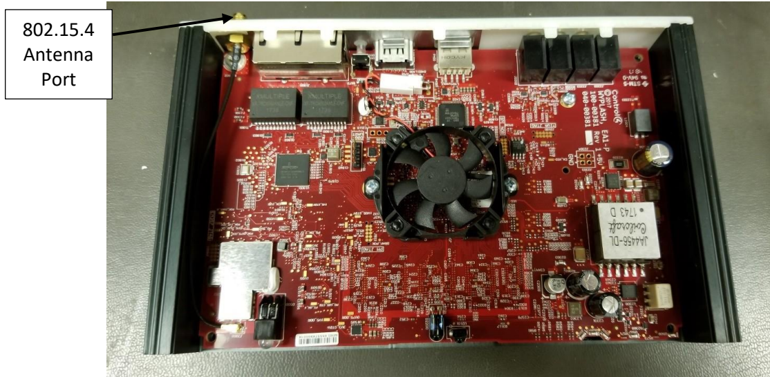
Photograph 1 – Top View of the PCB
