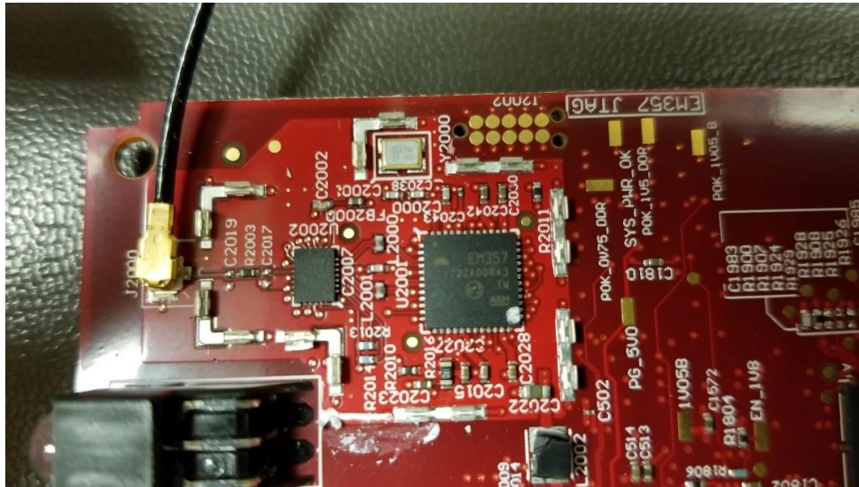
Photograph 4 – View of the Circuitry Under the RF Shield
