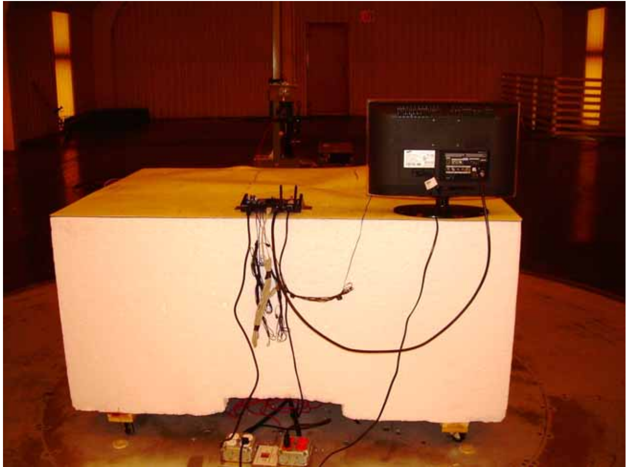
Back View Radiated Disturbance Configuration – Oxford TEC Antenna
